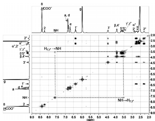
Figure 3. H,H-COSY spectrum of 5 (300 MHz, [\text{D}_6]\text{DMSO} ).
