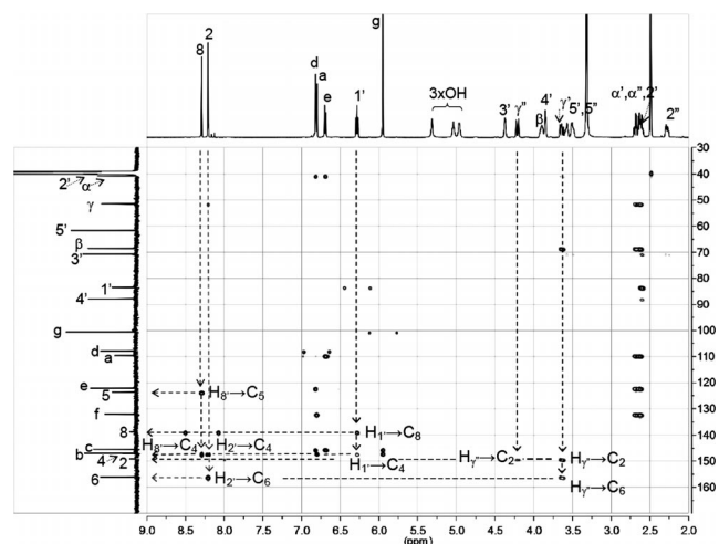
Figure 2. HMBC spectrum of 4 (500 MHz, [\text{D}_6] DMSO).
