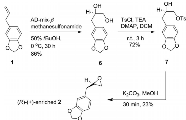
Scheme 1. Enantioselective synthesis of ( R )-(+)-enriched 2 .
