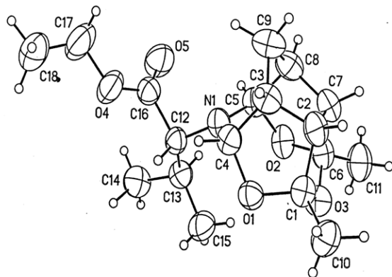
Figure 1. ORTEP diagram of 34a .
