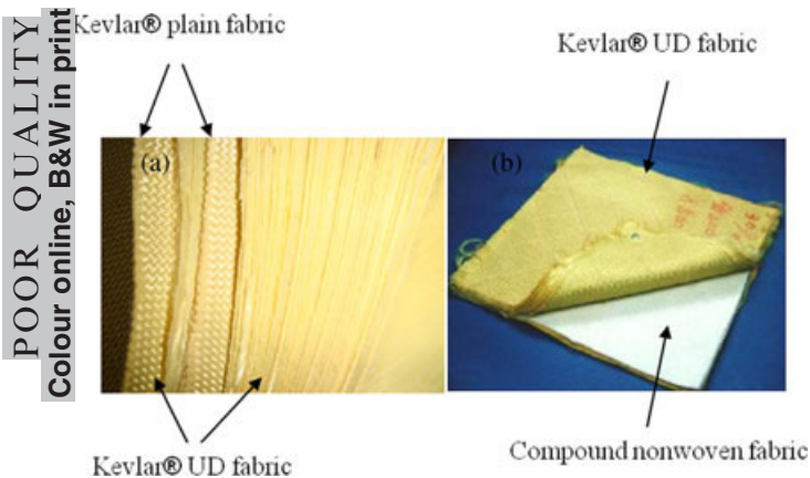
FIG. 3—Pictures of (a) commercial exemplar vest and (b) new armor target.
