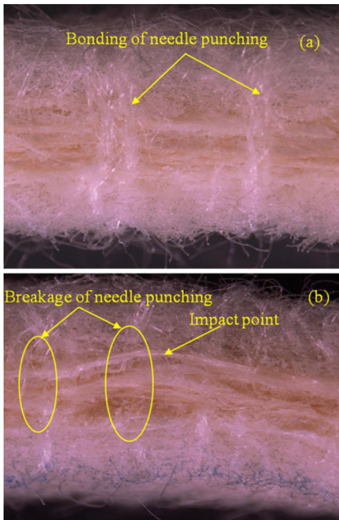
FIG. 8—Cross-section of compound nonwoven fabric (a) before and (b) after impact.
