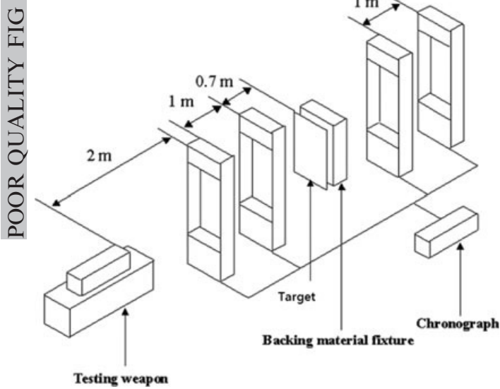
FIG. 6—The setup for the shooting test.
