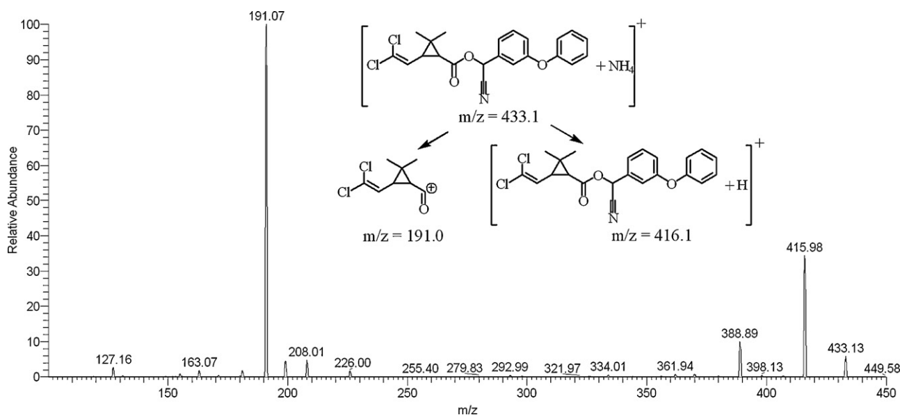
Fig. 3. Product ion spectrum of cypermethrin at 15 eV demonstrated that the fragment at m/z 416 as the [M+H]^+ ion of cypermethrin and the fragment at m/z 191 showing as the dichlorovinylidimethylcyclopropane acylium ion from cleavage of the carbon–oxygen bond of the ester group.
