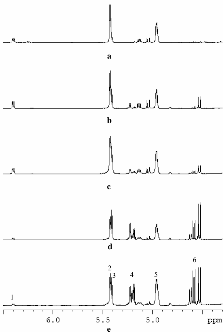
Figure 4. ^1\text{H-NMR} spectra of processed Rehmannia glutinosa roots in the range of \delta 4.3 – \delta 6.5. a: fresh root; b: dried root; c: one cycle processing (rinsed with Chinese rice wine, steamed and baked); d: five cycles processing; e: nine cycles processing. 1: H-3 of catalpol; 2: H-1 of raffinose and stachynose; 3: H-1 of sucrose; 4: H-1 of \alpha -glucose and \alpha -galactose; 5: H-1 of internal \alpha -glucose and \alpha -galactose moiety of raffinose and stachynose; 6: H-1 of \beta -glucose and \beta -galactose.
