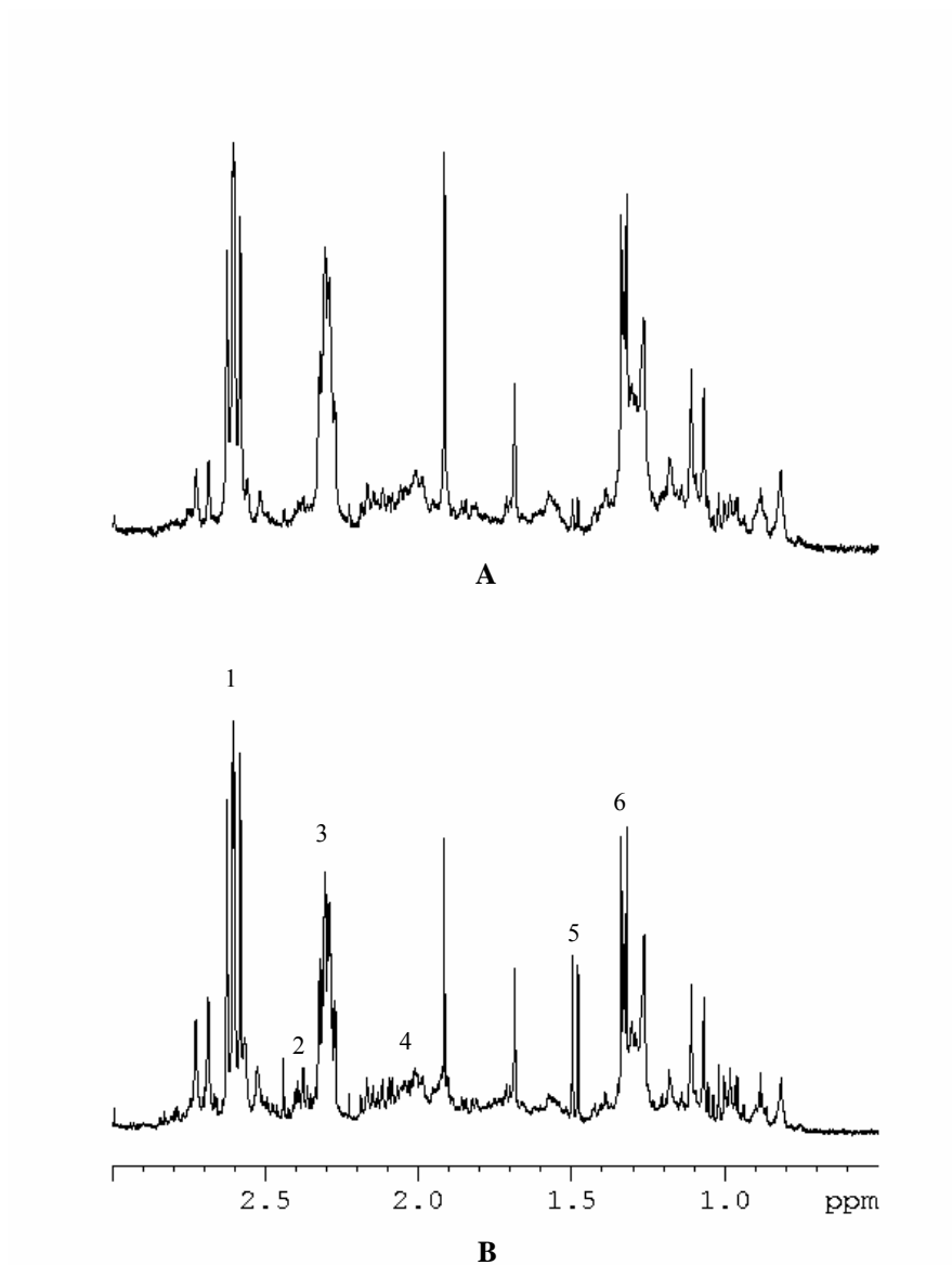
Figure 5. 1 H-NMR spectra of processed Rehmannia glutinosa roots in the range of \delta 0.5 – \delta 3.0. A: processed root grown at 22°C; B: processed root grown at 25°C. 1: H-9 of catalpol; 2: H-3 of proline; 3: H-5 of catalpol; 4: H-3' of proline; 5: H-3 of alanine; 6: H-5 of threonine.
