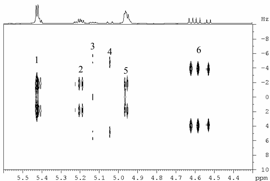
Figure 3. Two dimensional J -resolved NMR spectra of processed Rehmannia glutinosa roots in the range of \delta 4.3 – \delta 5.6. 1: H-1 of raffinose, stachynose and sucrose; 2: H-1 of \alpha -glucose and \alpha -galactose; 3: H-4 of catalpol; 4: H-1' of catalpol; 5: H-1 of internal \alpha -glucose and \alpha -galactose moiety of raffinose and stachynose; 6: H-1 of \beta -glucose and \beta -galactose.
