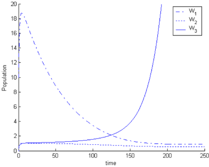
Fig. 8.3 Numerical simulation with \sigma_2 + \gamma_2 < \mu , \sigma_2 + \gamma_2 > \gamma_3 , and \hat{\beta} > C in (W_1, W_2, W_3) -space, as the population approaches E_{3\infty} .
