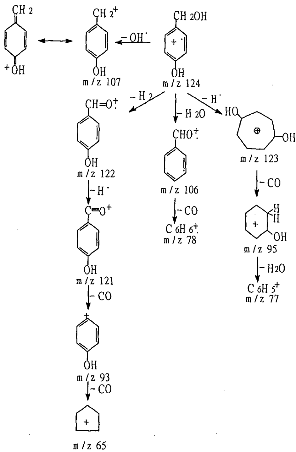
Scheme 2. The mass spectral fragmentation patterns of gastrodigenin
