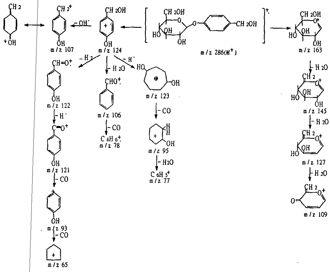
Scheme 1. The mass spectral fragmentation patterns of gastrodin
