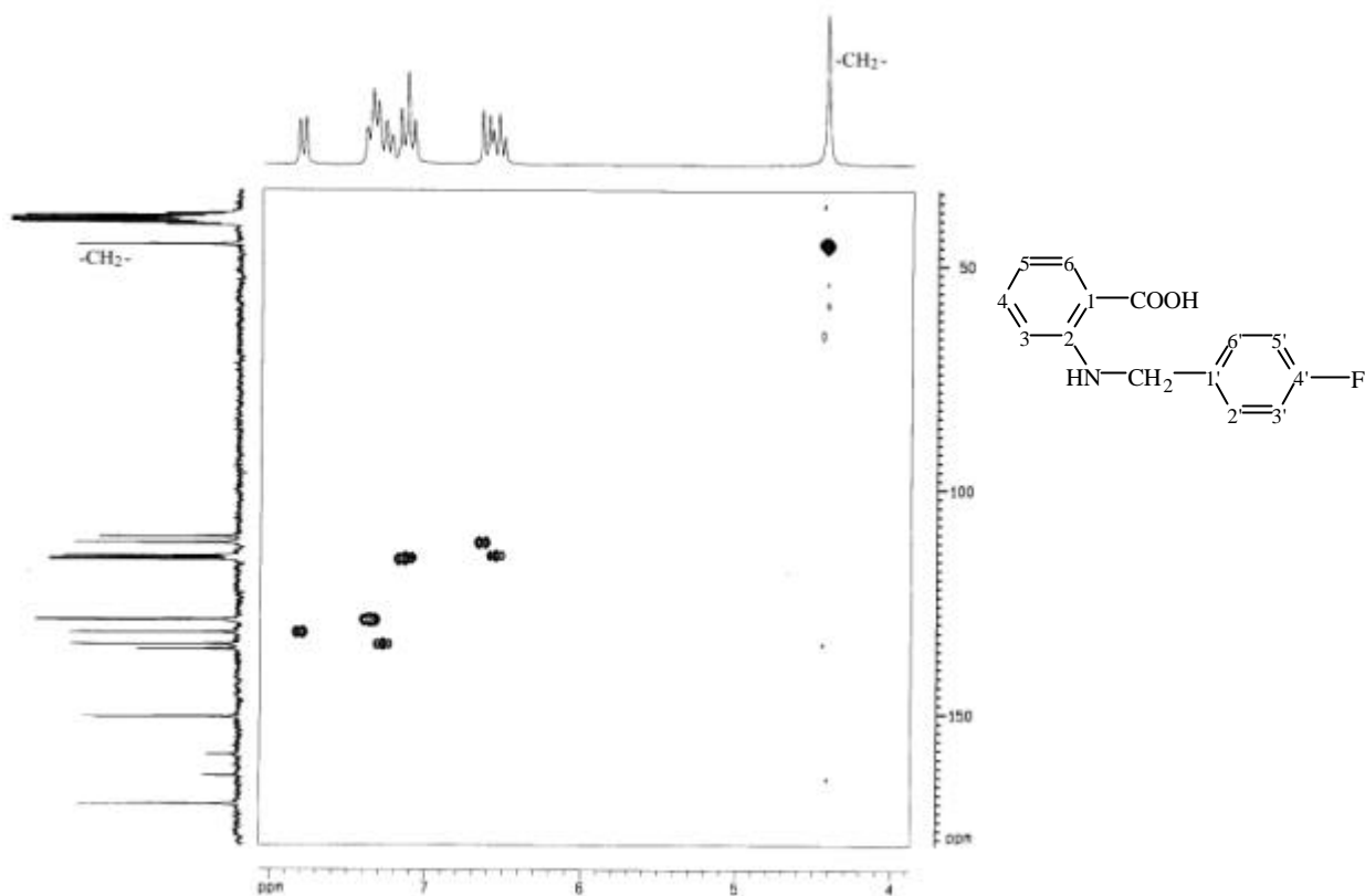
圖 71-6a HMQC (DMSO- d_6 ) spectrum of compound 71
