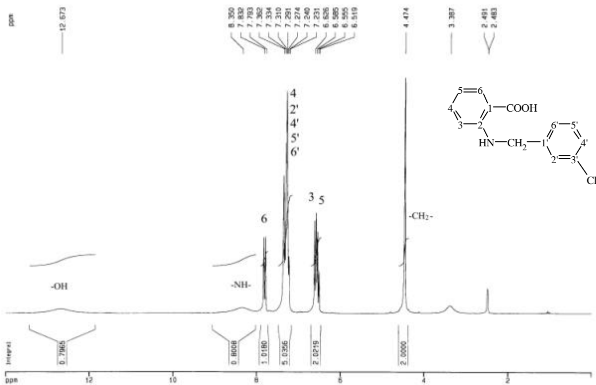
圖 67-3 ^1\text{H-NMR} (DMSO- d_6 , 200 MHz) spectrum of compound 67
