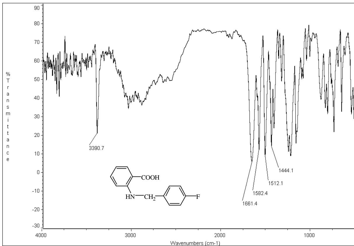
圖 71-2 IR (KBr) spectrum of compound 71
