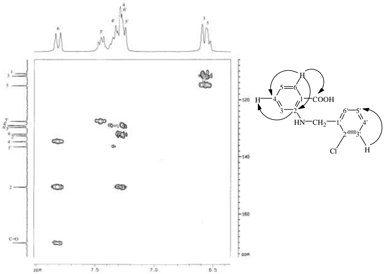
圖 66-5a HMBC (DMSO- d 6 ) spectrum of compound 66
