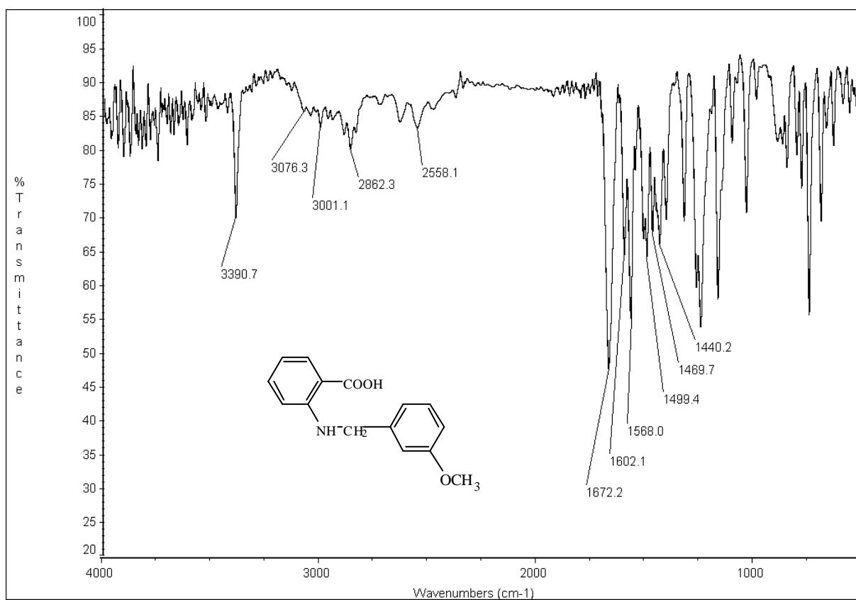
圖 72-2 IR (KBr) spectrum of compound 72
