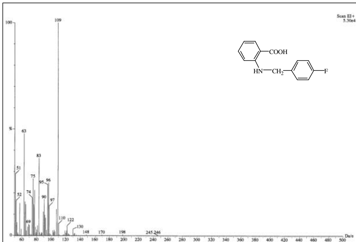
圖 71-1 MS spectrum of compound 71
