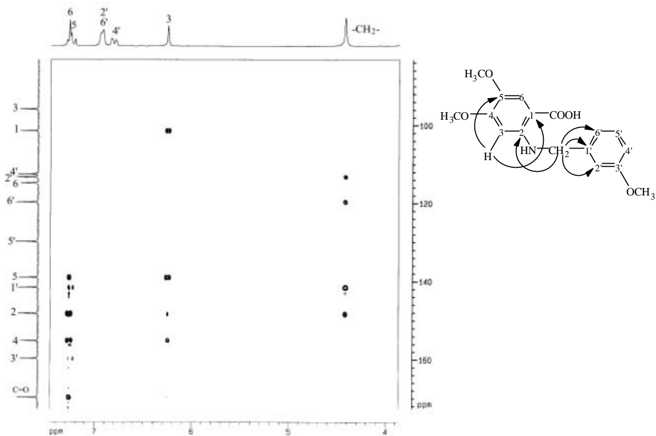
圖 74-5 HMBC (DMSO- d_6 ) spectrum of compound 74
