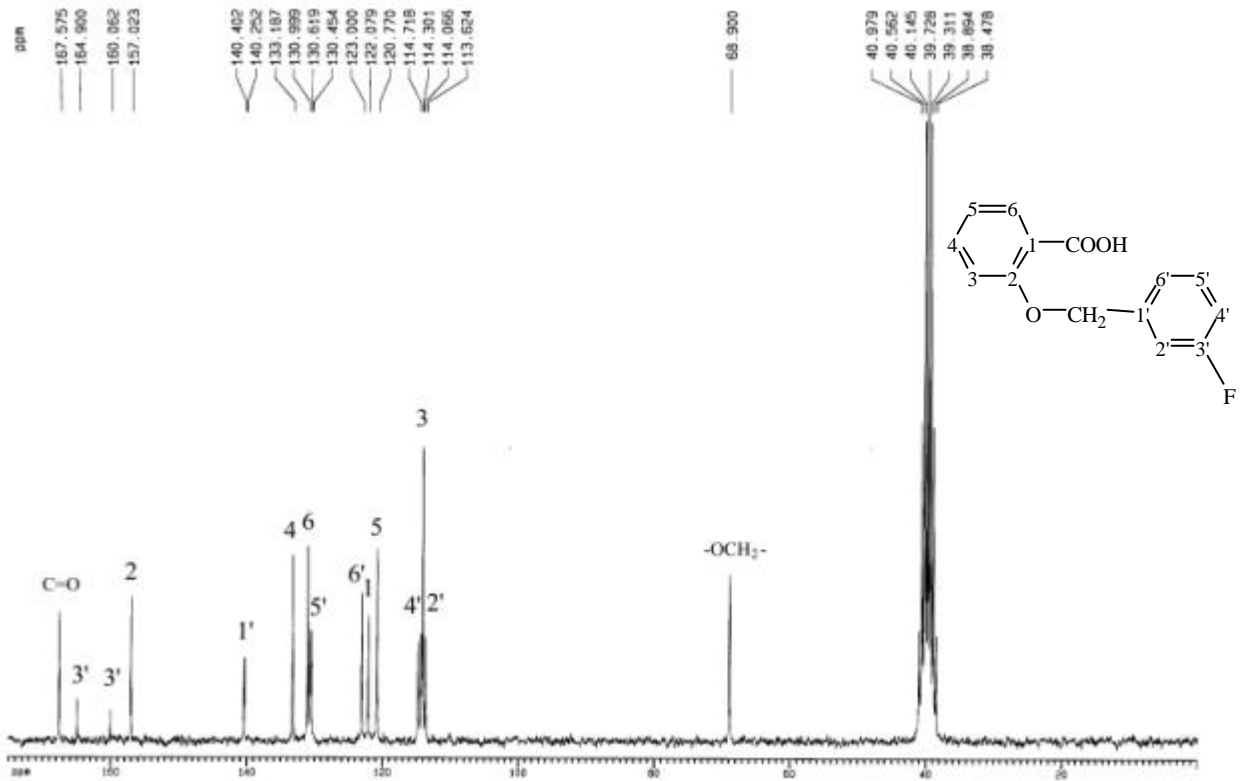
圖 61-4 13 C-NMR (DMSO- d 6 , 50 MHz) spectrum of compound 61
