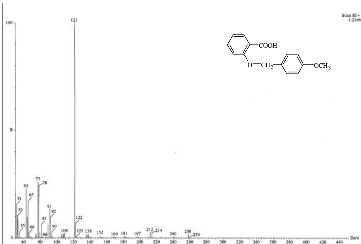
圖 64-1 MS spectrum of compound 64
