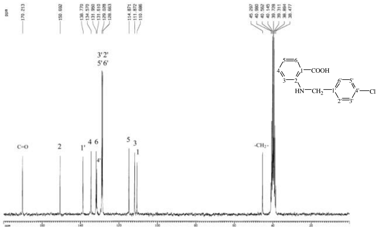
圖 68-4 ^{13}\text{C-NMR} ( \text{DMSO-}d_6 , 50 MHz) spectrum of compound 68
