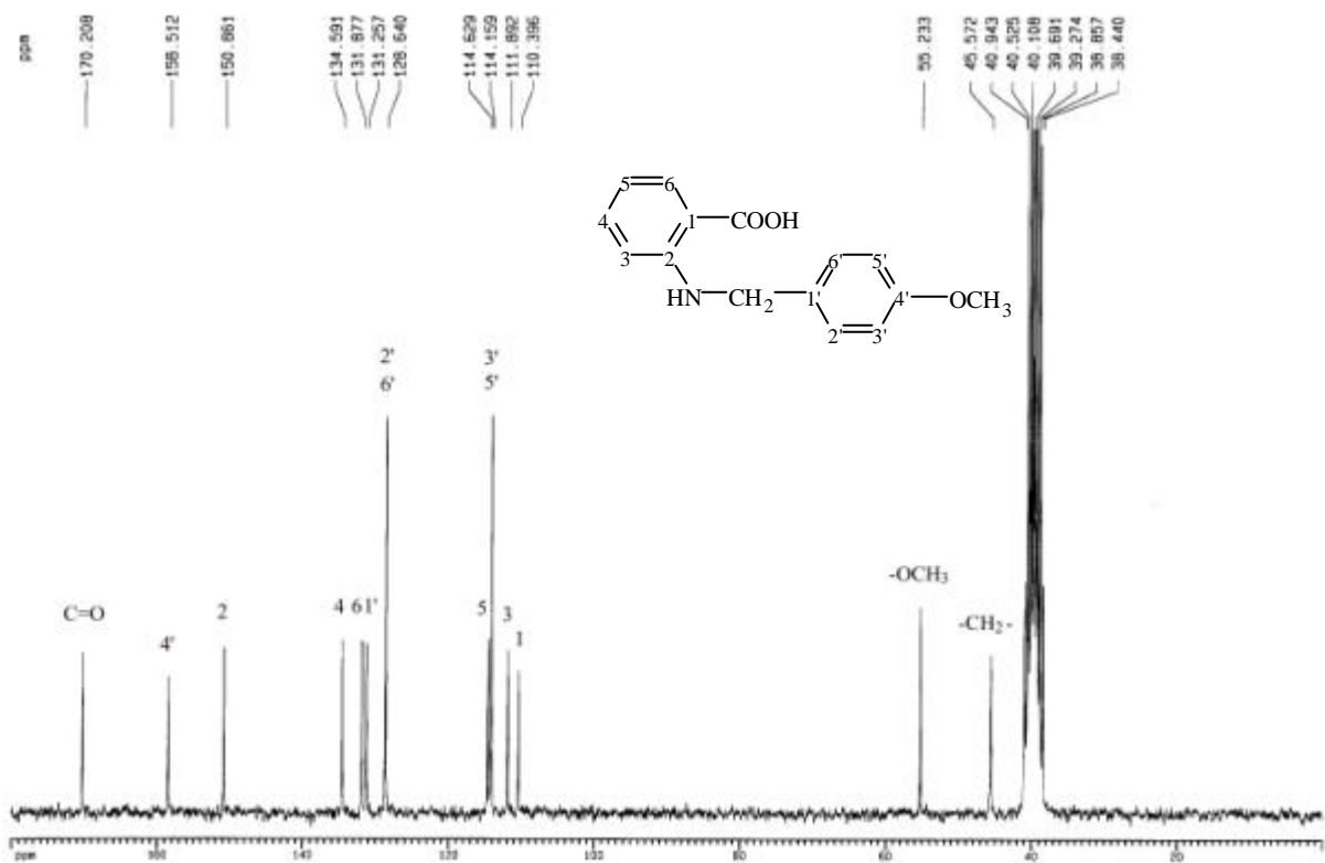
圖 73-4 13 C-NMR (DMSO- d 6 , 50 MHz) spectrum of compound 73
