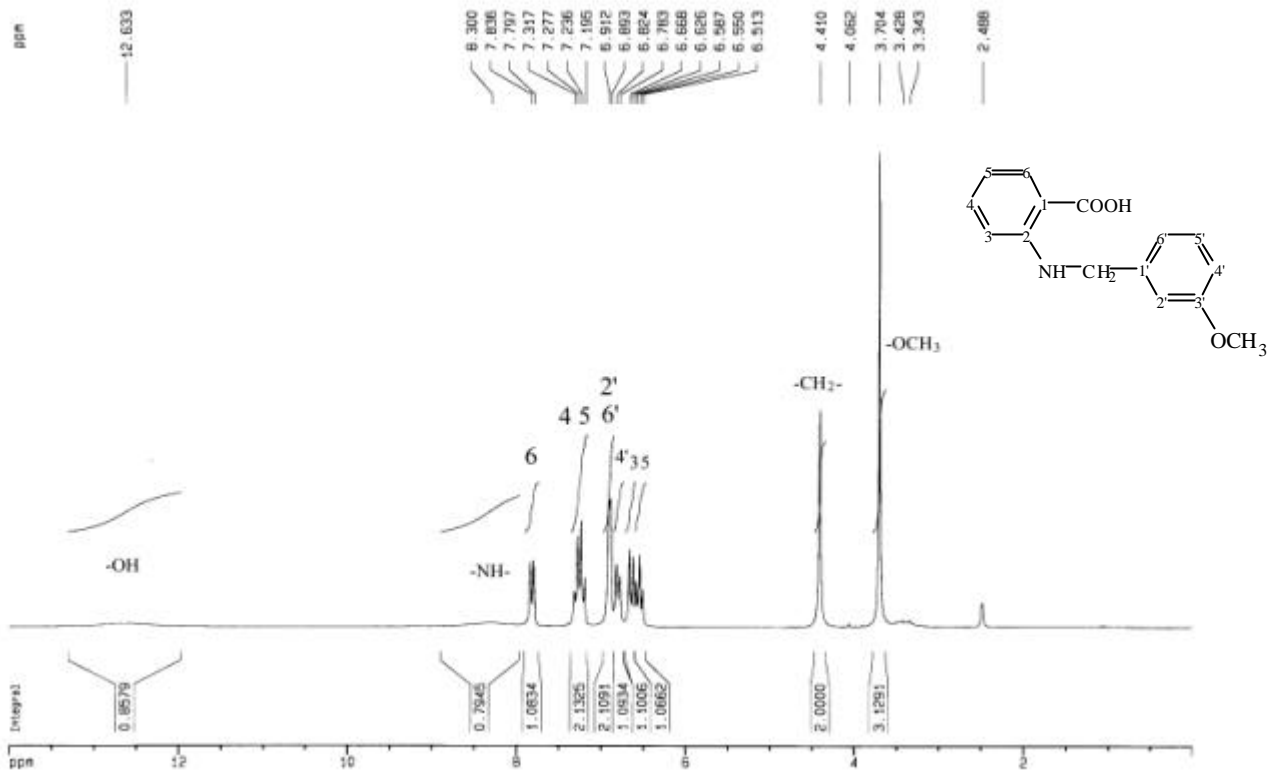
圖 72-3 ^1\text{H-NMR} (DMSO- d_6 , 200 MHz) spectrum of compound 72
