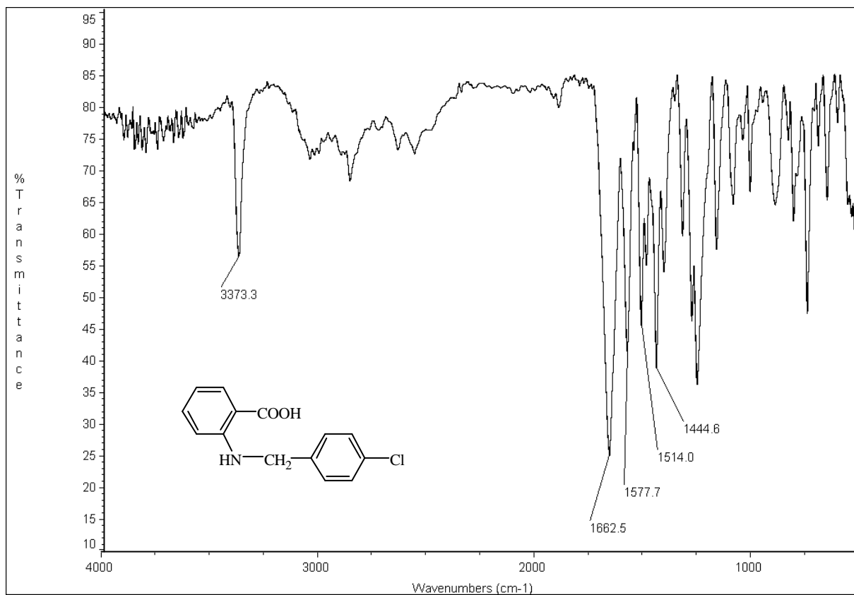
圖 68-2 IR (KBr) spectrum of compound 68
