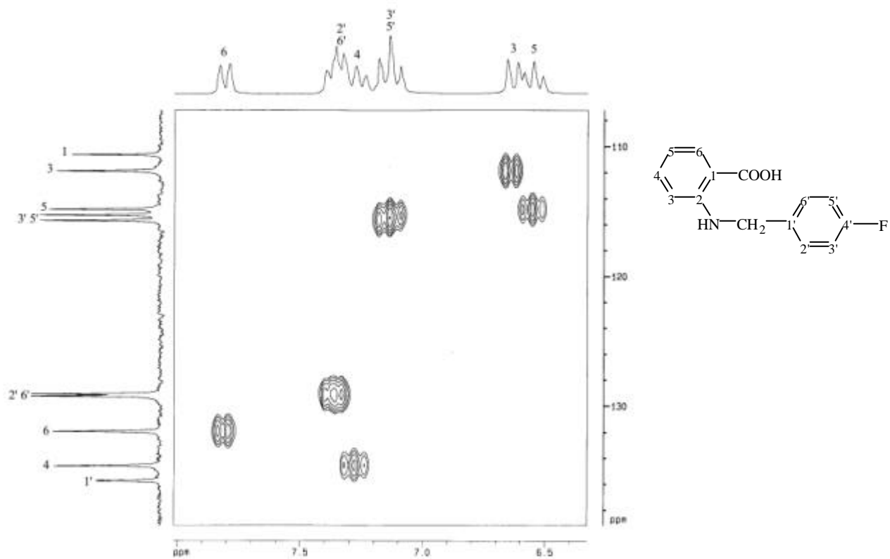
圖 71-6b HMQC (DMSO- d_6 ) spectrum of compound 71
