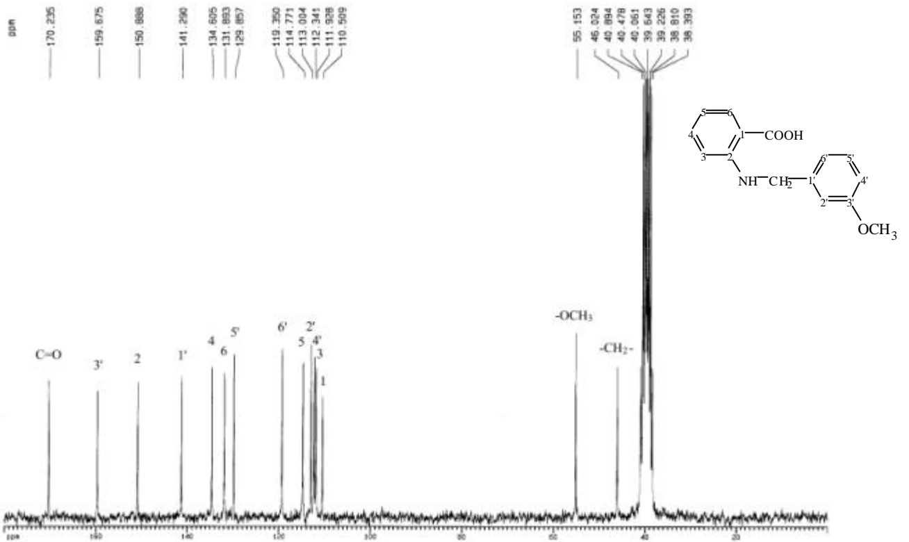
圖 72-4 ^{13}\text{C-NMR} (DMSO- d_6 , 50 MHz) spectrum of compound 72
