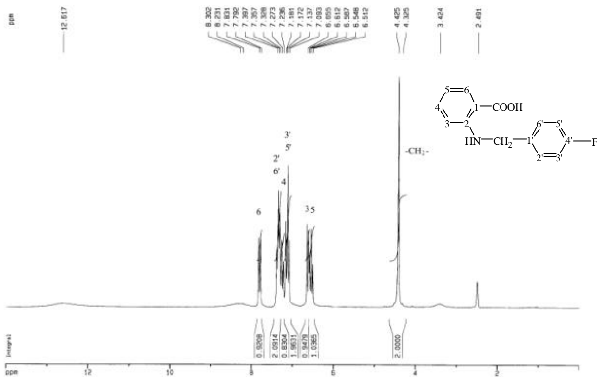
圖 71-3 ^1\text{H-NMR} ( \text{DMSO-}d_6 , 200 MHz) spectrum of compound 71
