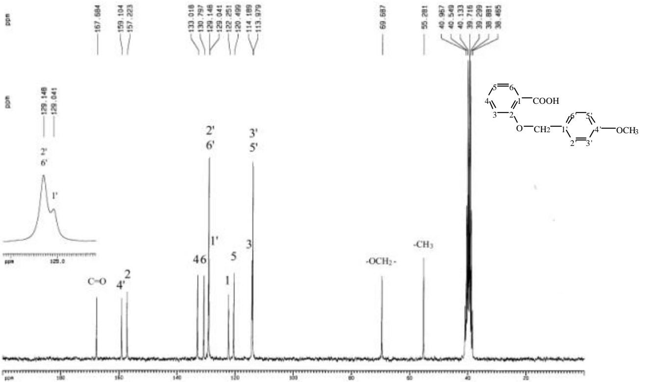
圖 64-4 13 C-NMR (DMSO- d 6 , 50 MHz) spectrum of compound 64
