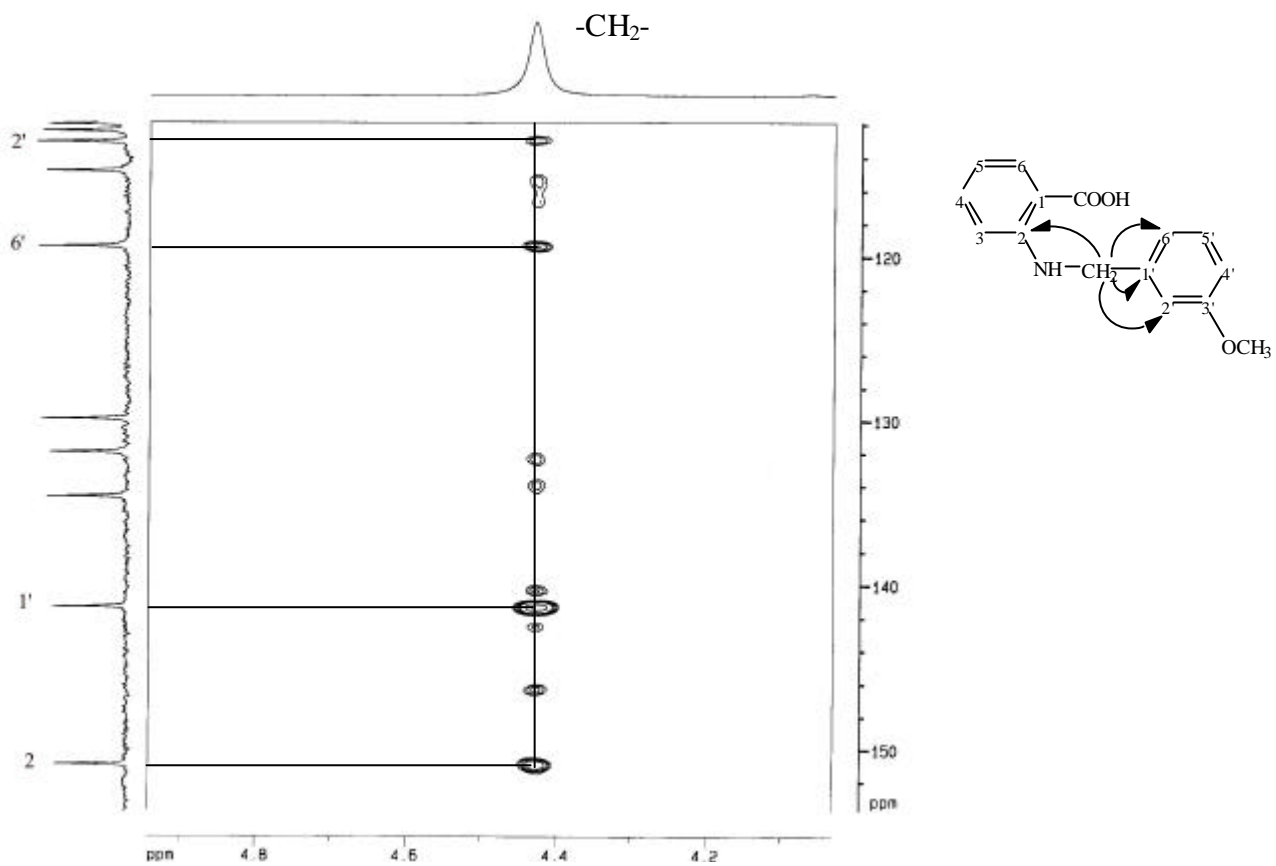
圖 72-5a HMBC (DMSO- d_6 ) spectrum of compound 72
