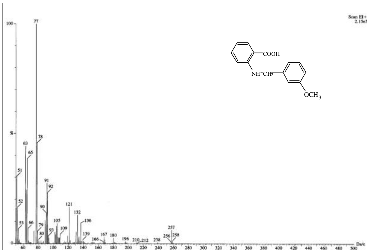
圖 72-1 MS spectrum of compound 72
