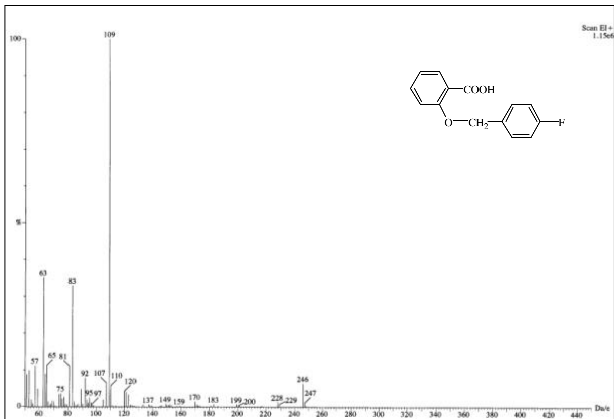
圖 62-1 MS spectrum of compound 62
