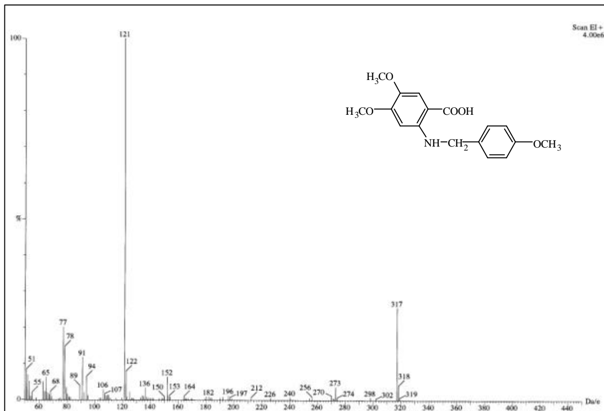
圖 75-1 MS spectrum of compound 75
