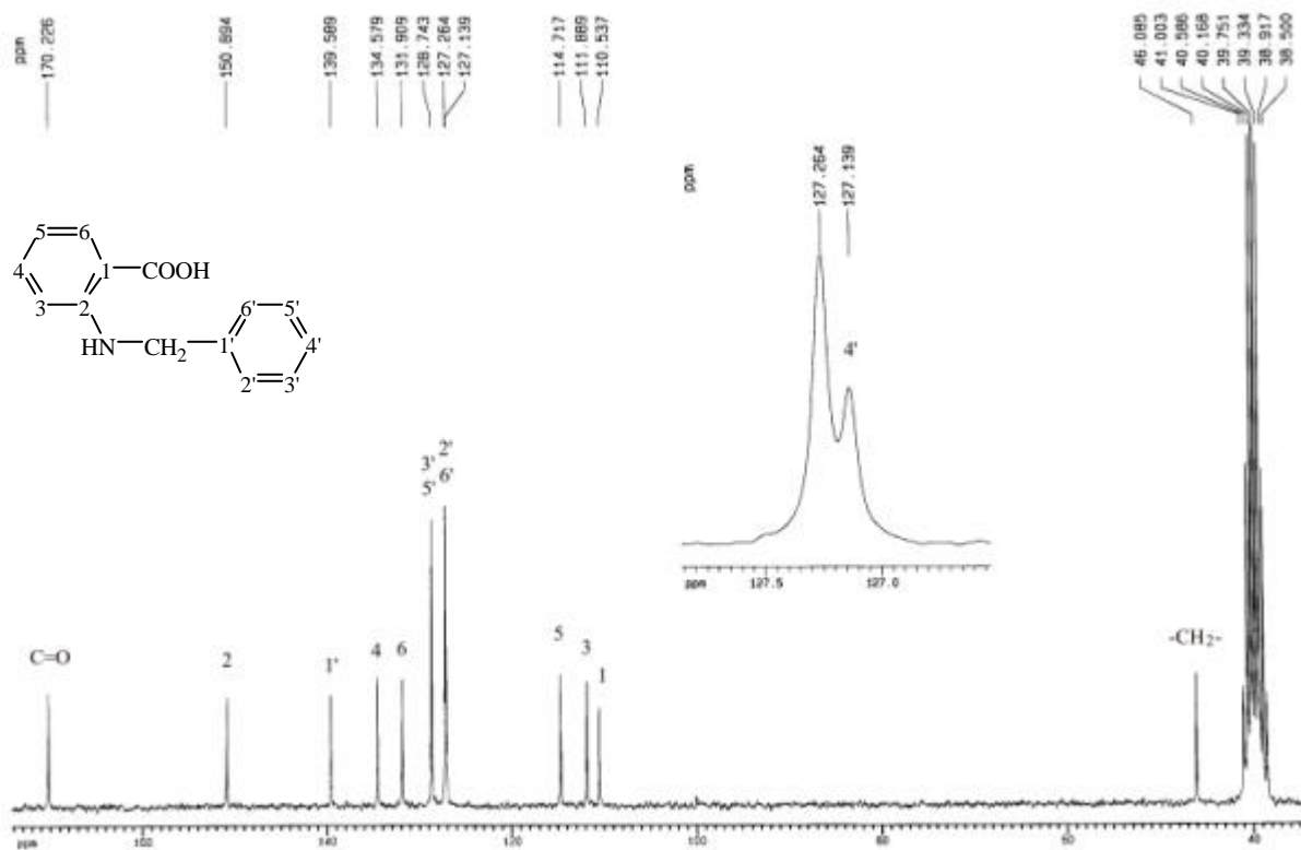
圖 65-4 ^{13}\text{C-NMR} ( \text{DMSO-}d_6 , 50 MHz) spectrum of compound 65
