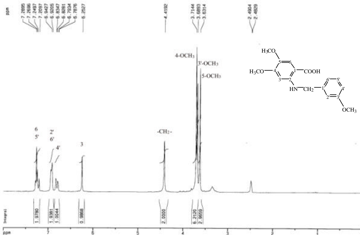
圖 74-3 1 H-NMR (DMSO- d 6 , 200 MHz) spectrum of compound 74
