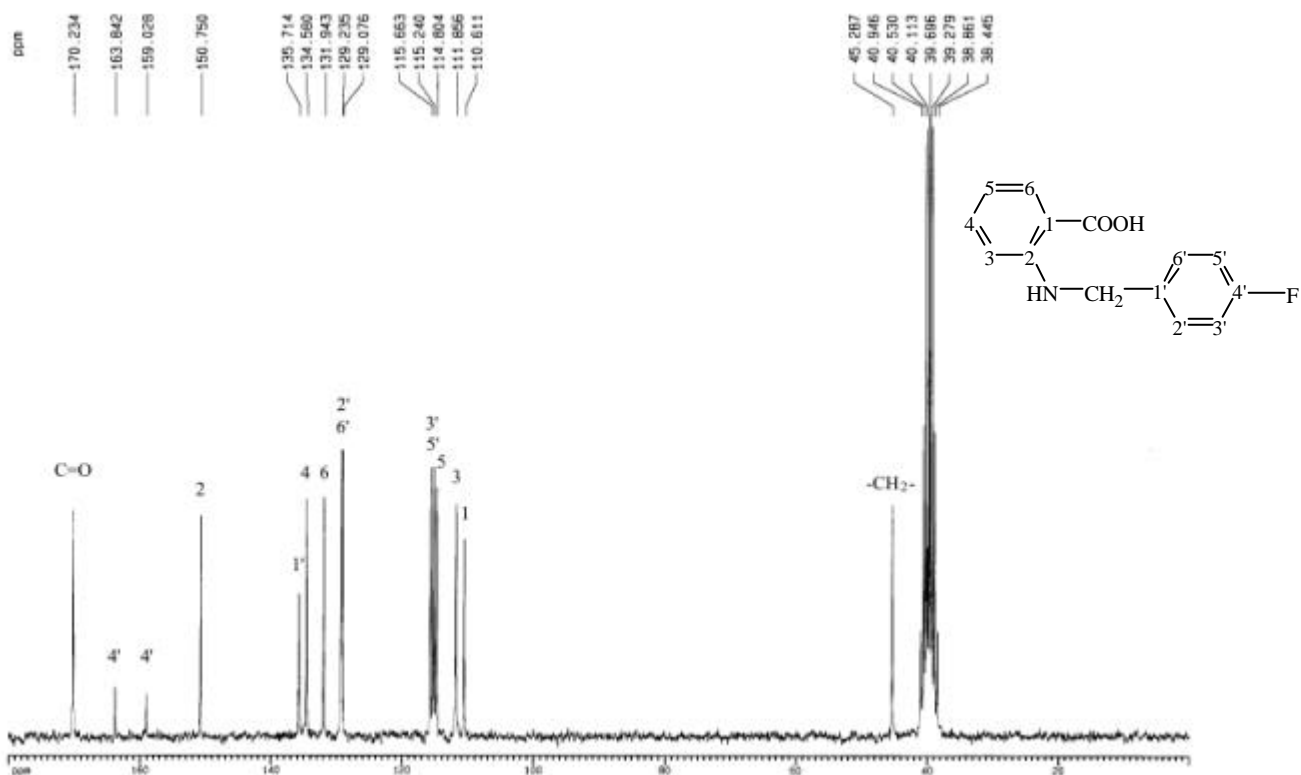
圖 71-4 ^{13}\text{C-NMR} ( \text{DMSO-}d_6 , 50 MHz) spectrum of compound 71
