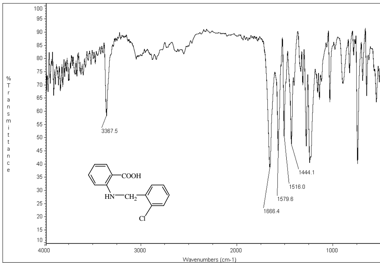
圖 66-2 IR (KBr) spectrum of compound 66
