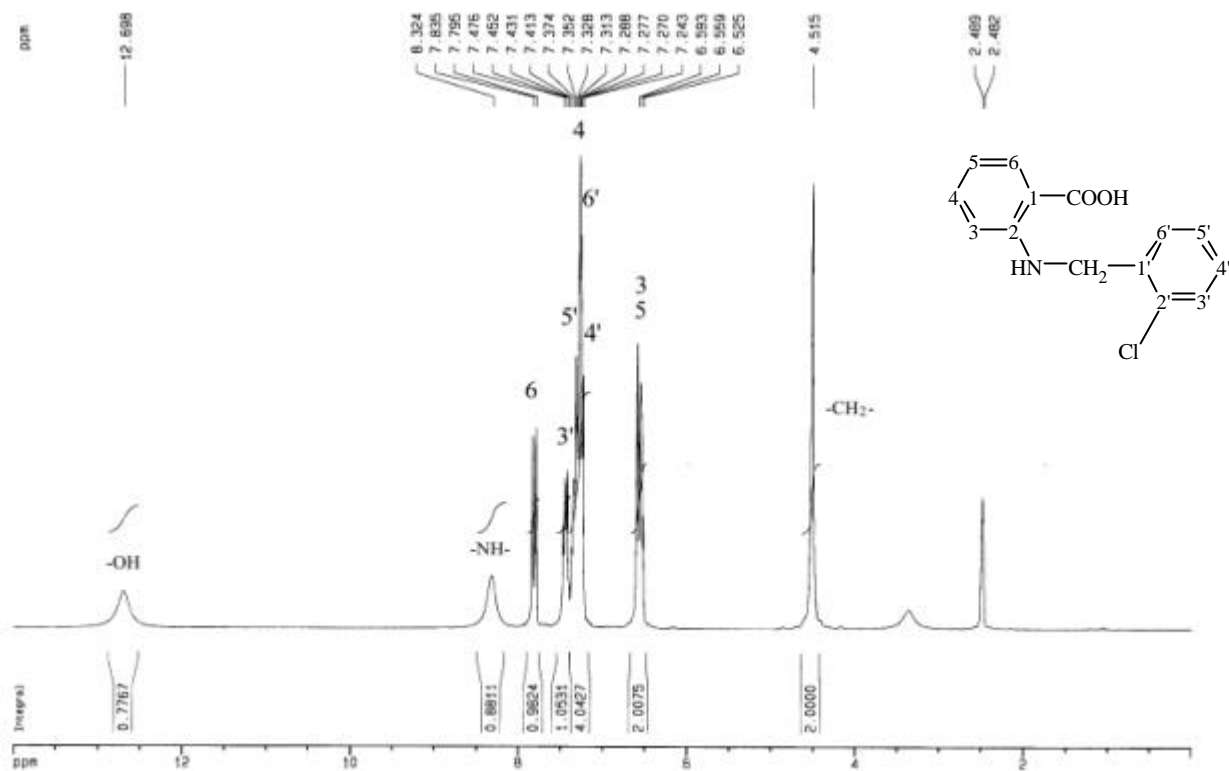
圖 66-3 ^1\text{H-NMR} ( \text{DMSO-}d_6 , 200 MHz) spectrum of compound 66
