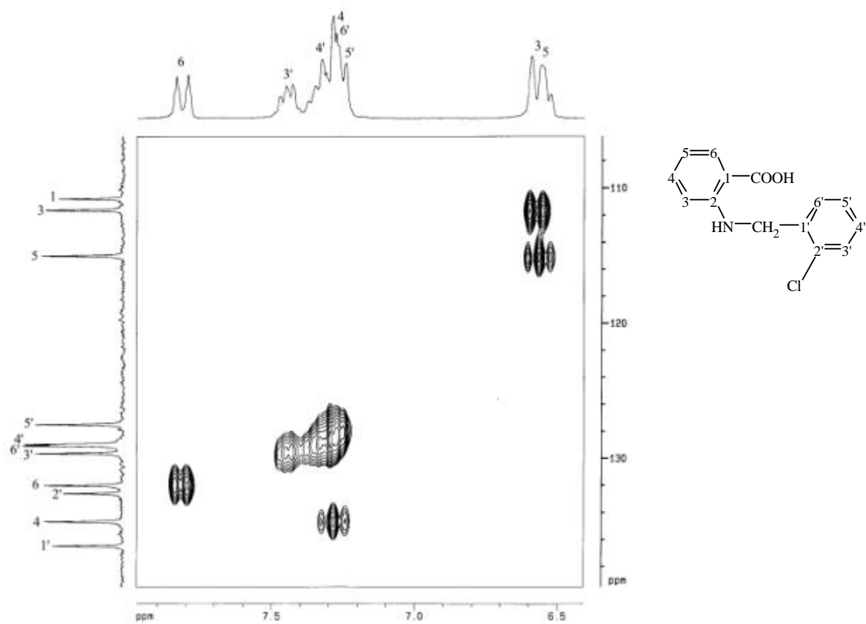
圖 66-6b HMQC (DMSO- d_6 ) spectrum of compound 66
