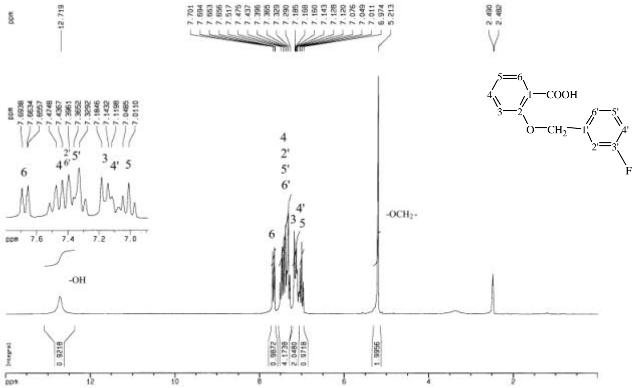
圖 61-3 1 H-NMR (DMSO- d 6 , 200 MHz) spectrum of compound 61
