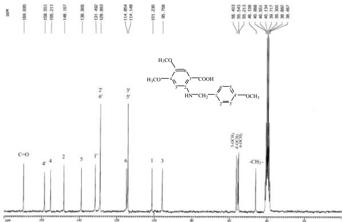
圖 75-4 13 C-NMR (DMSO- d 6 , 50 MHz) spectrum of compound 75
