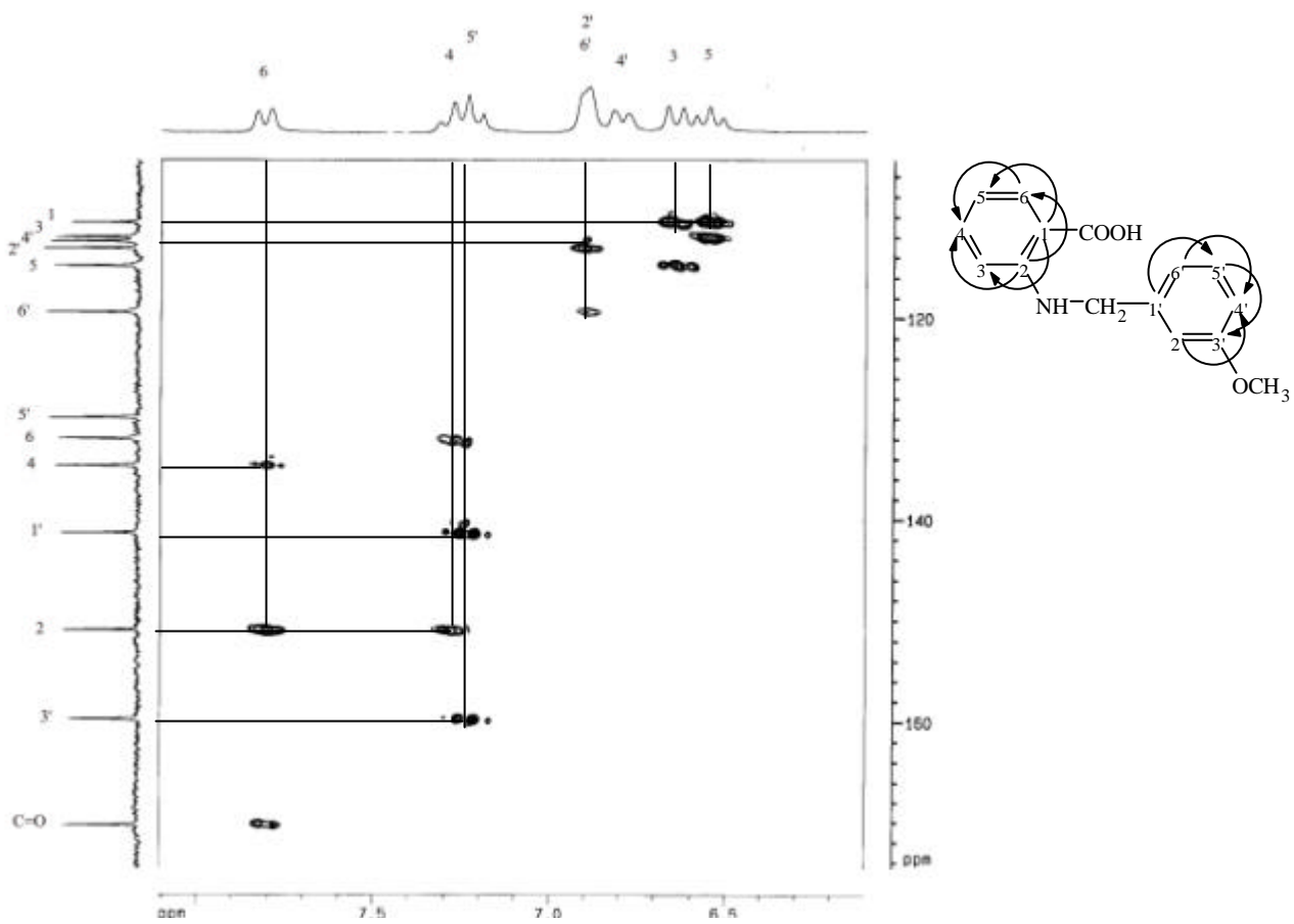
圖 72-5b HMBC (DMSO- d_6 ) spectrum of compound 72
