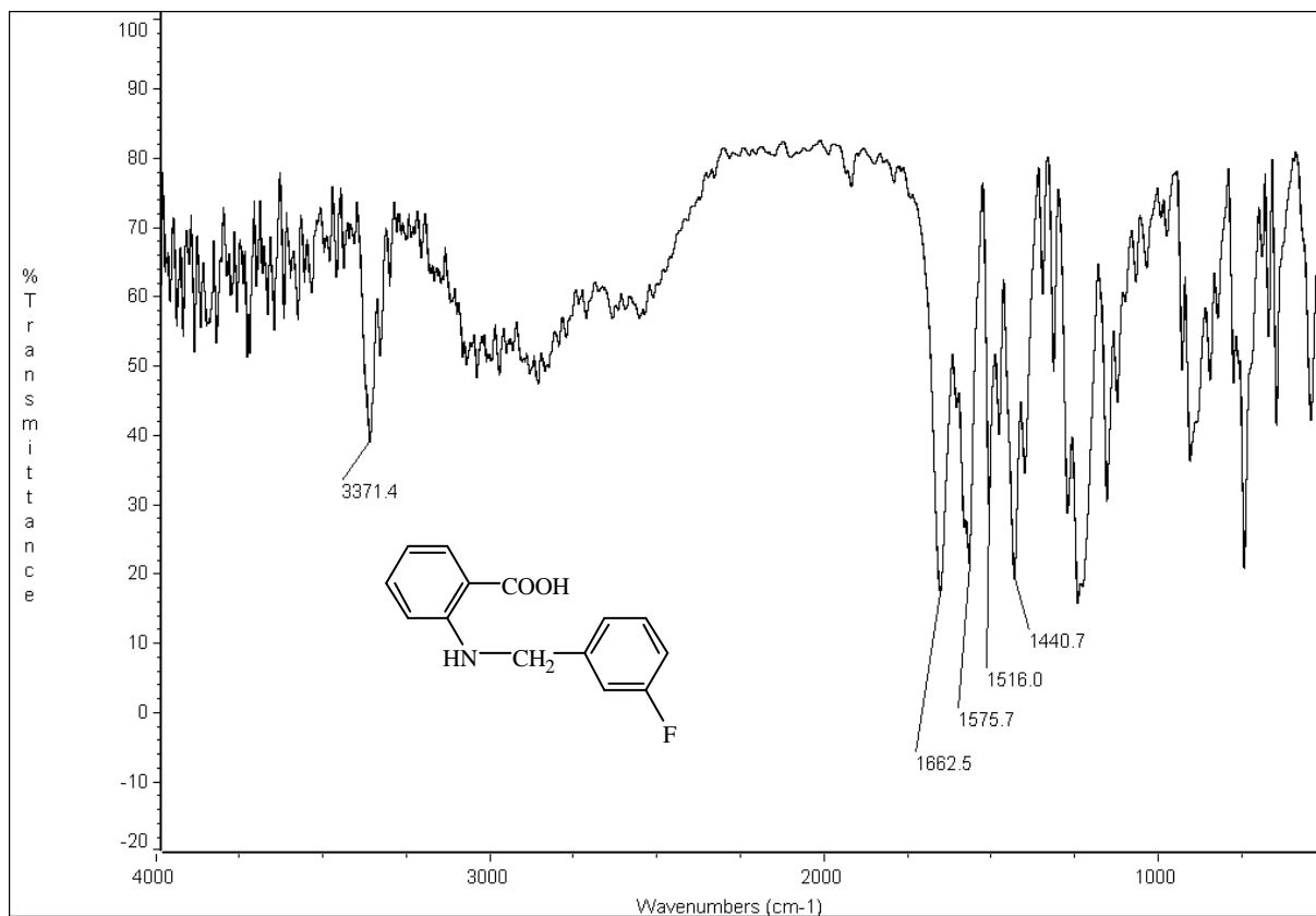
圖 70-2 IR (KBr) spectrum of compound 70
