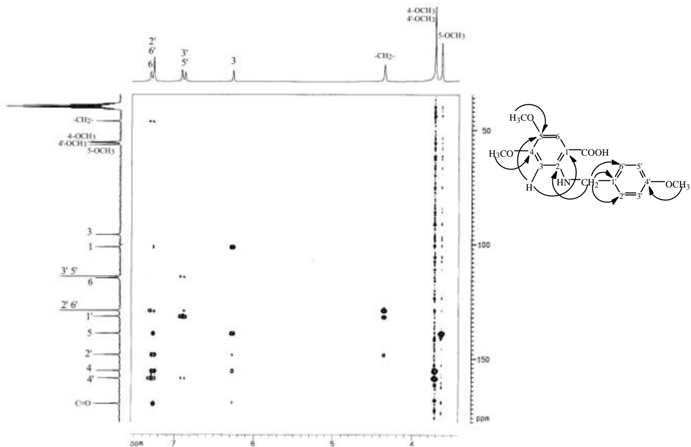
圖 75-5 HMBC (DMSO- d_6 ) spectrum of compound 75
