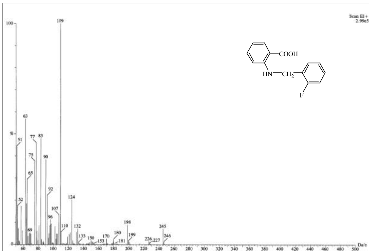
圖 69-1 MS spectrum of compound 69
