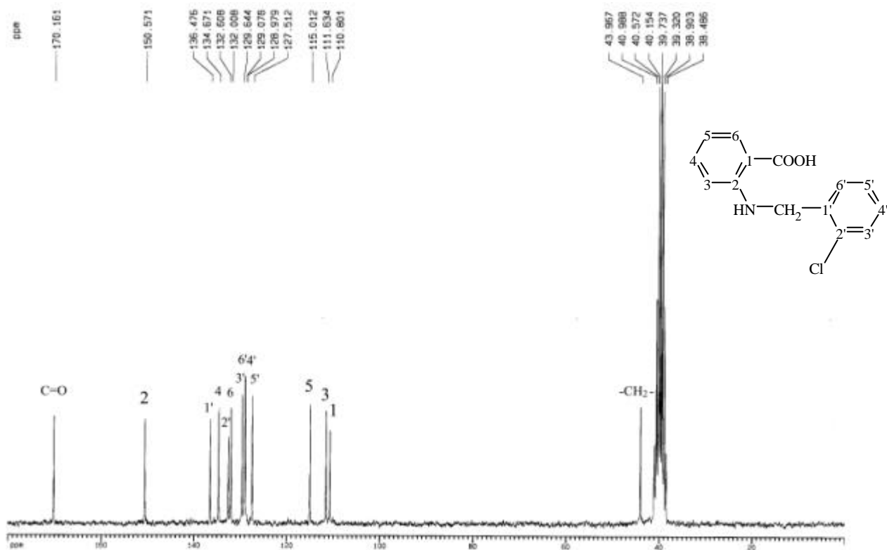
圖 66-4 ^{13}\text{C-NMR} ( \text{DMSO-}d_6 , 50 MHz) spectrum of compound 66
