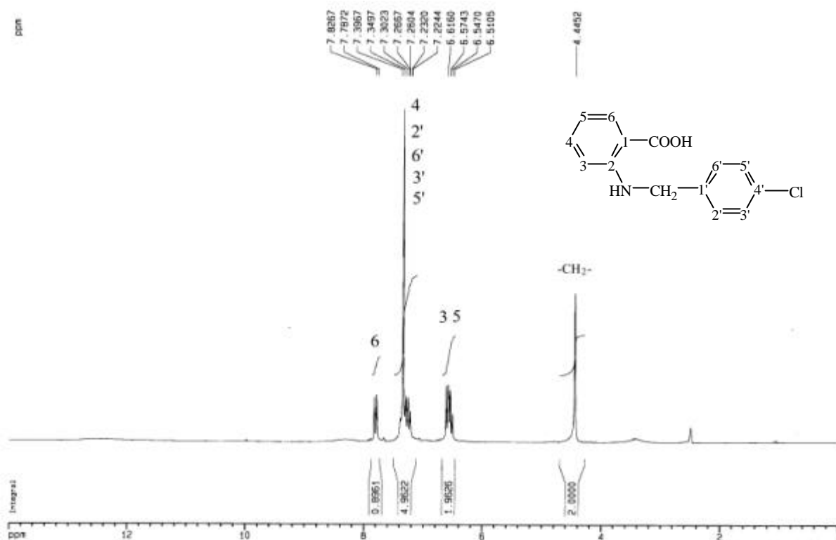
圖 68-3 ^1\text{H-NMR} ( \text{DMSO-}d_6 , 200 MHz) spectrum of compound 68
