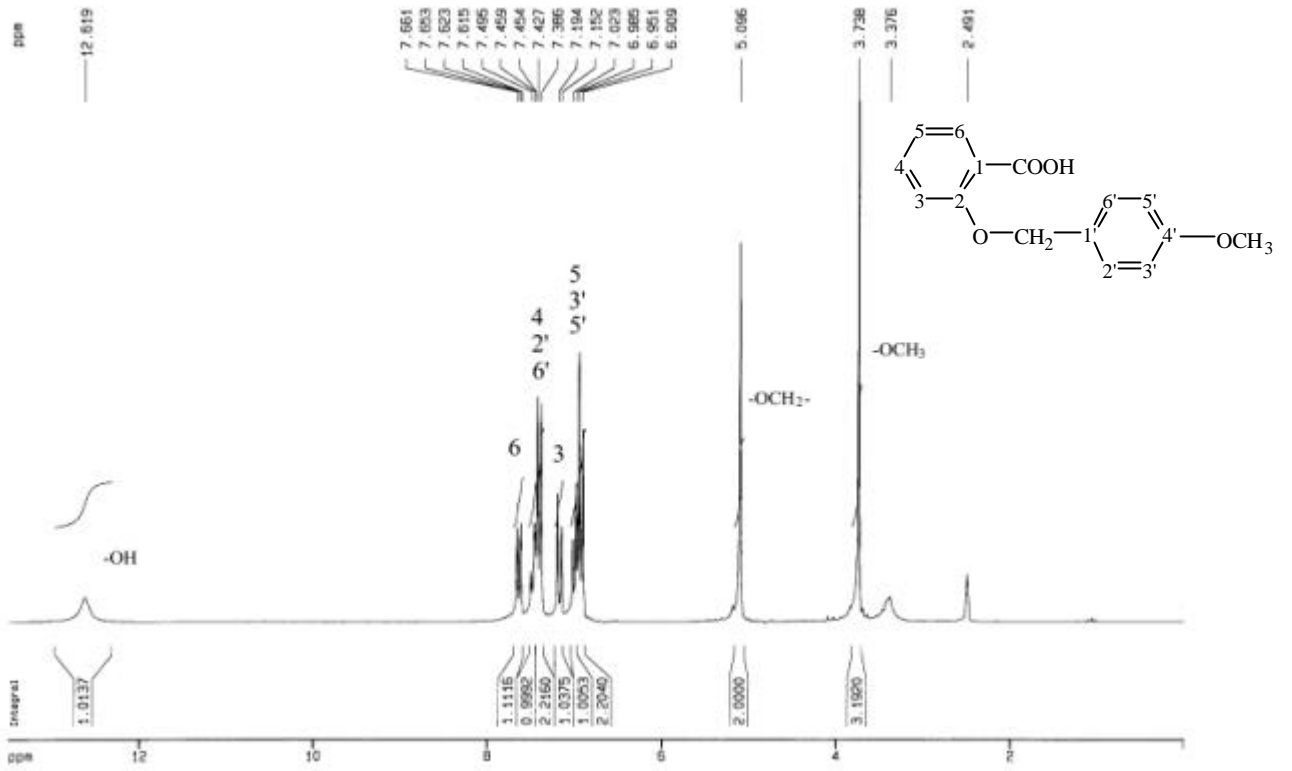
圖 64-3 1 H-NMR (DMSO- d 6 , 200 MHz) spectrum of compound 64
