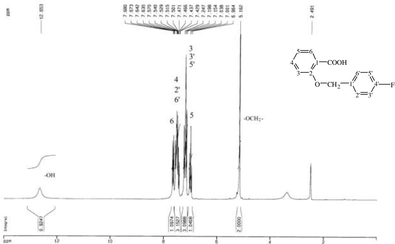
圖 62-3 1 H-NMR (DMSO- d 6 , 200 MHz) spectrum of compound 62
