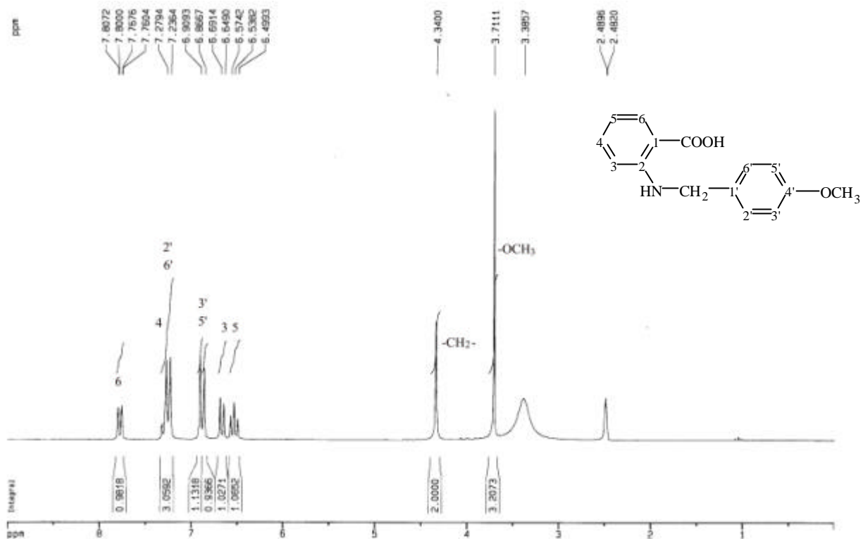
圖 73-3 1 H-NMR (DMSO- d 6 , 200 MHz) spectrum of compound 73
