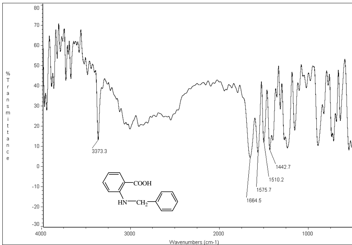
圖 65-2 IR (KBr) spectrum of compound 65
