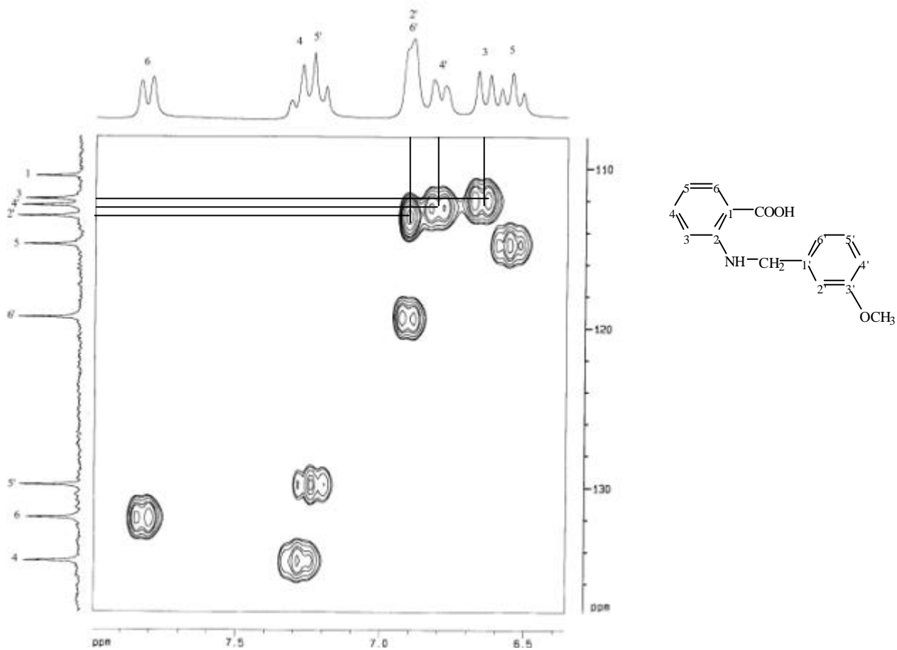
圖 72-6b HMQC (DMSO- d_6 ) spectrum of compound 72
