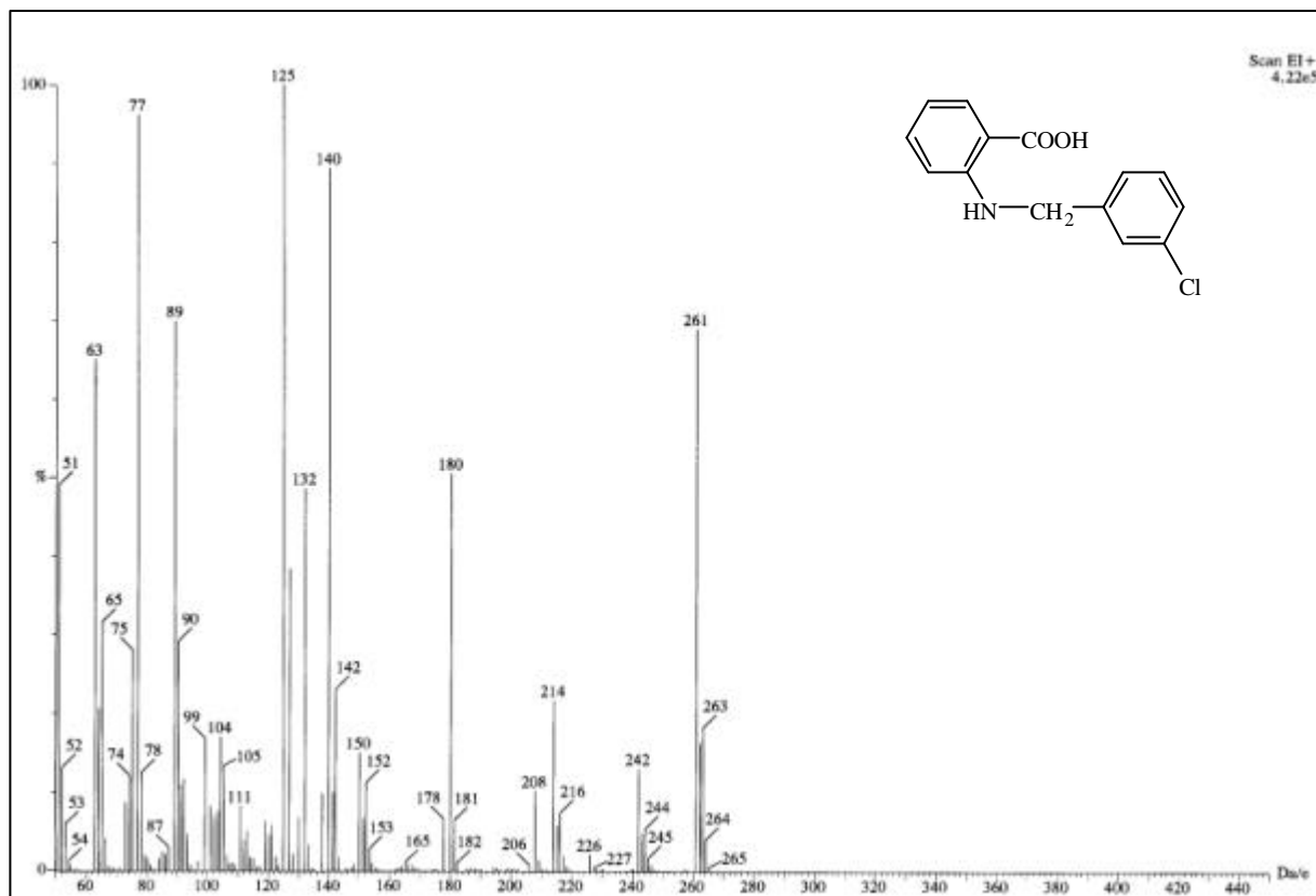
圖 67-1 MS spectrum of compound 67
