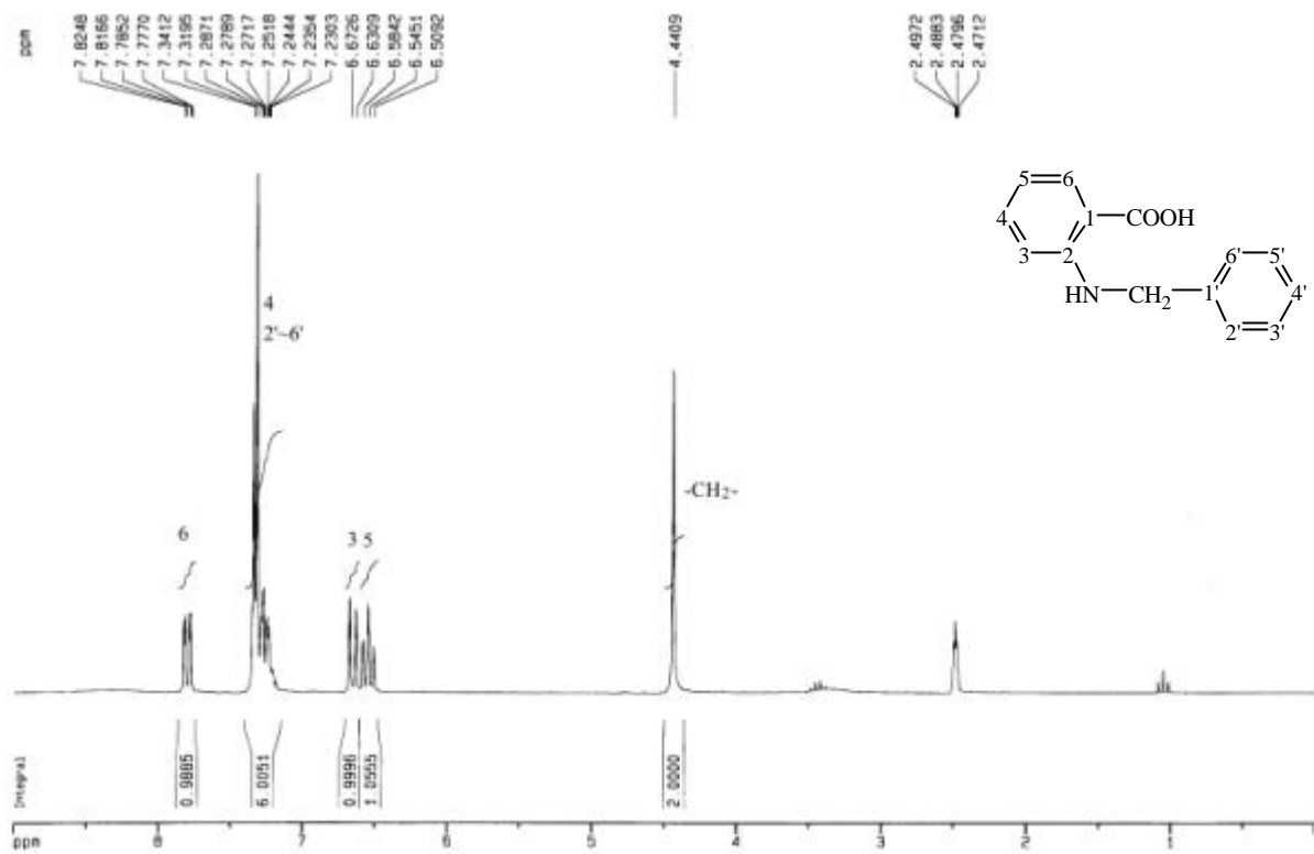
圖 65-3 ^1\text{H-NMR} ( \text{DMSO-}d_6 , 200 MHz) spectrum of compound 65
