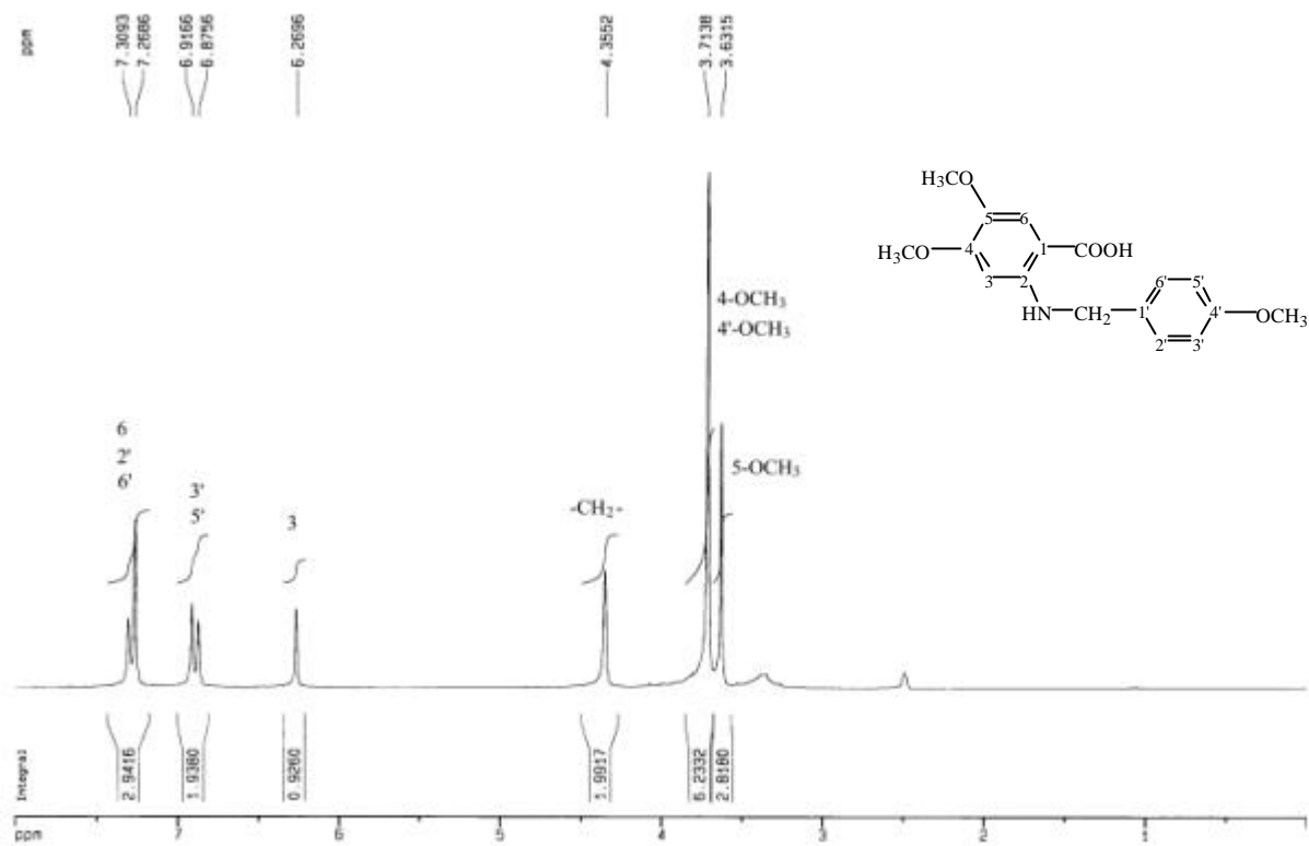
圖 75-3 1 H-NMR (DMSO- d 6 , 200 MHz) spectrum of compound 75
