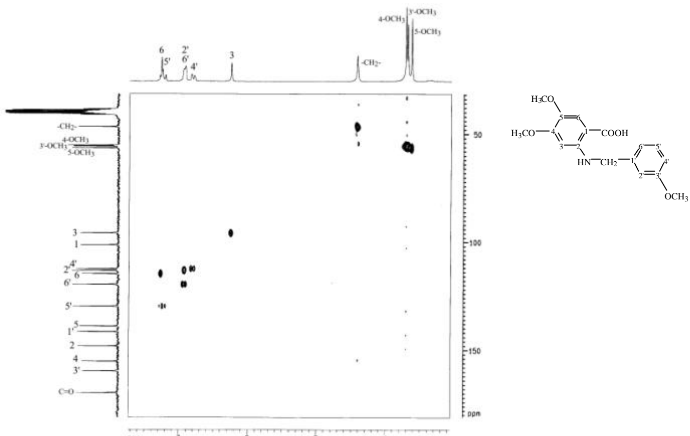
圖 74-6 HMQC (DMSO- d_6 ) spectrum of compound 74
