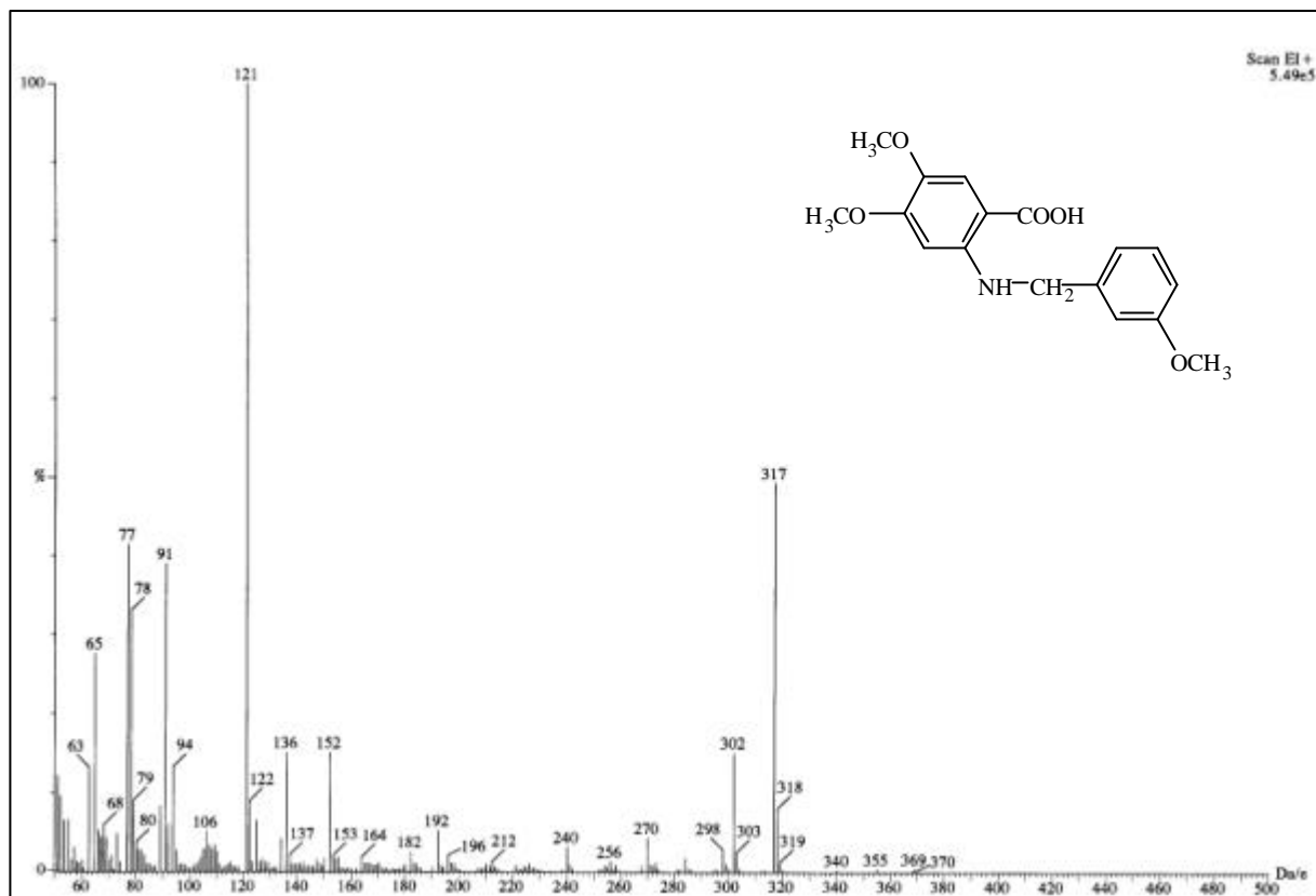
圖 74-1 MS spectrum of compound 74
