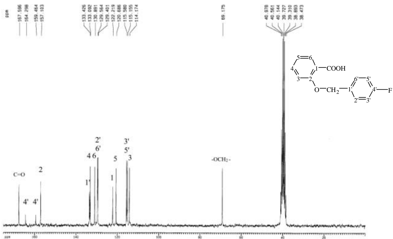
圖 62-4 13 C-NMR (DMSO- d 6 , 50 MHz) spectrum of compound 62
