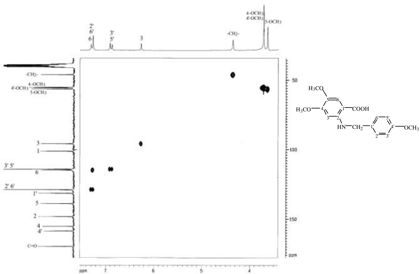
圖 75-6 HMQC (DMSO- d_6 ) spectrum of compound 75
