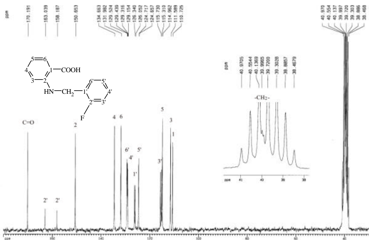
圖 69-4 13 C-NMR (DMSO- d 6 , 50 MHz) spectrum of compound 69
