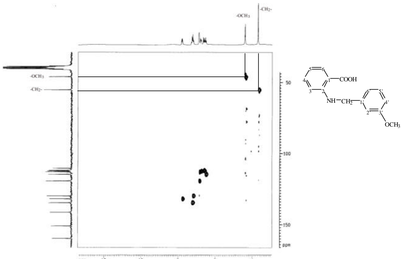
圖 72-6a HMQC (DMSO- d_6 ) spectrum of compound 72
