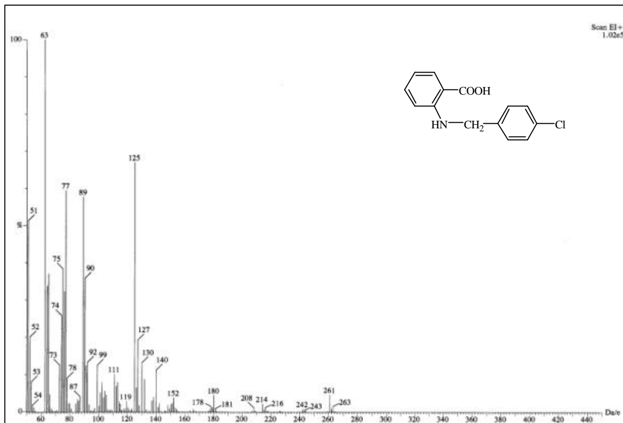
圖 68-1 MS spectrum of compound 68
