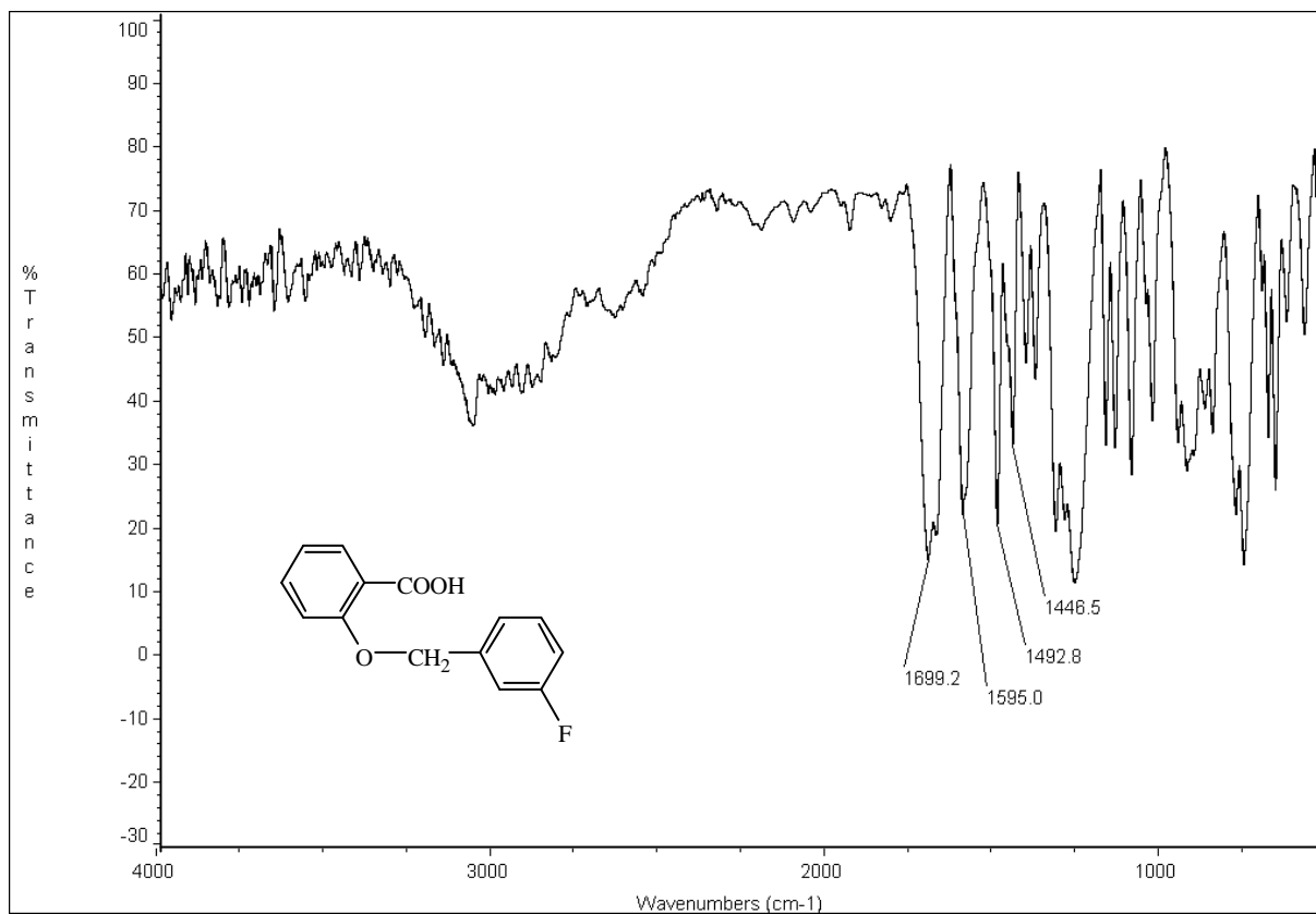
圖 61-2 IR (KBr) spectrum of compound 61
