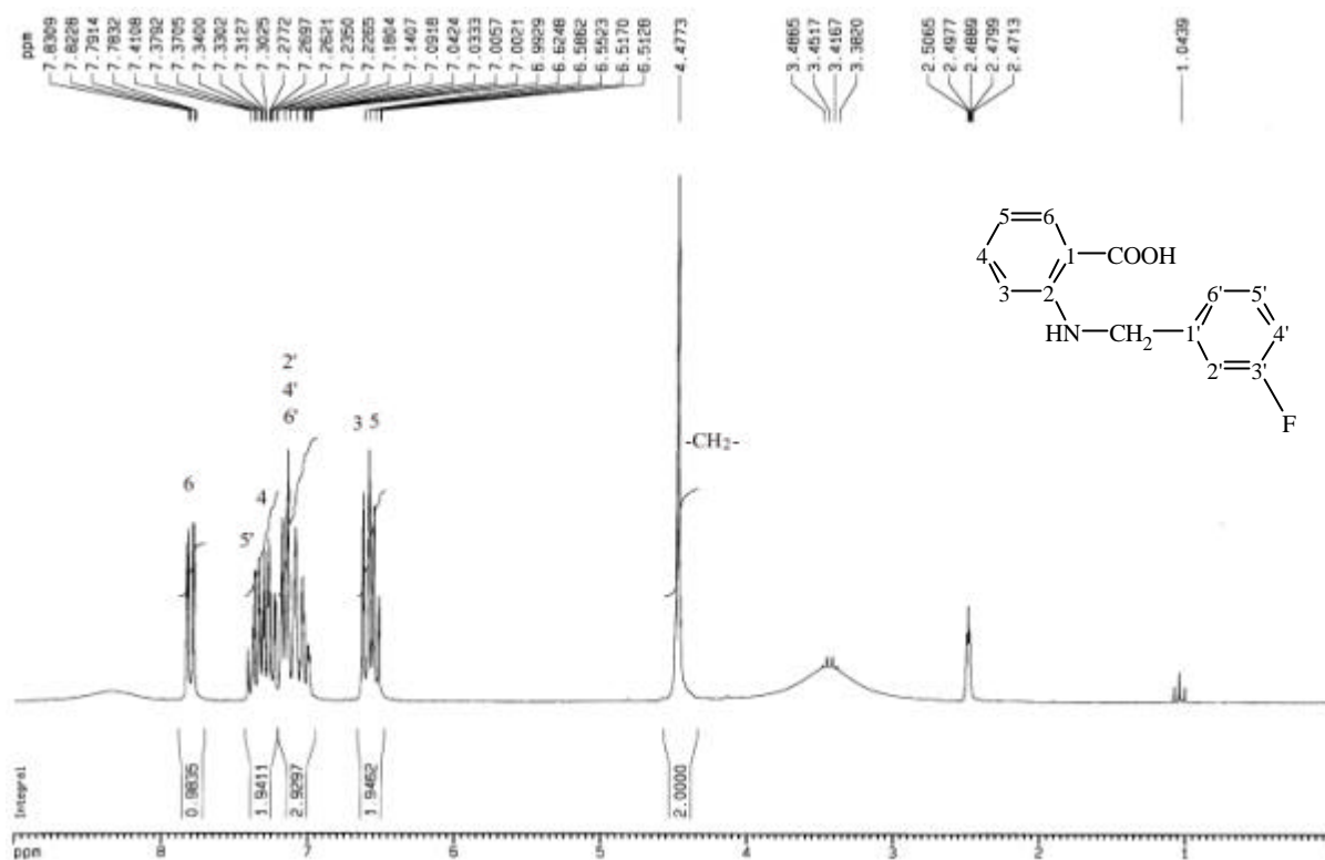
圖 70-3 1 H-NMR (DMSO- d 6 , 200 MHz) spectrum of compound 70
