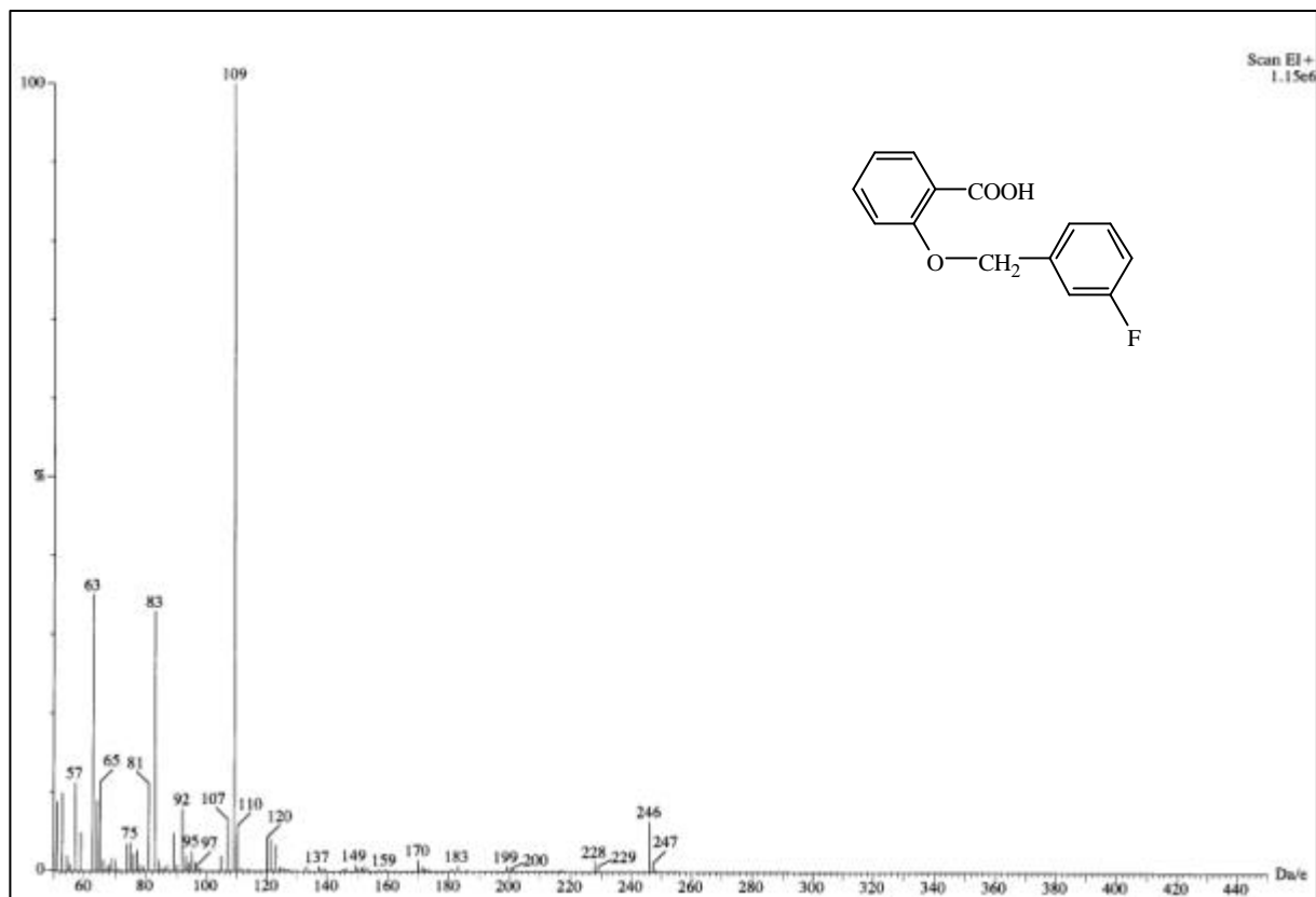
圖 61-1 MS spectrum of compound 61
