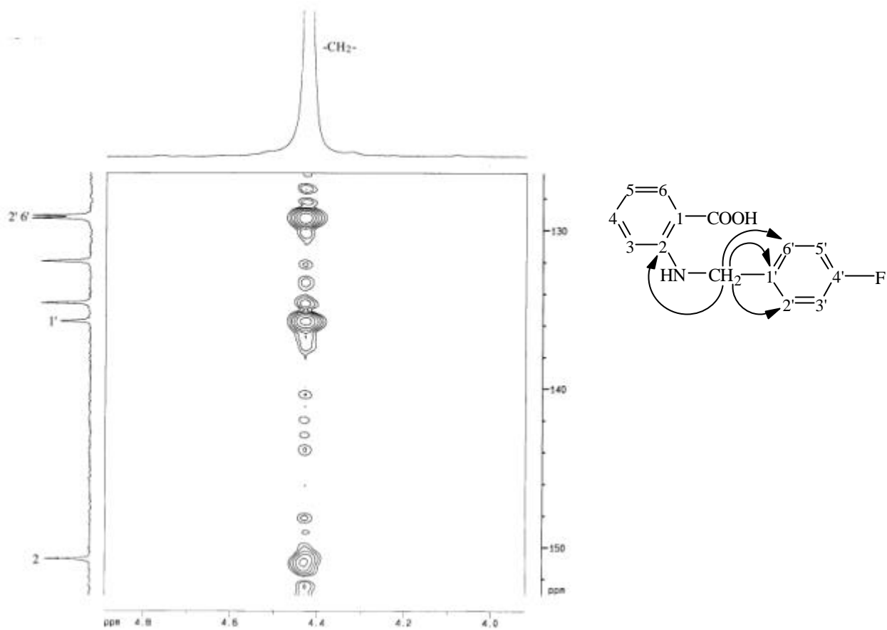
圖 71-5a HMBC (DMSO- d_6 ) spectrum of compound 71
