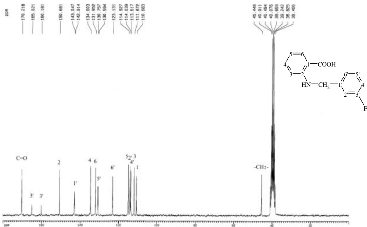
圖 70-4 13 C-NMR (DMSO- d 6 , 50 MHz) spectrum of compound 70
