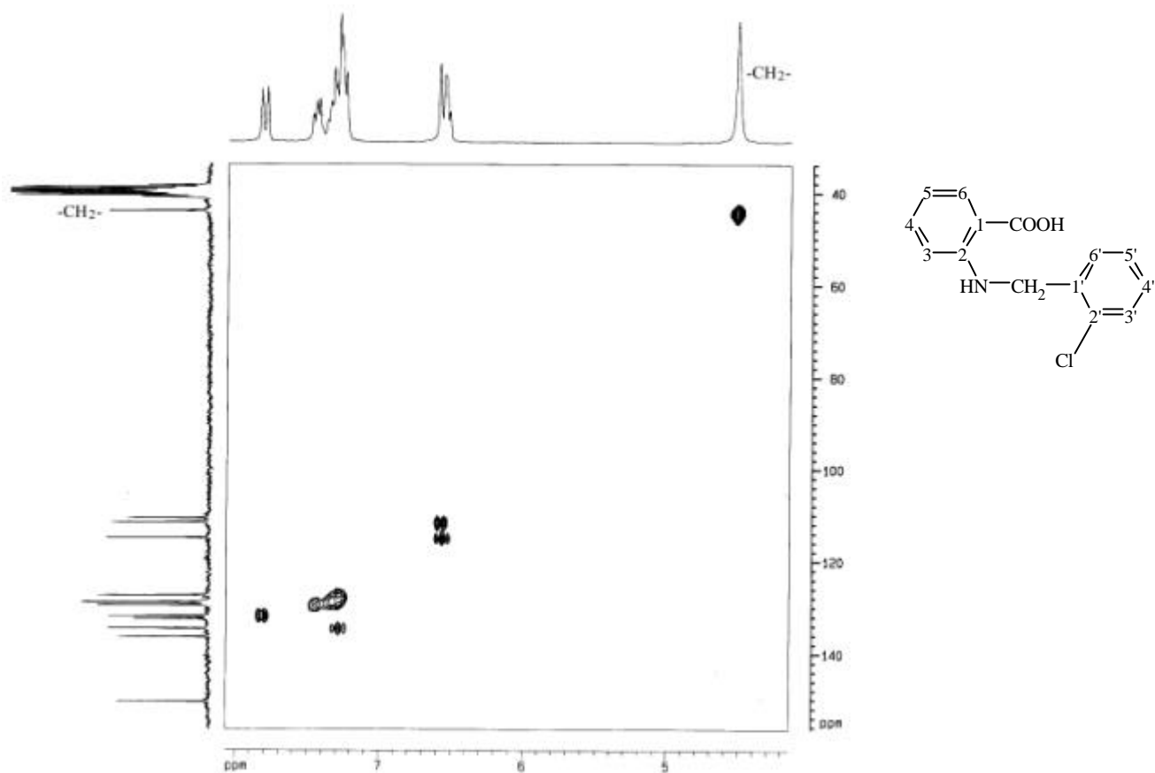
圖 66-6a HMQC (DMSO- d_6 ) spectrum of compound 66
