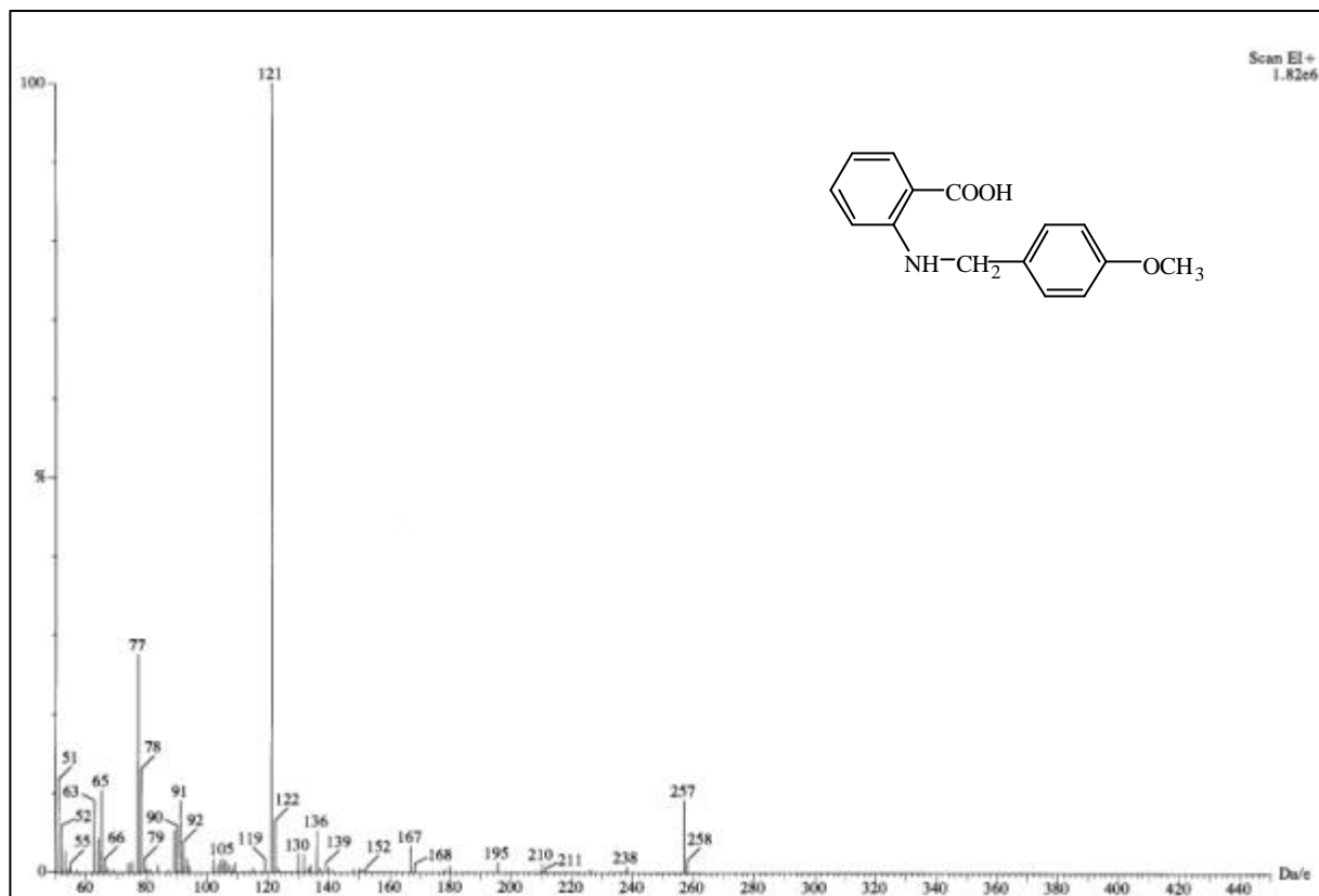
圖 73-1 MS spectrum of compound 73
