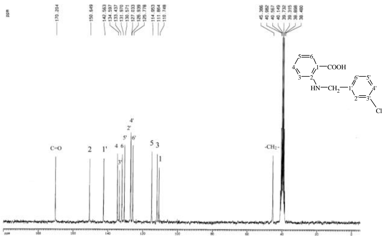
圖 67-4 ^{13}\text{C-NMR} (DMSO- d_6 , 50 MHz) spectrum of compound 67
