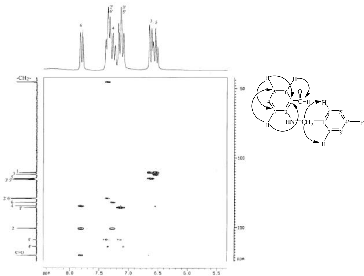
圖 71-5b HMBC (DMSO- d_6 ) spectrum of compound 71
