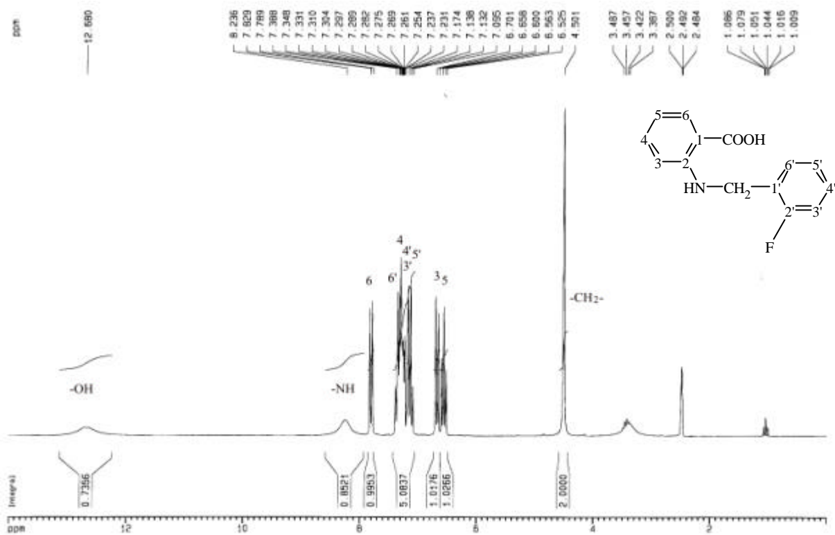
圖 69-3 1 H-NMR (DMSO- d 6 , 200 MHz) spectrum of compound 69
