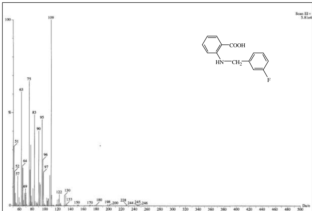
圖 70-1 MS spectrum of compound 70
