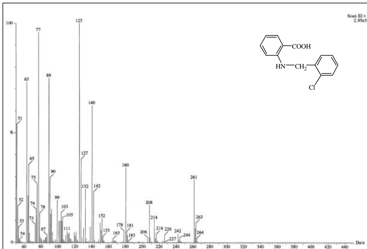
圖 66-1 MS spectrum of compound 66
