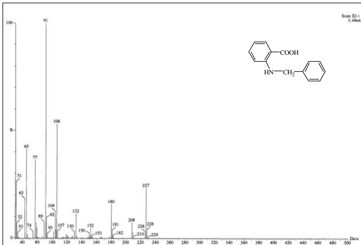
圖 65-1 MS spectrum of compound 65
