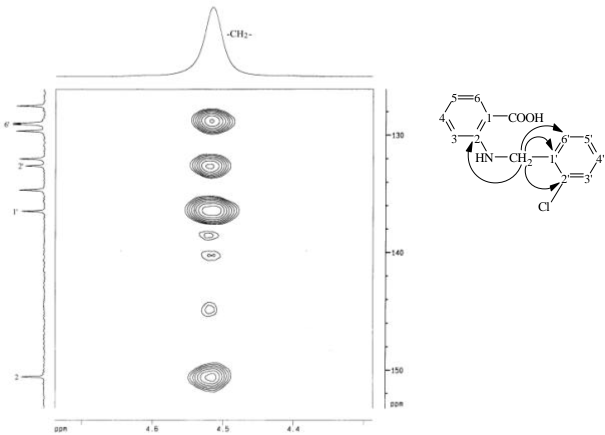
圖 66-5b HMBC (DMSO- d 6 ) spectrum of compound 66
