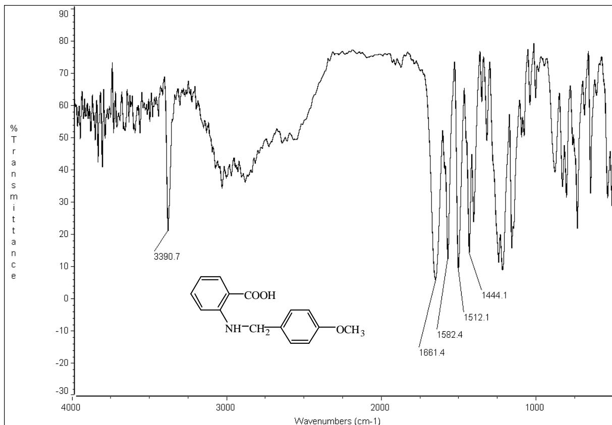
圖 73-2 IR (KBr) spectrum of compound 73
