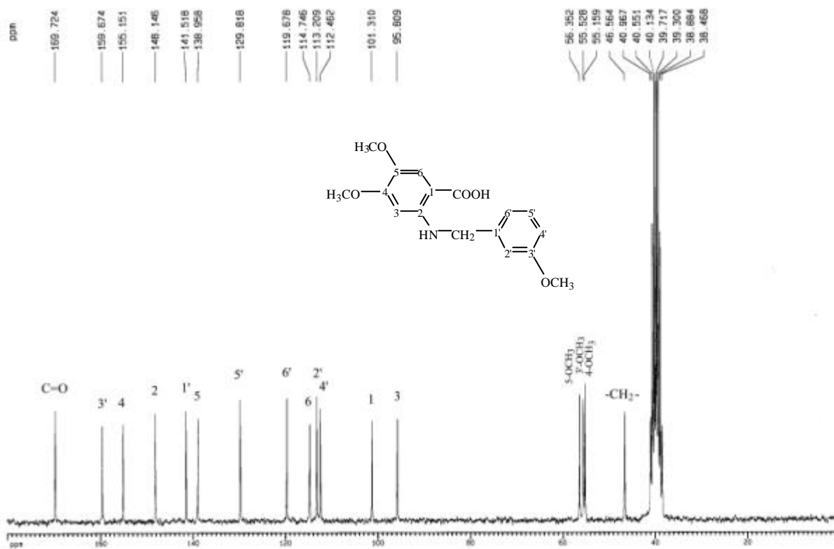
圖 74-4 13 C-NMR (DMSO- d 6 , 50 MHz) spectrum of compound 74
