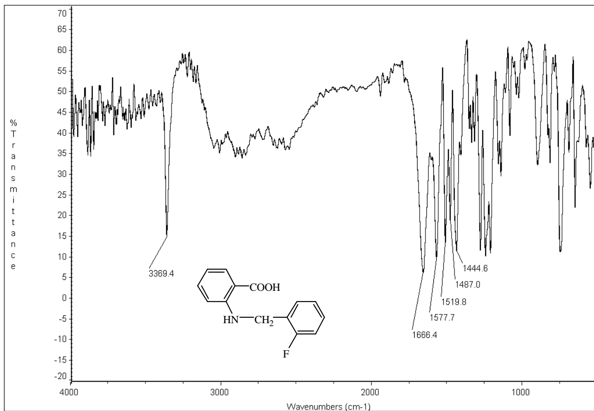
圖 69-2 IR (KBr) spectrum of compound 69
