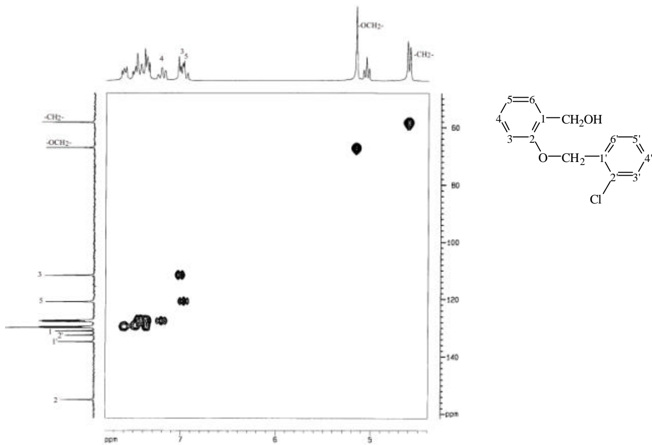
圖 31-6a HMQC (DMSO- d_6 ) spectrum of compound 31
