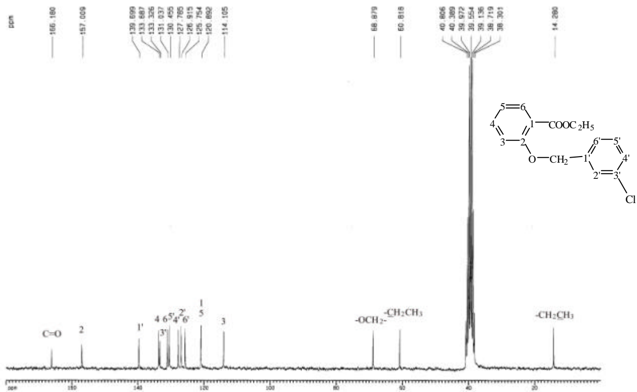
圖 40-4 13 C-NMR (DMSO- d 6 , 50 MHz) spectrum of compound 40
