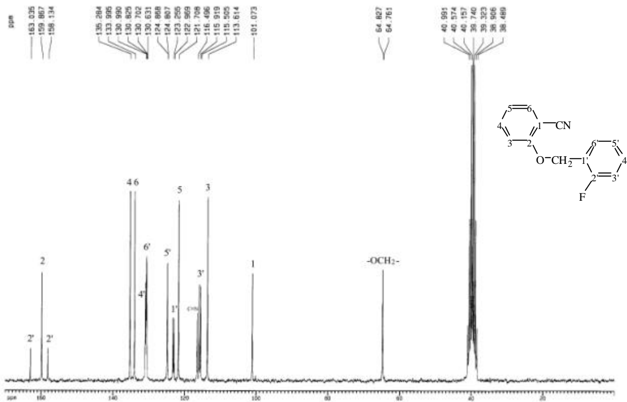
圖 21-4 ^{13}\text{C-NMR} (DMSO- d_6 , 50 MHz) spectrum of compound 21
