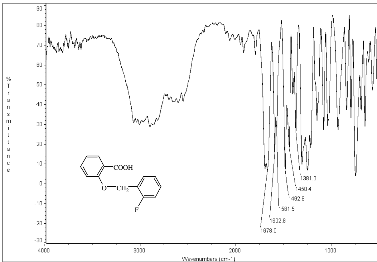
圖 60-2 IR (KBr) spectrum of compound 60
