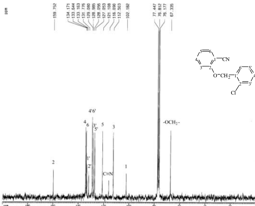
圖 18-4 13 C-NMR (CDCl 3 , 50 MHz) spectrum of compound 18
