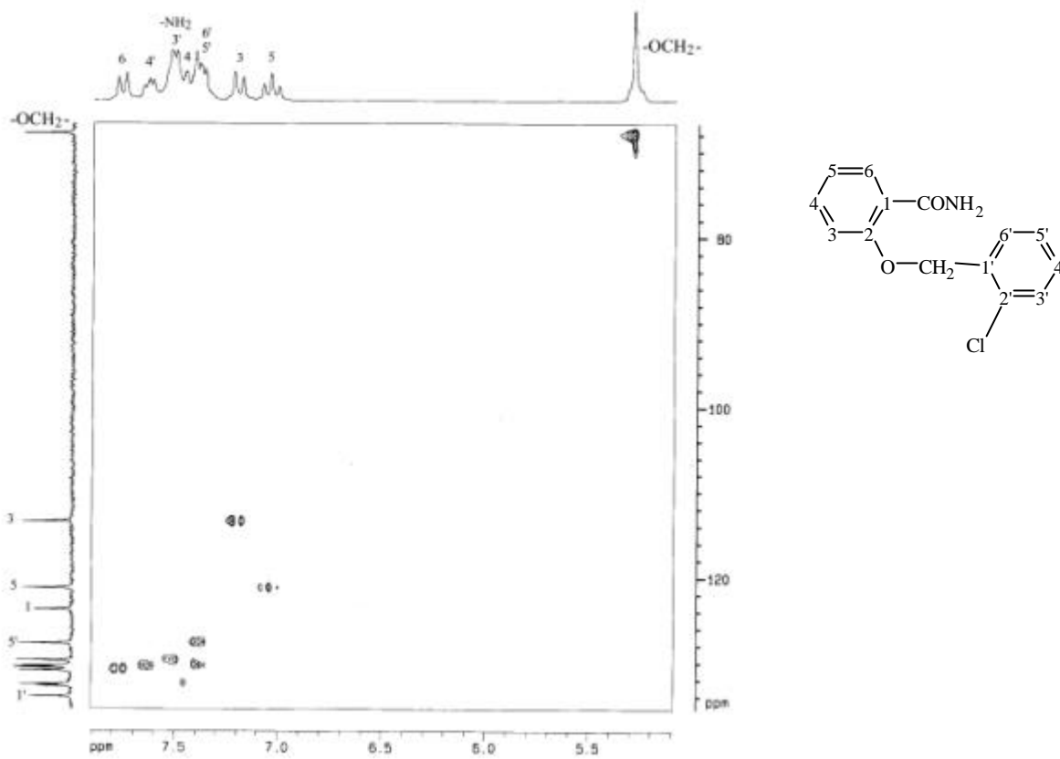
圖 42-6a HMQC (DMSO- d_6 ) spectrum of compound 42
