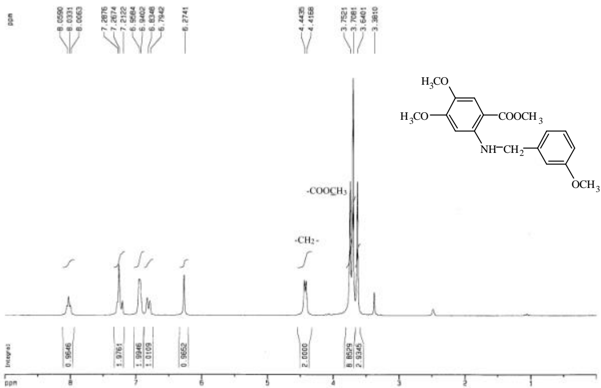
圖 54-1 ^1\text{H-NMR} ( \text{DMSO-}d_6 , 200 MHz) spectrum of compound 54
