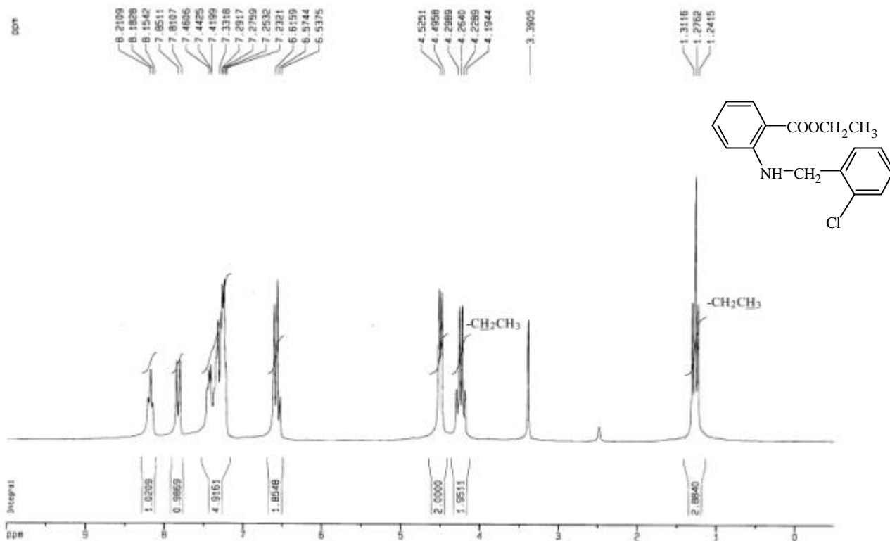
圖 46-1 1 H-NMR (DMSO- d 6 , 200 MHz) spectrum of compound 46
