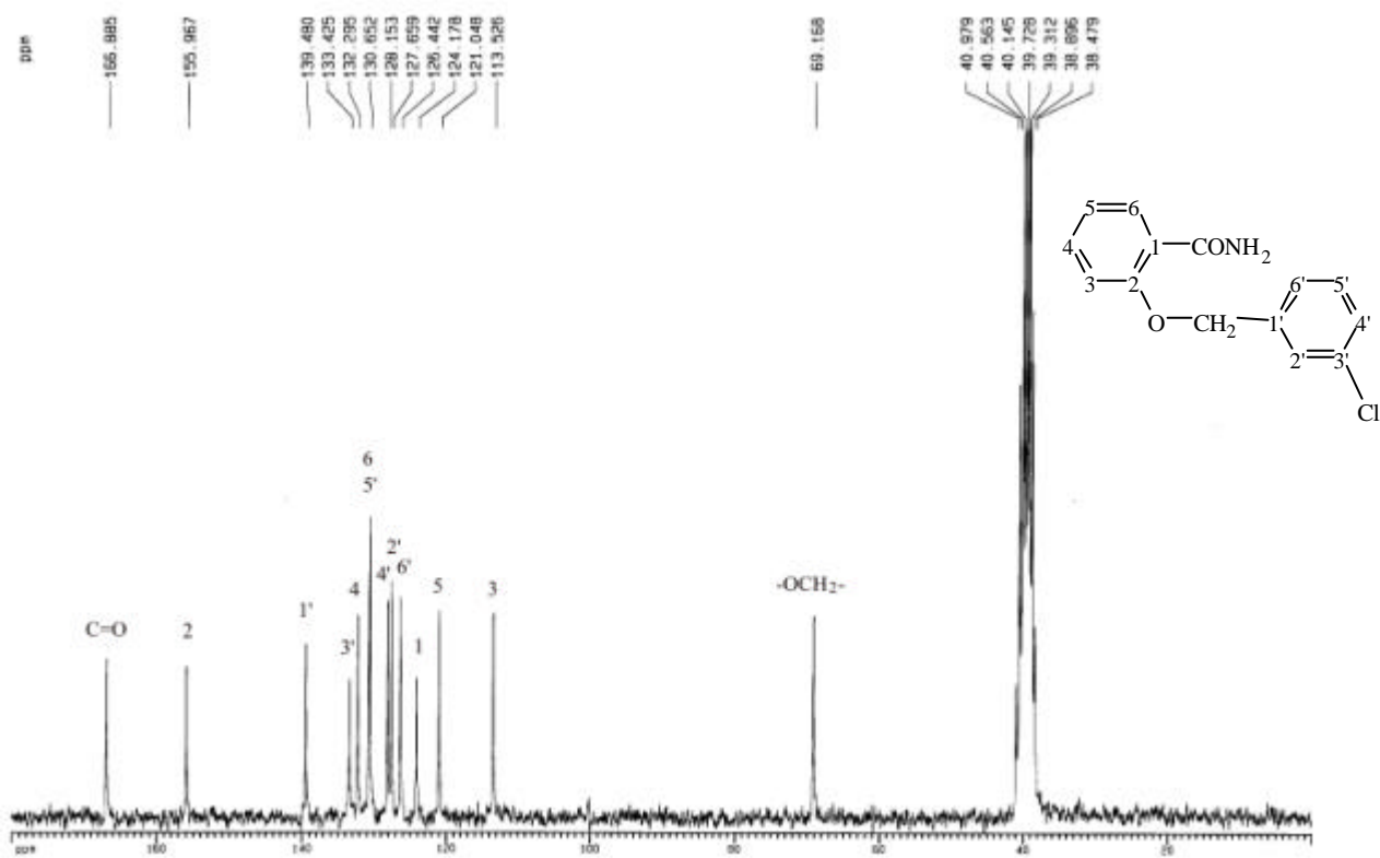
圖 43-4 ^{13}\text{C-NMR} ( \text{DMSO-}d_6 , 50 MHz) spectrum of compound 43
