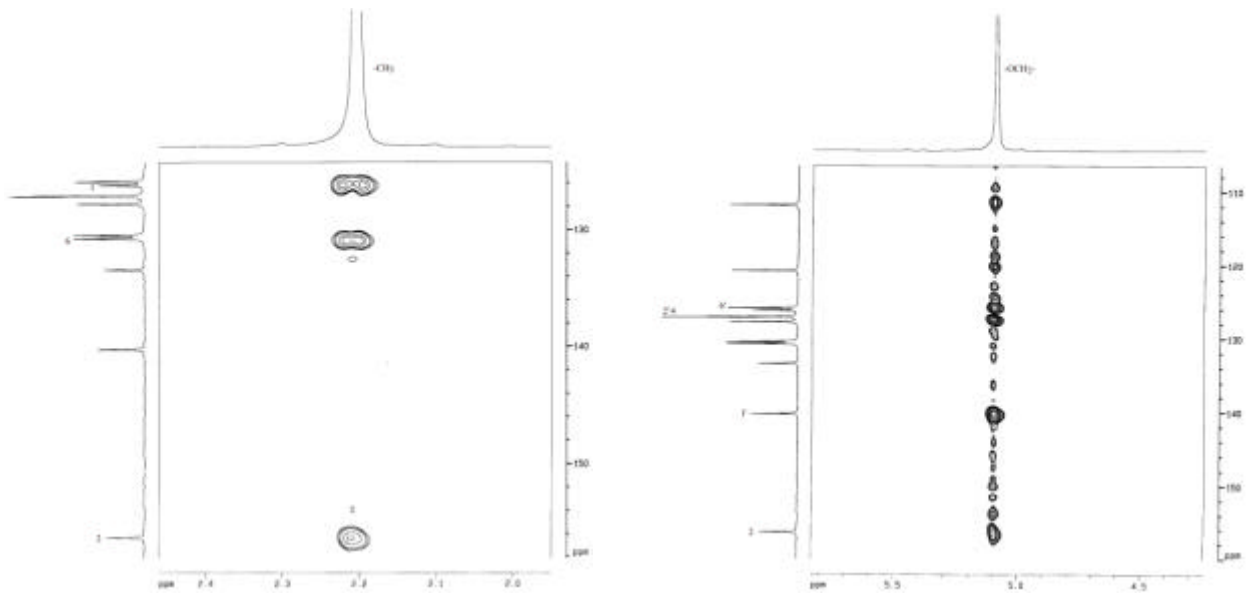
圖 28-5 HMBC (DMSO- d 6 ) spectrum of compound 28
