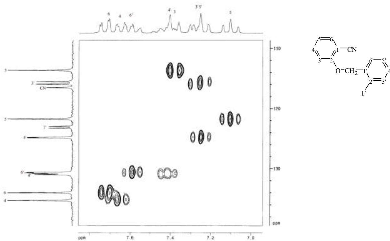
圖 21-6 HMQC (DMSO- d_6 ) spectrum of compound 21
