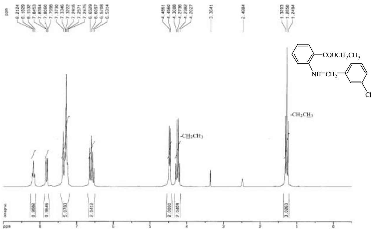
圖 47-1 1 H-NMR (DMSO- d 6 , 200 MHz) spectrum of compound 47
