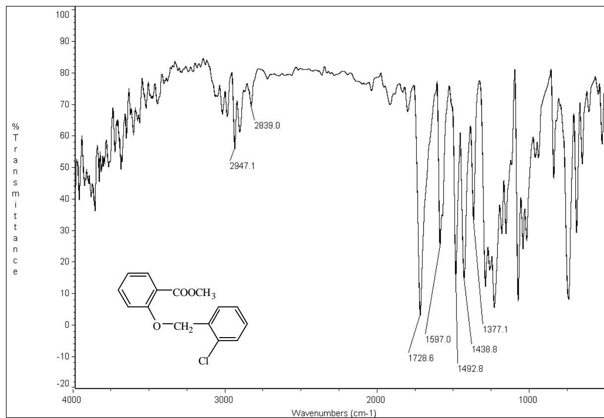
圖 35-2 IR (KBr) spectrum of compound 35
