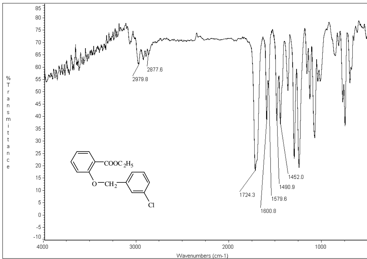
圖 40-2 IR (KBr) spectrum of compound 40
