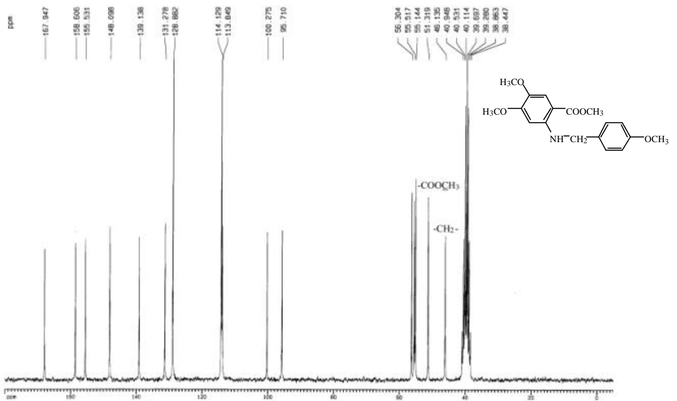
圖 55-2 ^{13}\text{C-NMR} ( \text{DMSO-}d_6 , 50 MHz) spectrum of compound 55
