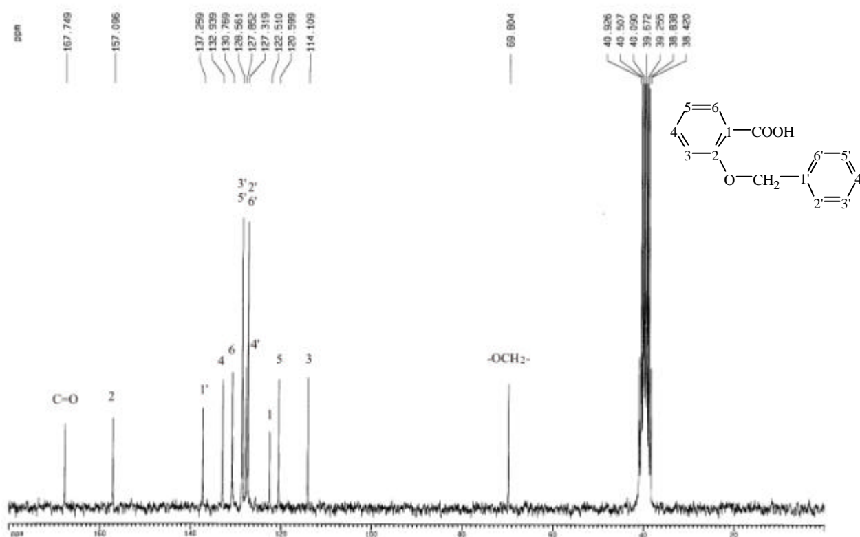
圖 56-4 13 C-NMR (DMSO- d 6 , 50 MHz) spectrum of compound 56
