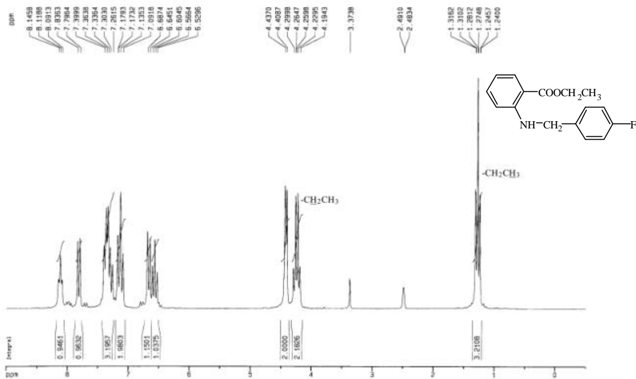
圖 51-1 ^1\text{H-NMR} (DMSO- d_6 , 200 MHz) spectrum of compound 51
