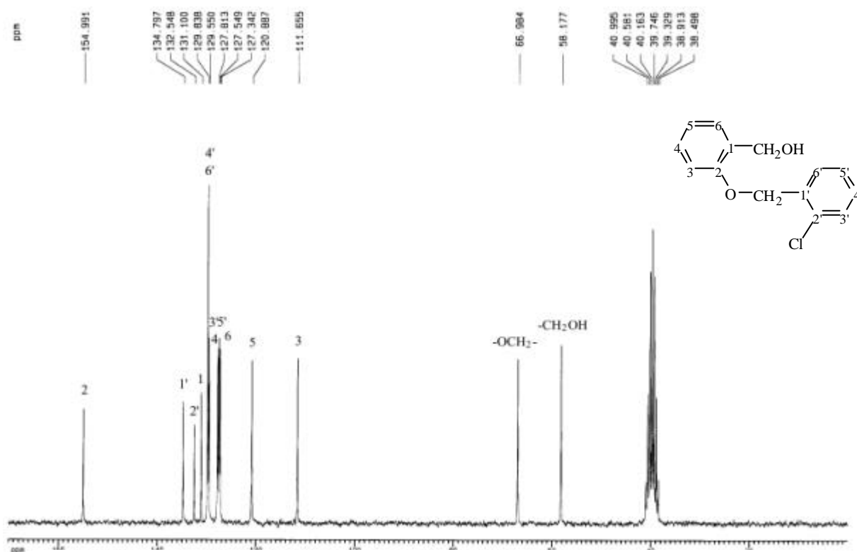
圖 31-4 13 C-NMR (DMSO- d 6 , 50 MHz) spectrum of compound 31
