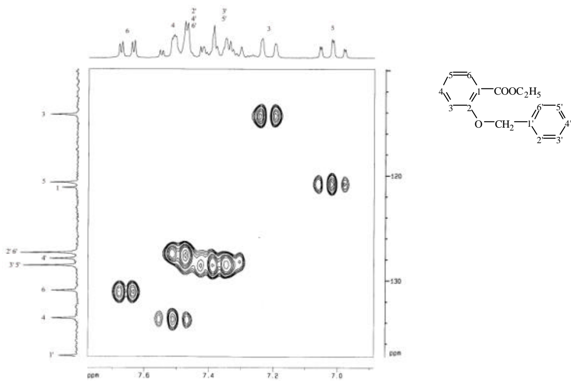
圖 38-6b HMQC (DMSO- d_6 ) spectrum of compound 38
