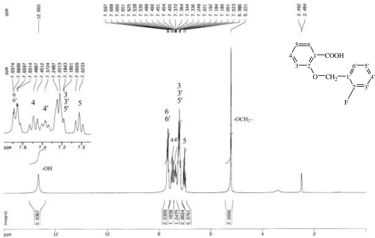
圖 60-3 1 H-NMR (DMSO- d 6 , 200 MHz) spectrum of compound 60
