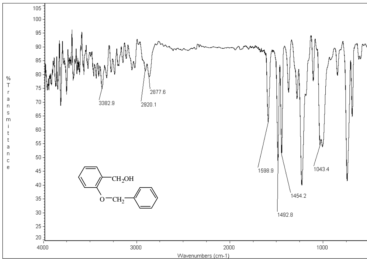
圖 30-2 IR (KBr) spectrum of compound 30
