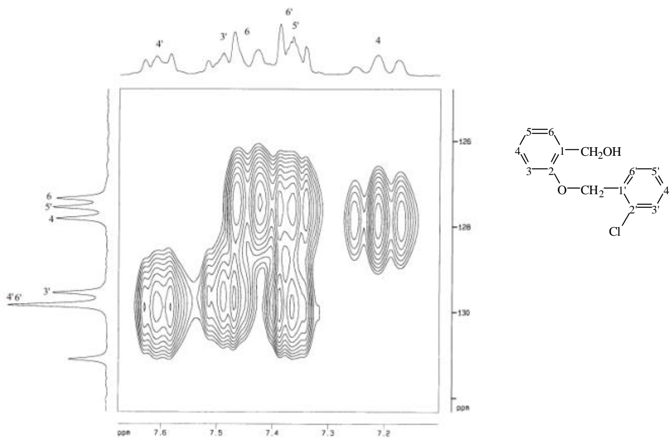
圖 31-6b HMQC (DMSO- d_6 ) spectrum of compound 31
