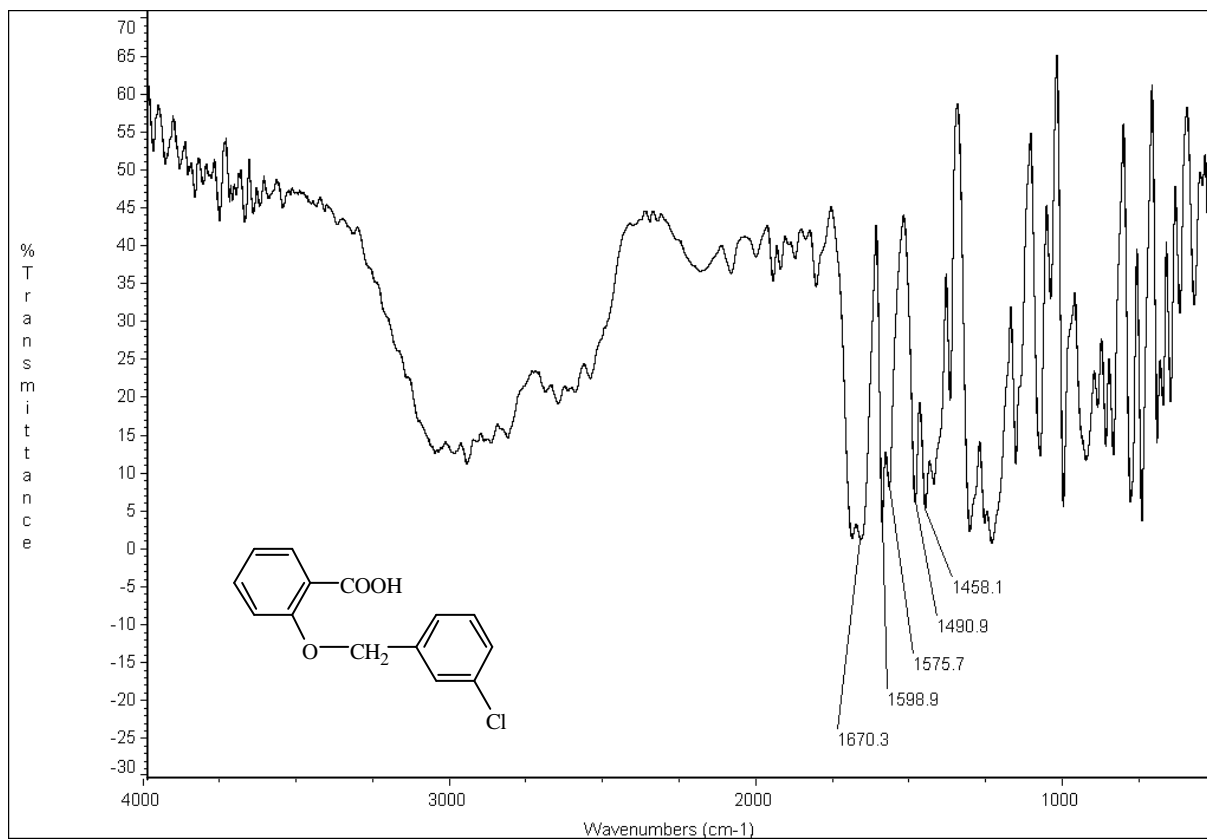
圖 58-2 IR (KBr) spectrum of compound 58
