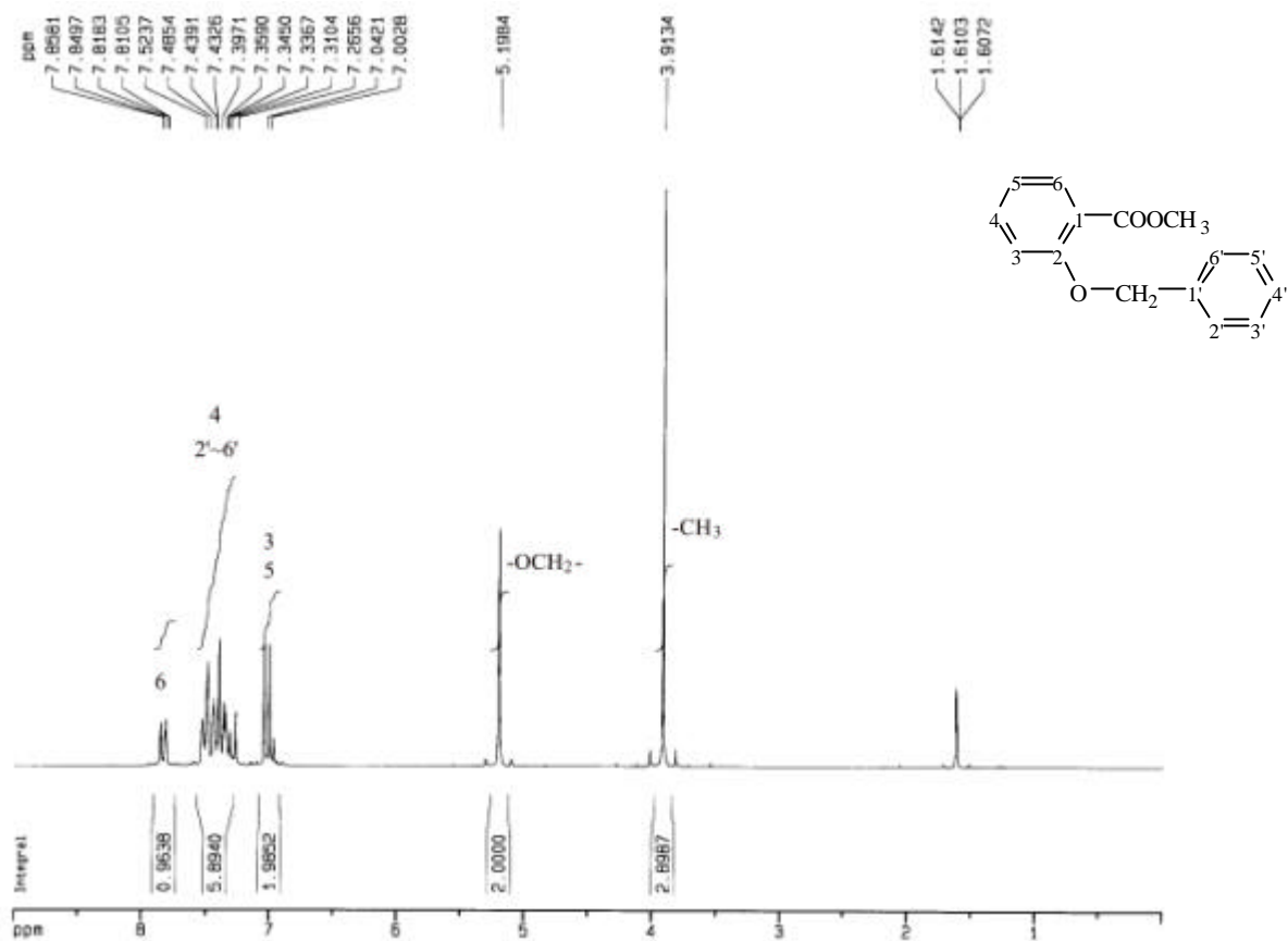
圖 34-3 1 H-NMR (CDCl 3 , 200 MHz) spectrum of compound 34
