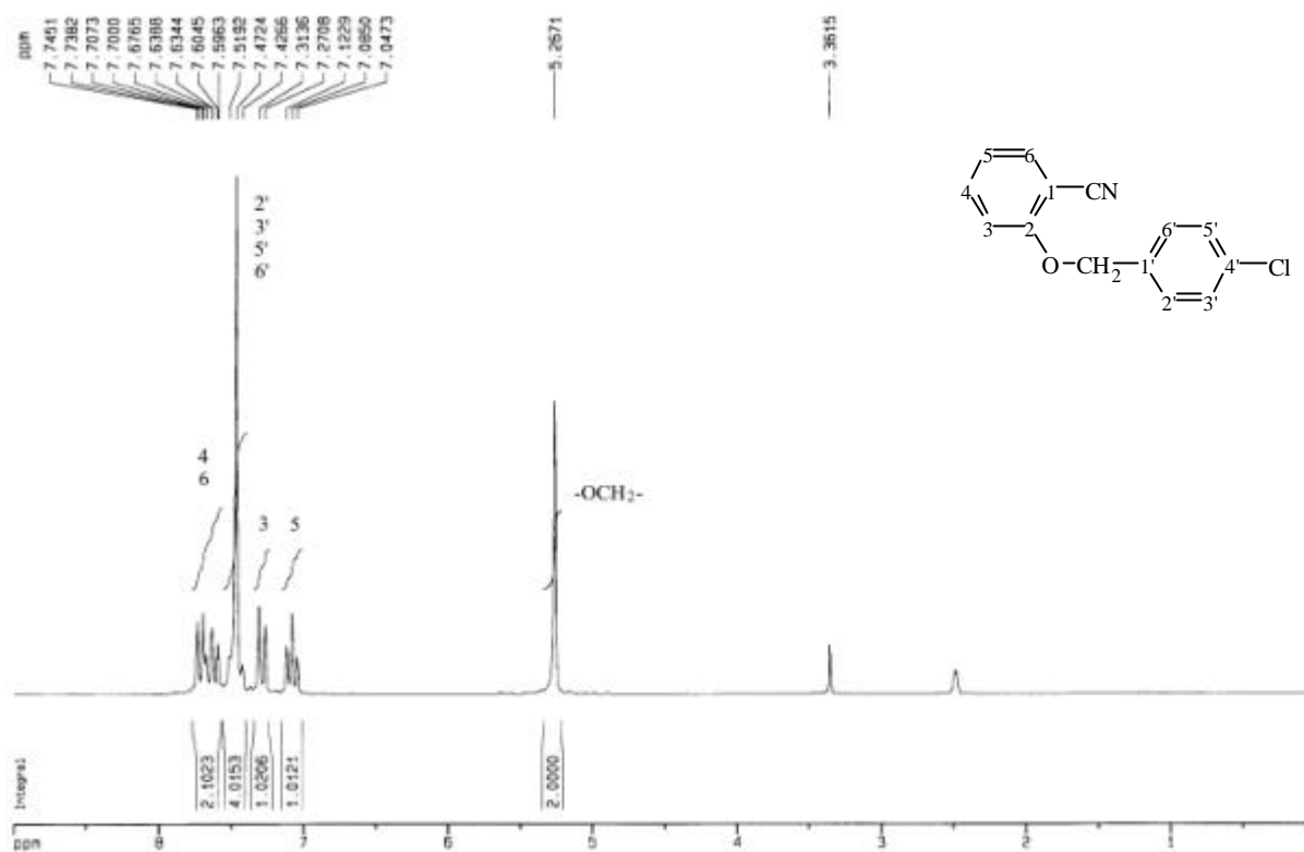
圖 20-3 ^1\text{H-NMR} (CDCl 3 , 200 MHz) spectrum of compound 20
