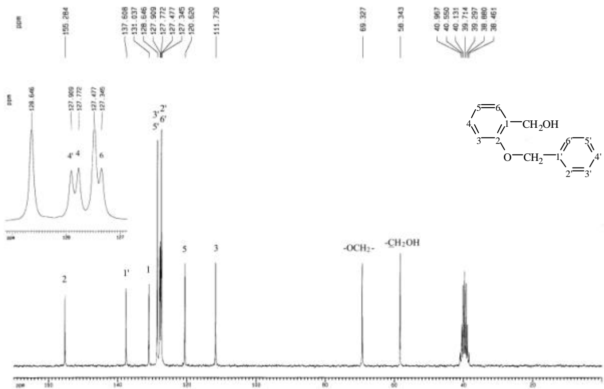
圖 30-4 ^{13}\text{C-NMR} (DMSO- d_6 , 50 MHz) spectrum of compound 30
