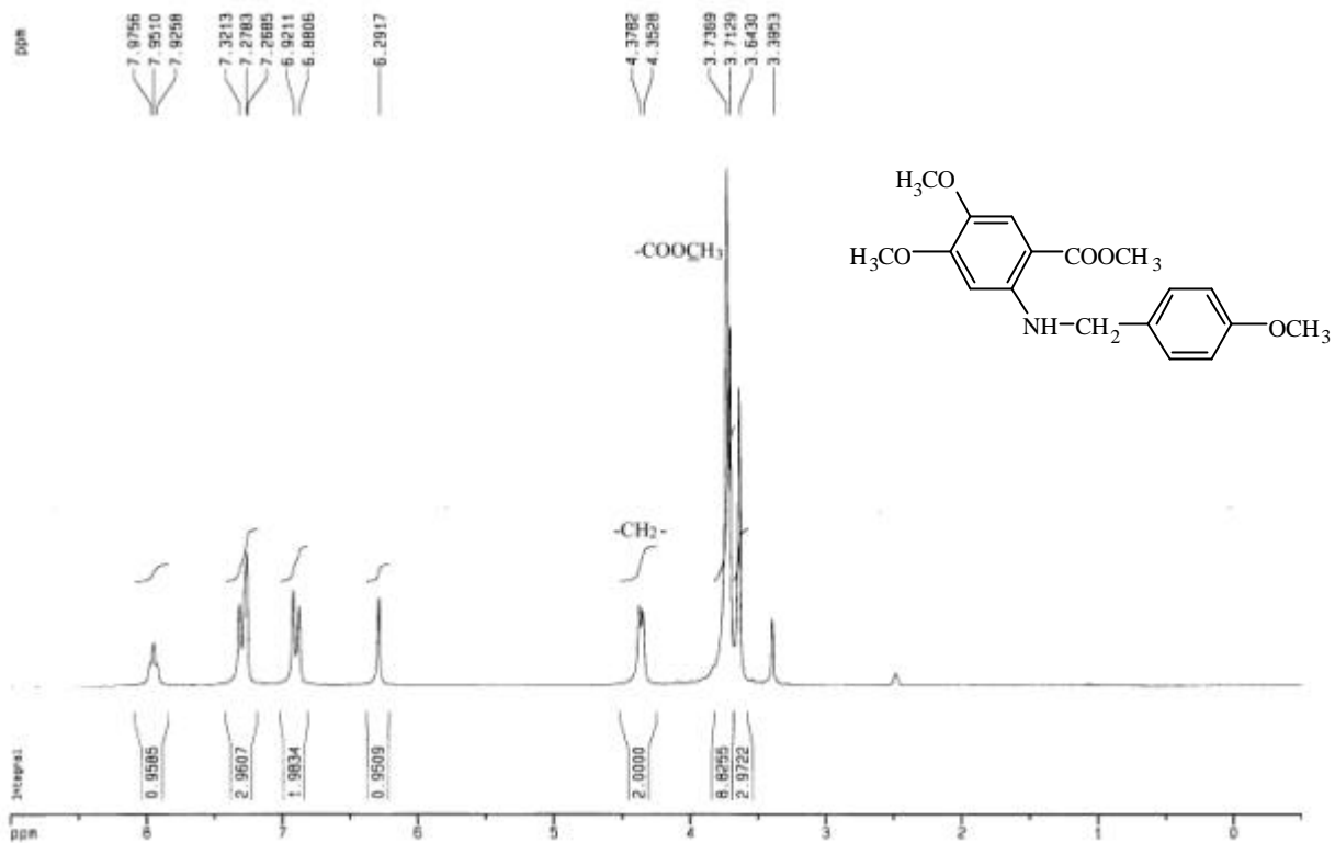
圖 55-1 ^1\text{H-NMR} ( \text{DMSO-}d_6 , 200 MHz) spectrum of compound 55
