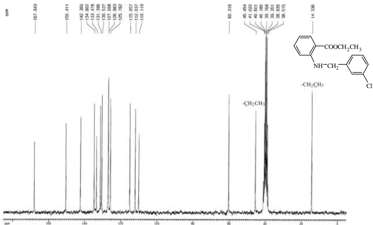
圖 47-2 13 C-NMR (DMSO- d 6 , 50 MHz) spectrum of compound 47
