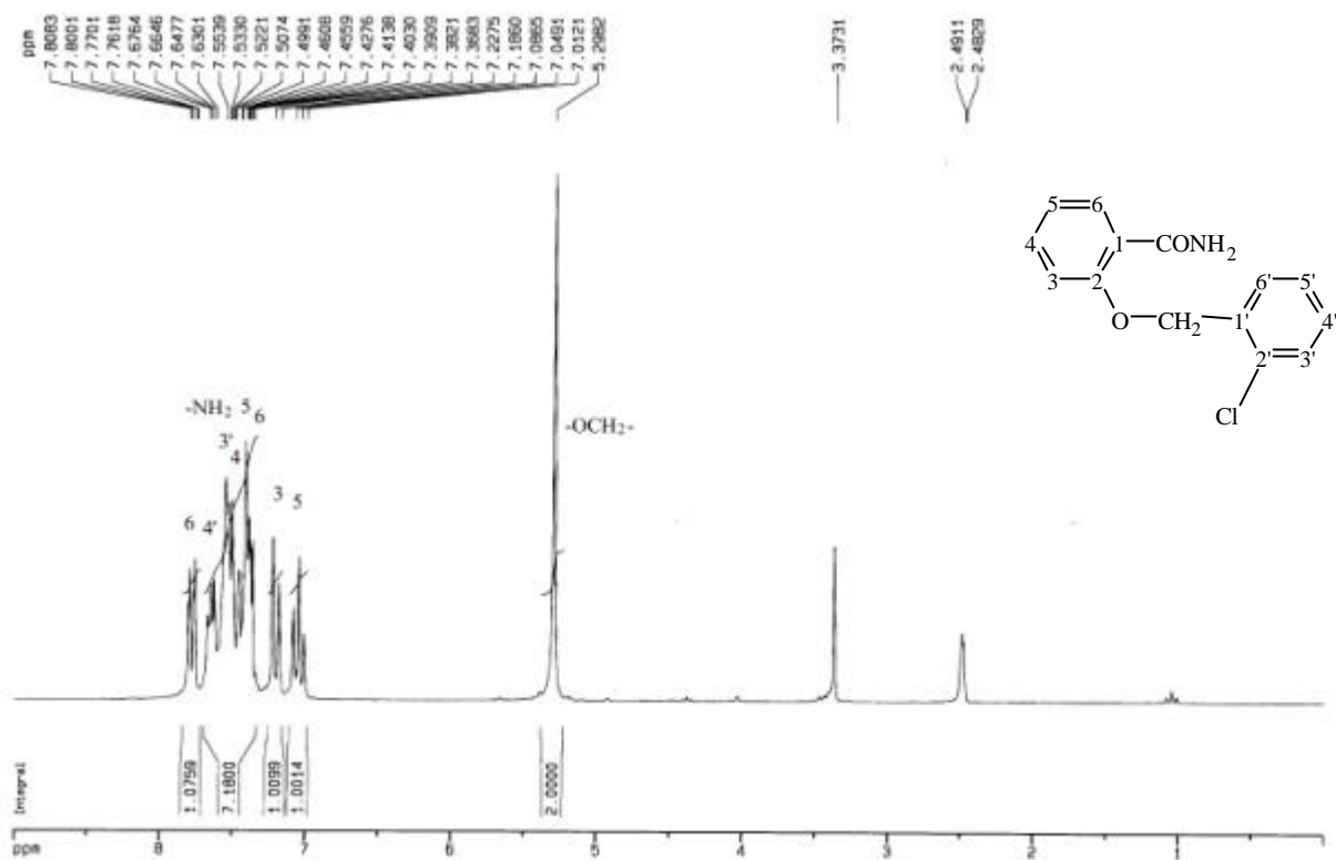
圖 42-3 ^1\text{H-NMR} (DMSO- d_6 , 200 MHz) spectrum of compound 42
