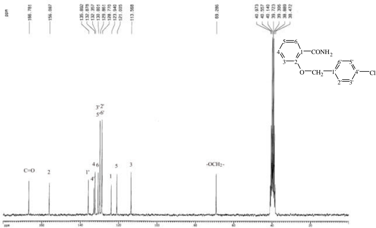
圖 44-4 ^{13}\text{C-NMR} ( \text{DMSO-}d_6 , 50 MHz) spectrum of compound 44
