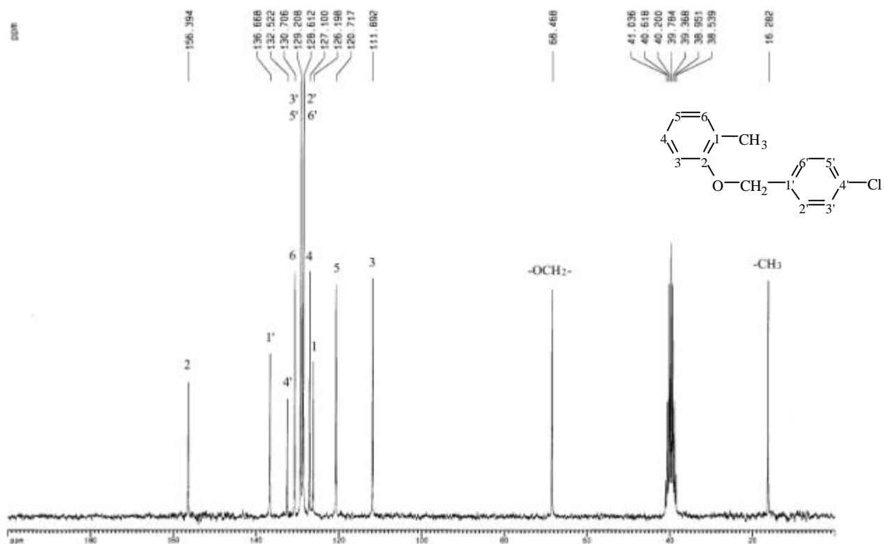
圖 29-4 ^{13}\text{C-NMR} (DMSO- d_6 , 50 MHz) spectrum of compound 29
