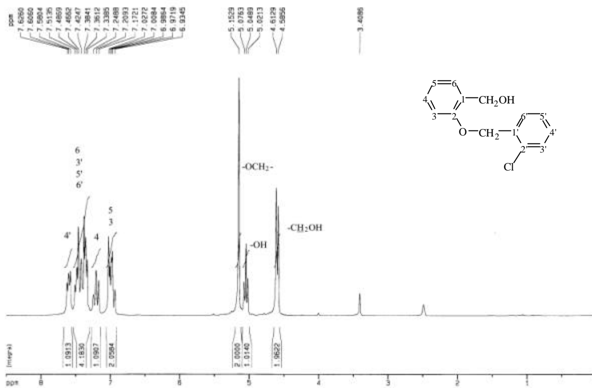
圖 31-3 1 H-NMR (DMSO- d 6 , 200 MHz) spectrum of compound 31
