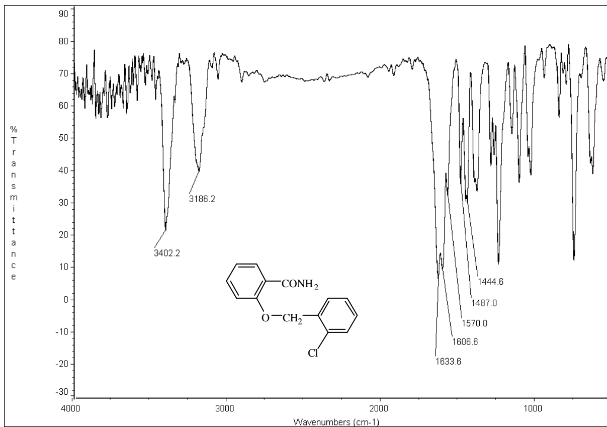
圖 42-2 IR (KBr) spectrum of compound 42
