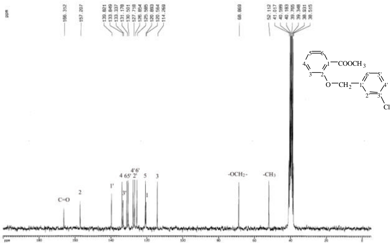
圖 36-4 13 C-NMR (DMSO- d 6 , 50 MHz) spectrum of compound 36
