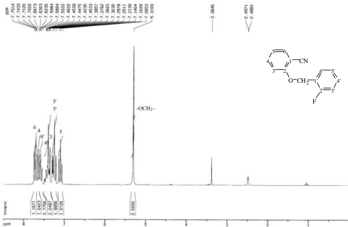
圖 21-3 ^1\text{H-NMR} (DMSO- d_6 , 200 MHz) spectrum of compound 21
