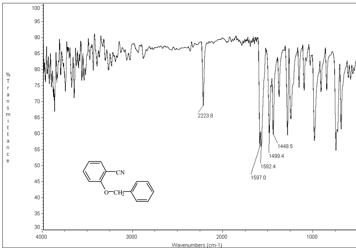
圖 17-2 IR (KBr) spectrum of compound 17
