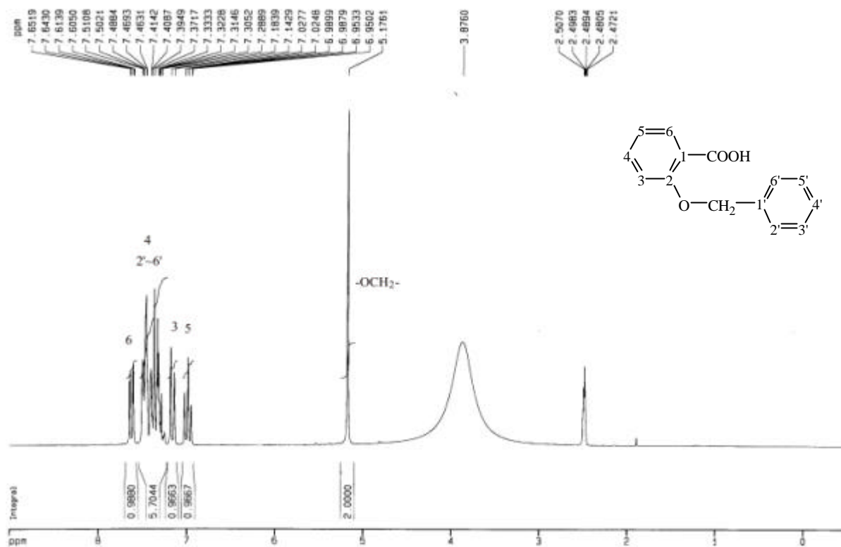
圖 56-3 1 H-NMR (DMSO- d 6 , 200 MHz) spectrum of compound 56
