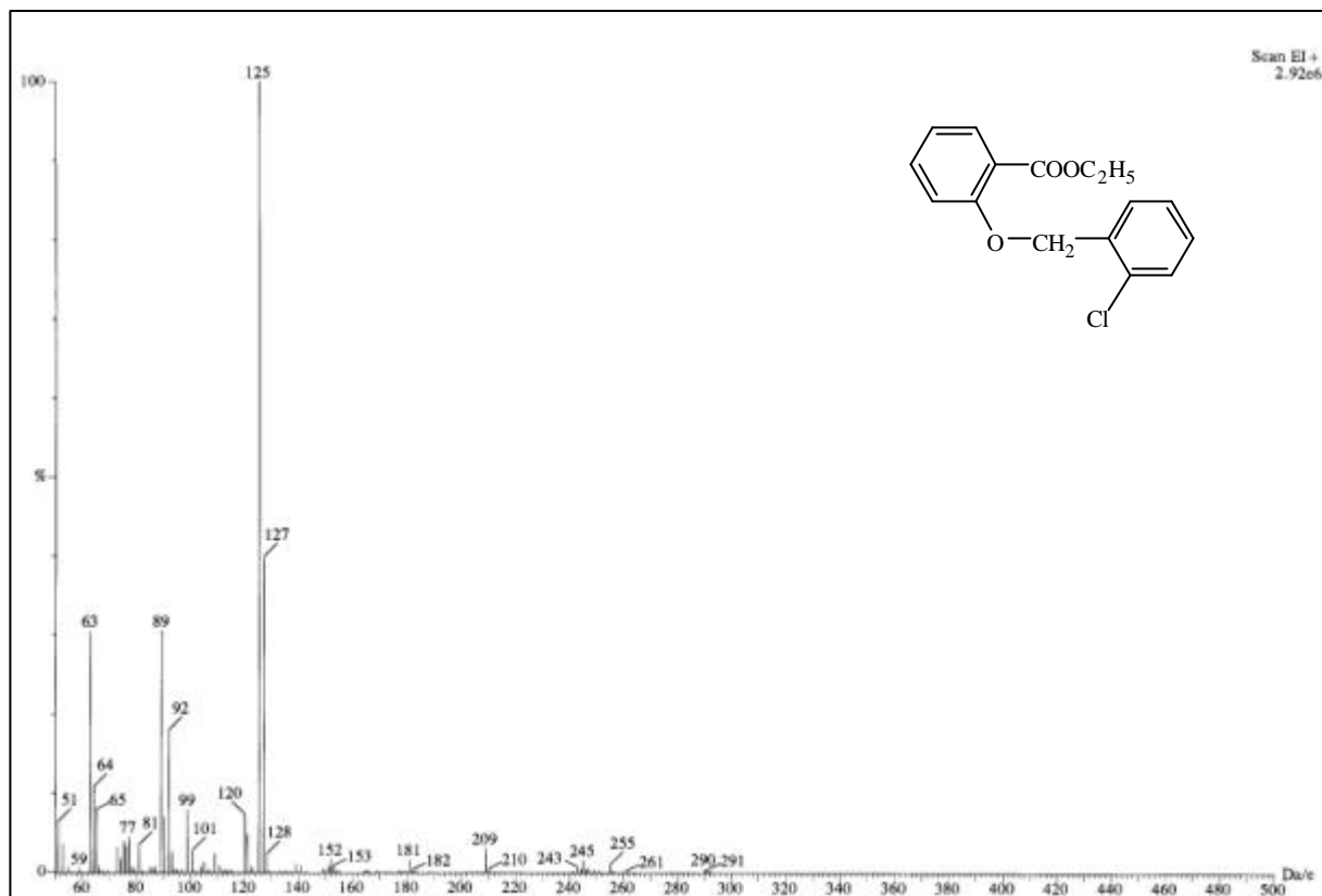
圖 39-1 MS spectrum of compound 39
