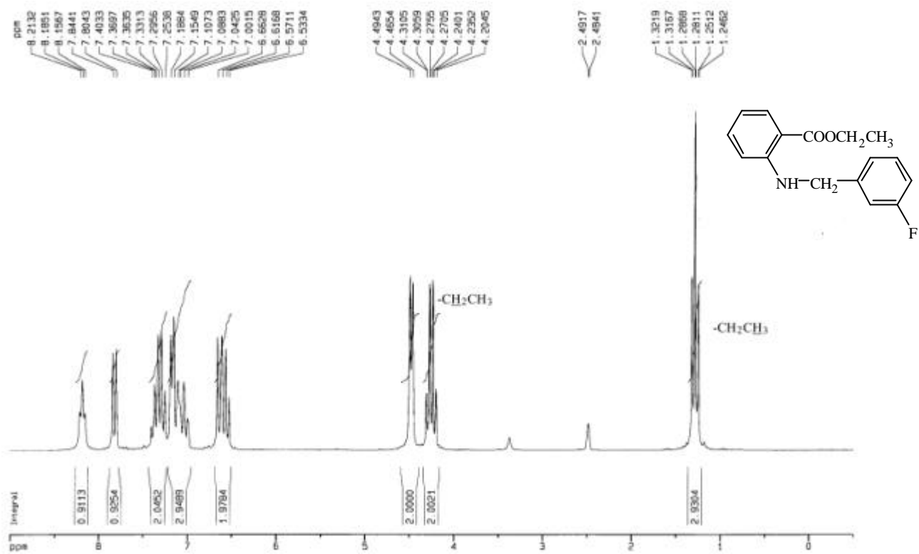
圖 50-1 1 H-NMR (DMSO- d 6 , 200 MHz) spectrum of compound 50
