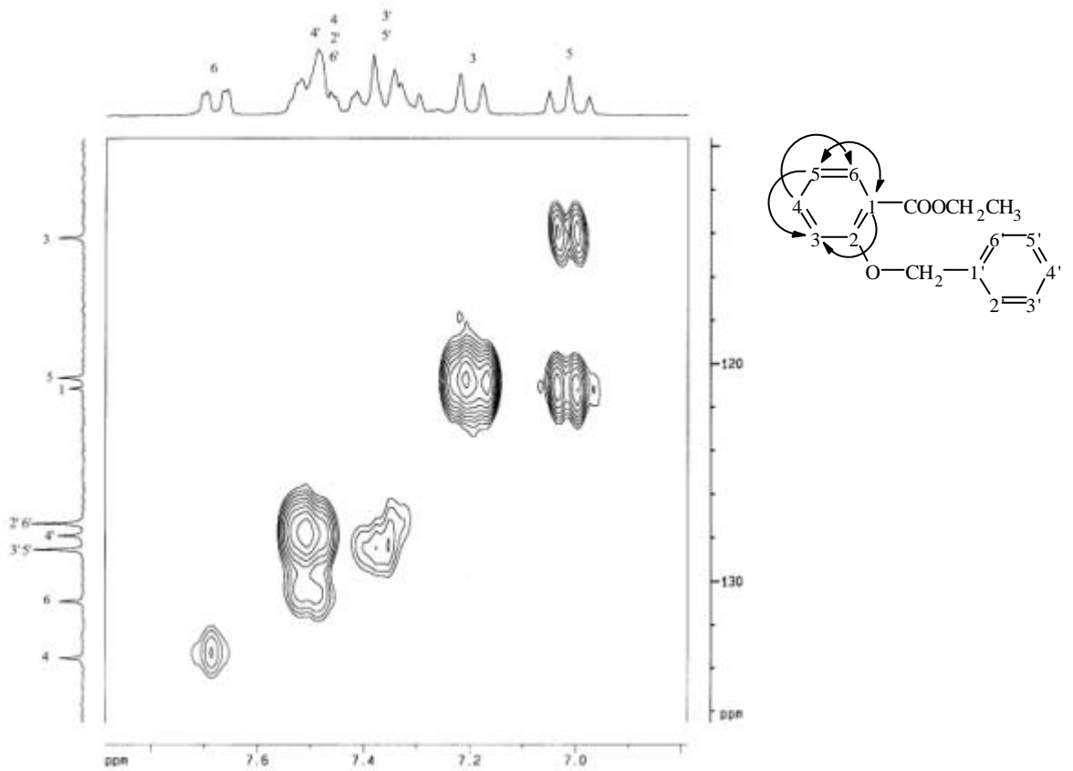
圖 38-5b HMBC (DMSO- d_6 ) spectrum of compound 38
