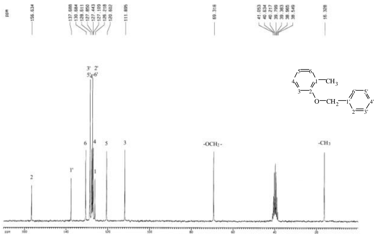
圖 26-4 ^{13}\text{C-NMR} ( \text{DMSO-}d_6 , 50 MHz) spectrum of compound 26
