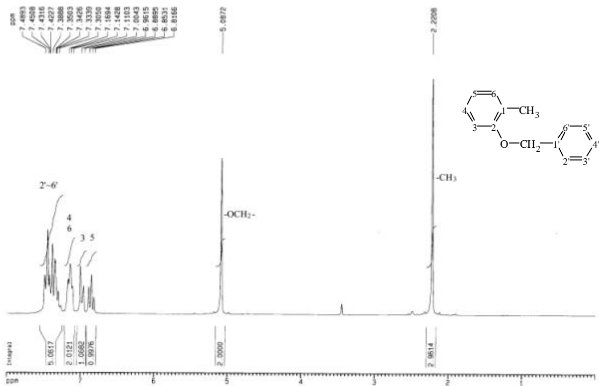
圖 26-3 ^1\text{H-NMR} ( \text{DMSO-}d_6 , 200 MHz) spectrum of compound 26
