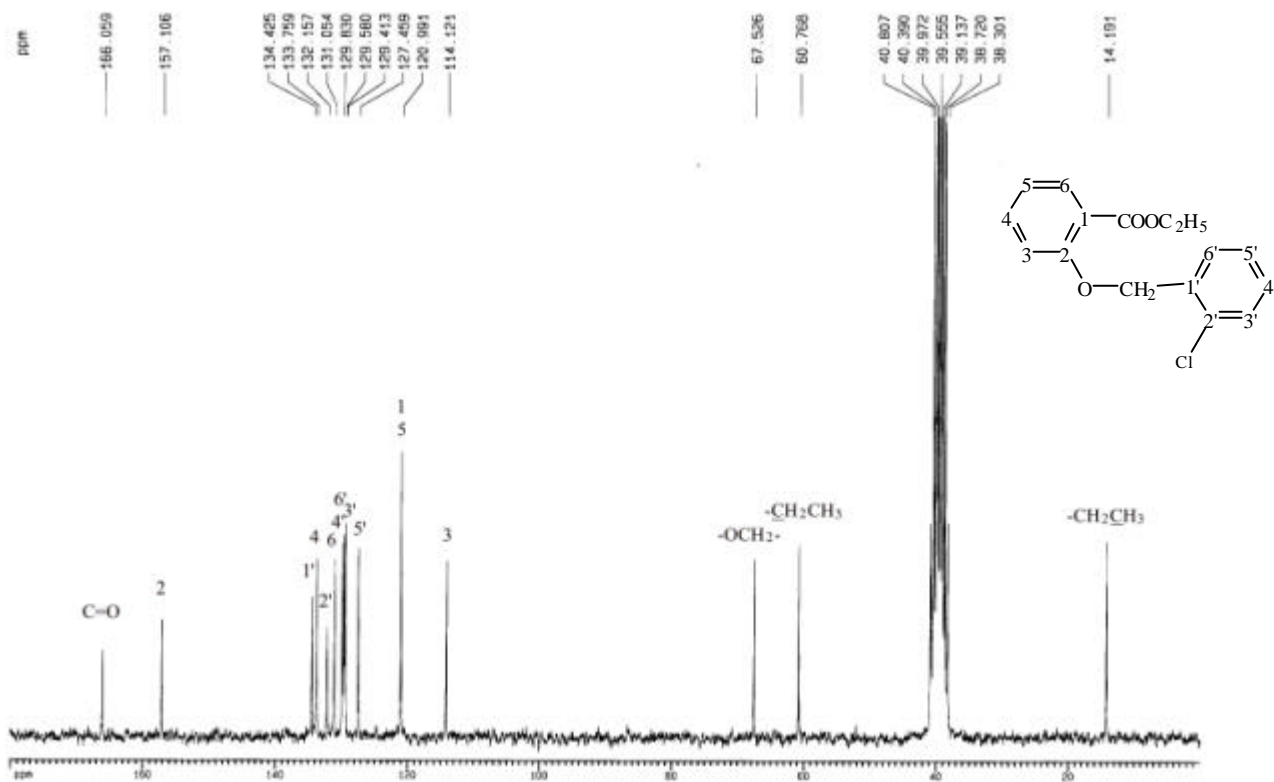
圖 39-4 13 C-NMR (DMSO- d 6 , 50 MHz) spectrum of compound 39
