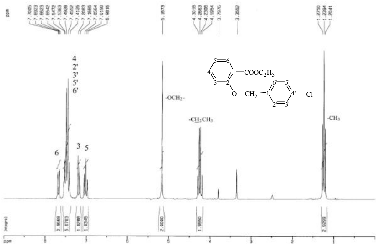
圖 41-3 ^1\text{H-NMR} ( \text{DMSO-}d_6 , 200 MHz) spectrum of compound 41
