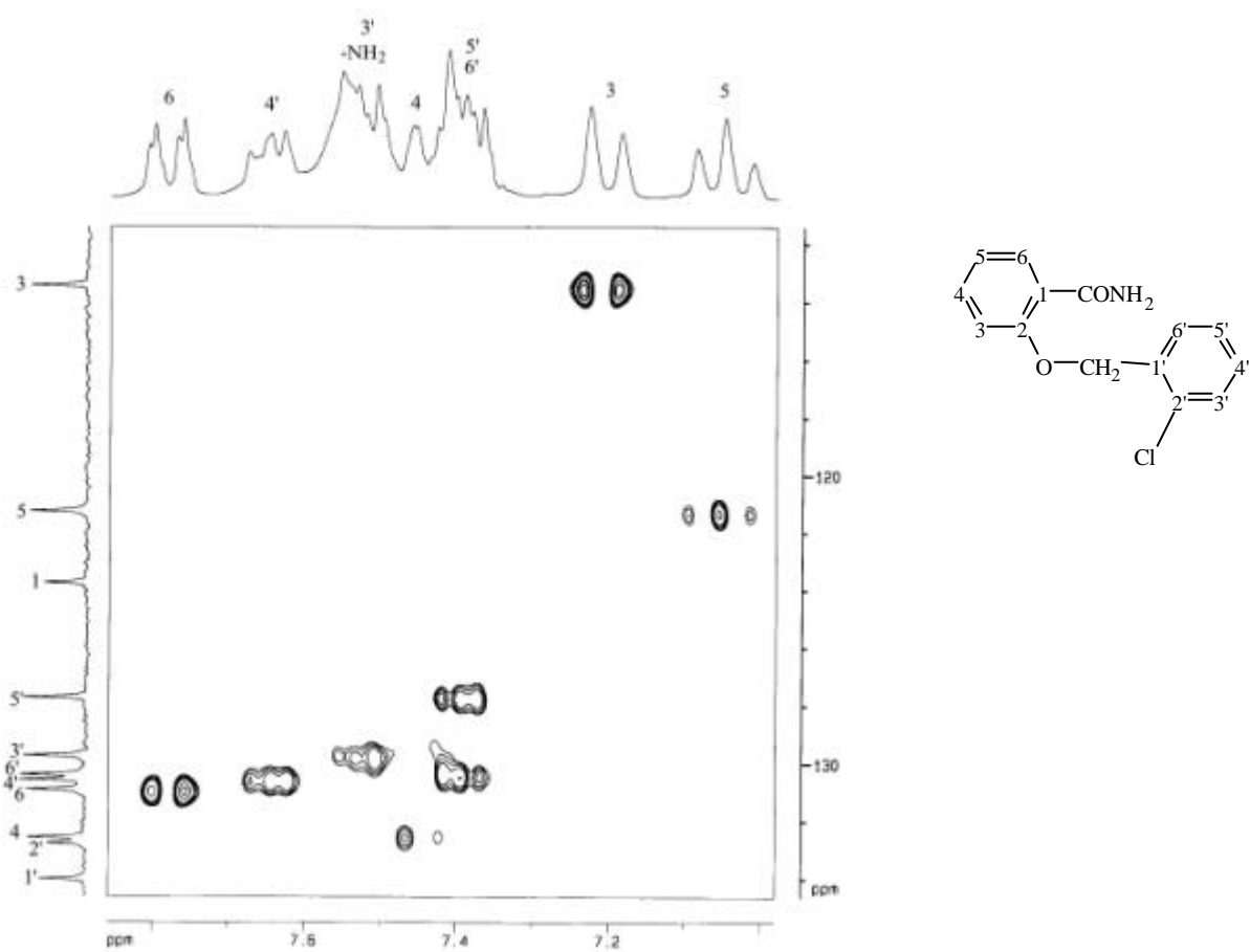
圖 42-6b HMQC (DMSO- d_6 ) spectrum of compound 42
