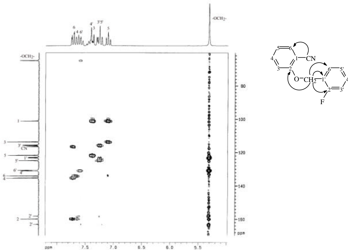
圖 21-5 HMBC (DMSO- d_6 ) spectrum of compound 21
