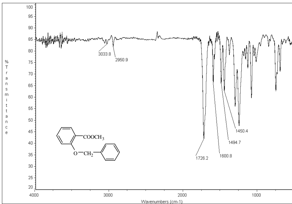
圖 34-2 IR (KBr) spectrum of compound 34
