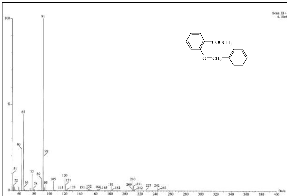
圖 34-1 MS spectrum of compound 34
