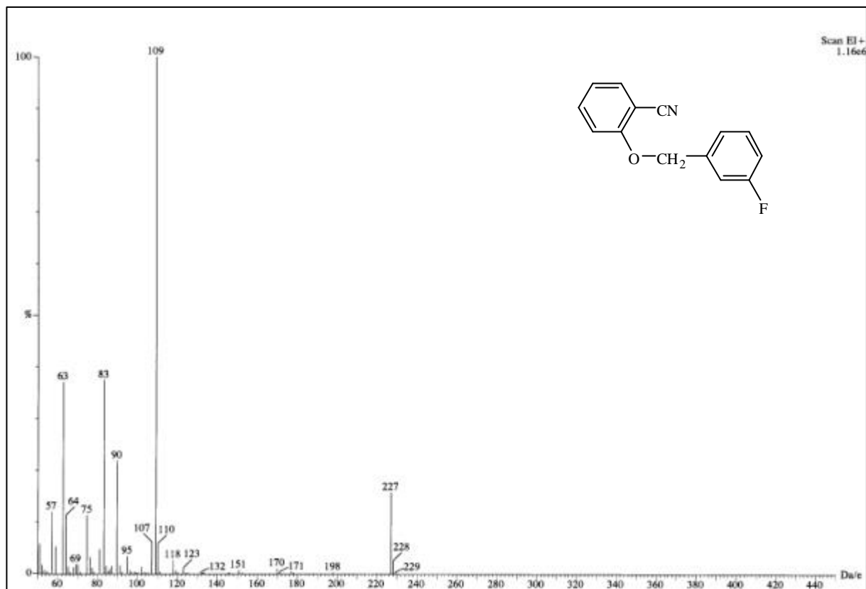
圖 22-1 MS spectrum of compound 22
