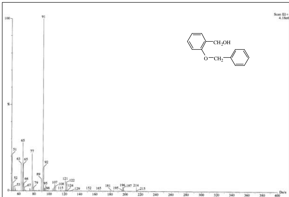
圖 30-1 MS spectrum of compound 30
