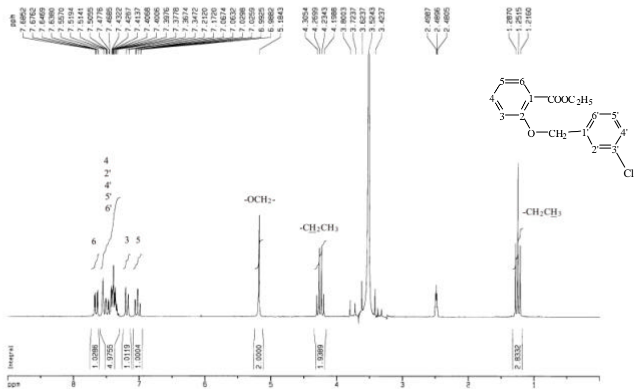
圖 40-3 1 H-NMR (DMSO- d 6 , 200 MHz) spectrum of compound 40
