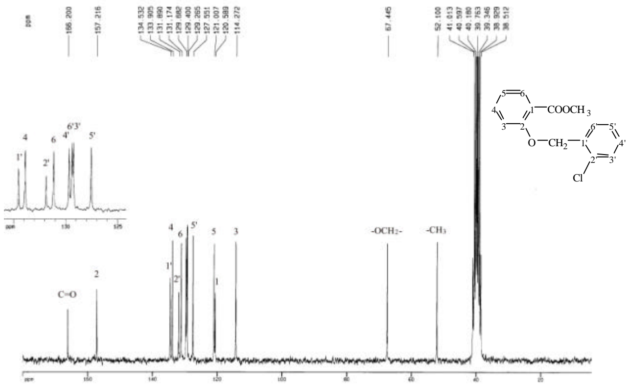
圖 35-4 13 C-NMR (DMSO- d 6 , 50 MHz) spectrum of compound 35
