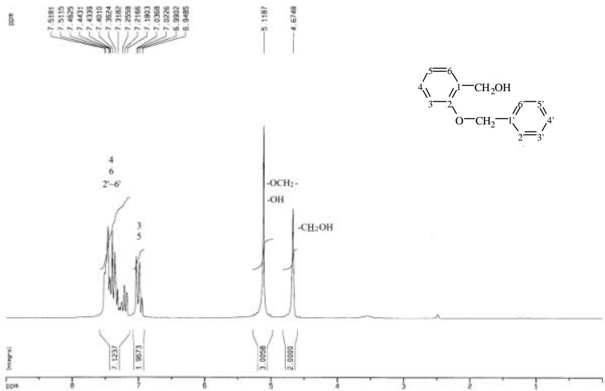
圖 30-3 ^1\text{H-NMR} (DMSO- d_6 , 200 MHz) spectrum of compound 30
