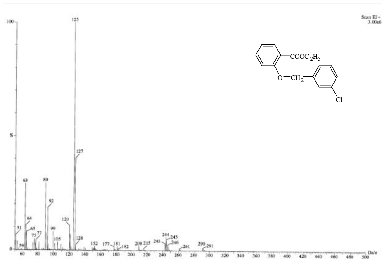
圖 40-1 MS spectrum of compound 40
