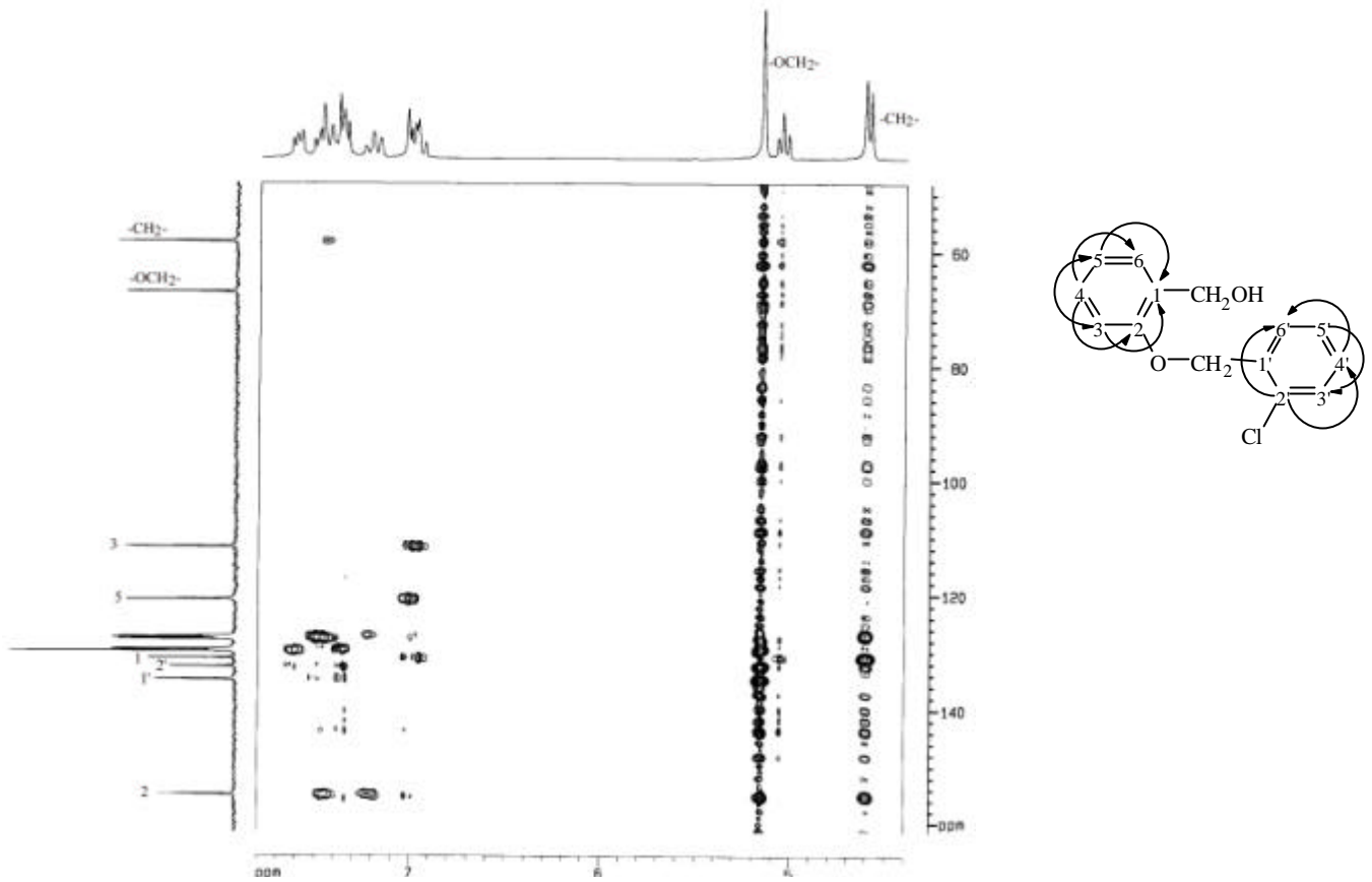
圖 31-5a HMBC (DMSO- d_6 ) spectrum of compound 31
