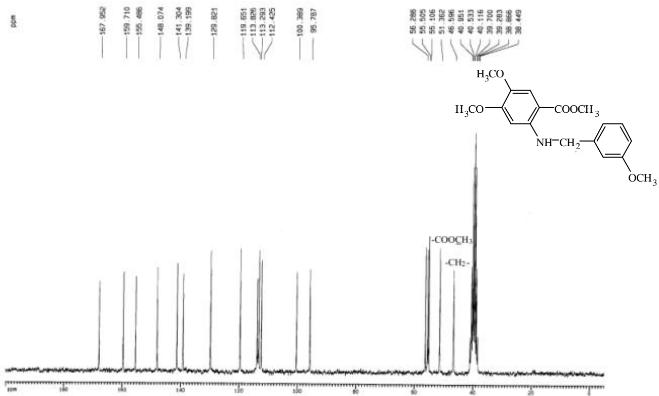
圖 54-2 ^{13}\text{C-NMR} ( \text{DMSO-}d_6 , 50 MHz) spectrum of compound 54
