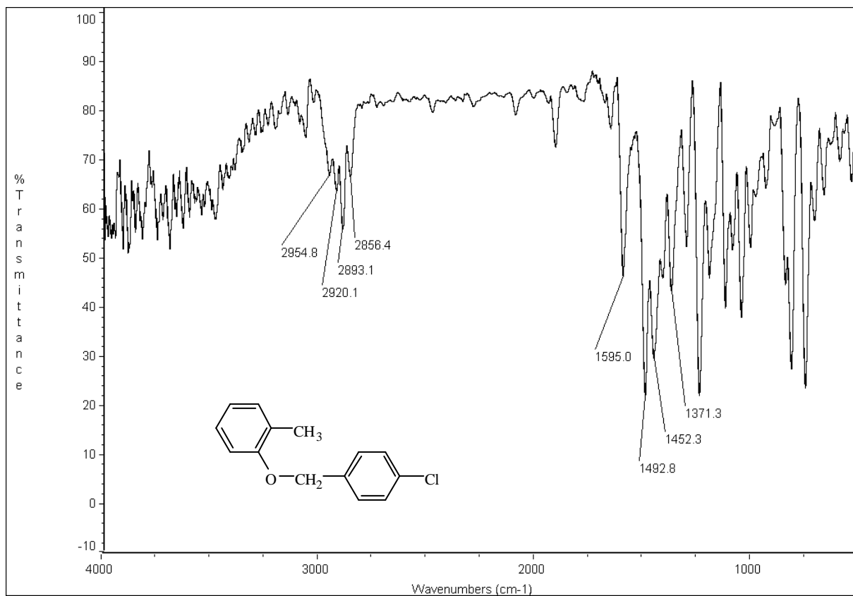
圖 29-2 IR (KBr) spectrum of compound 29
