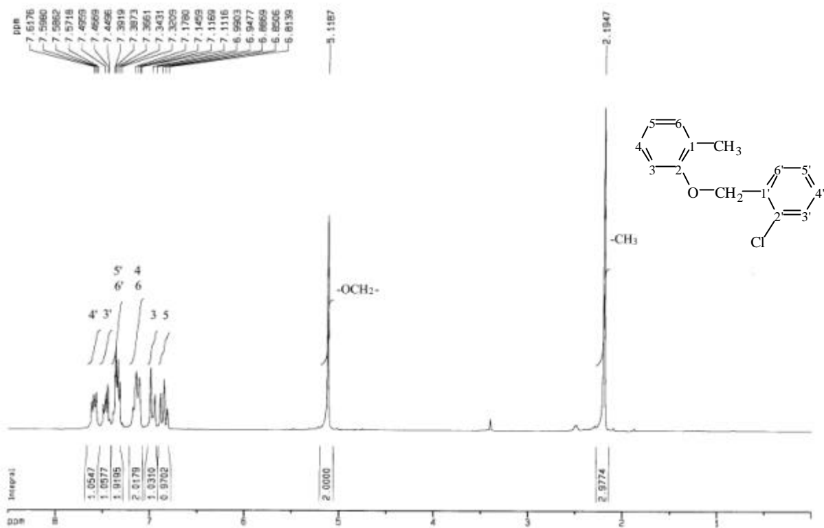
圖 27-3 1 H-NMR (DMSO- d 6 , 200 MHz) spectrum of compound 27
