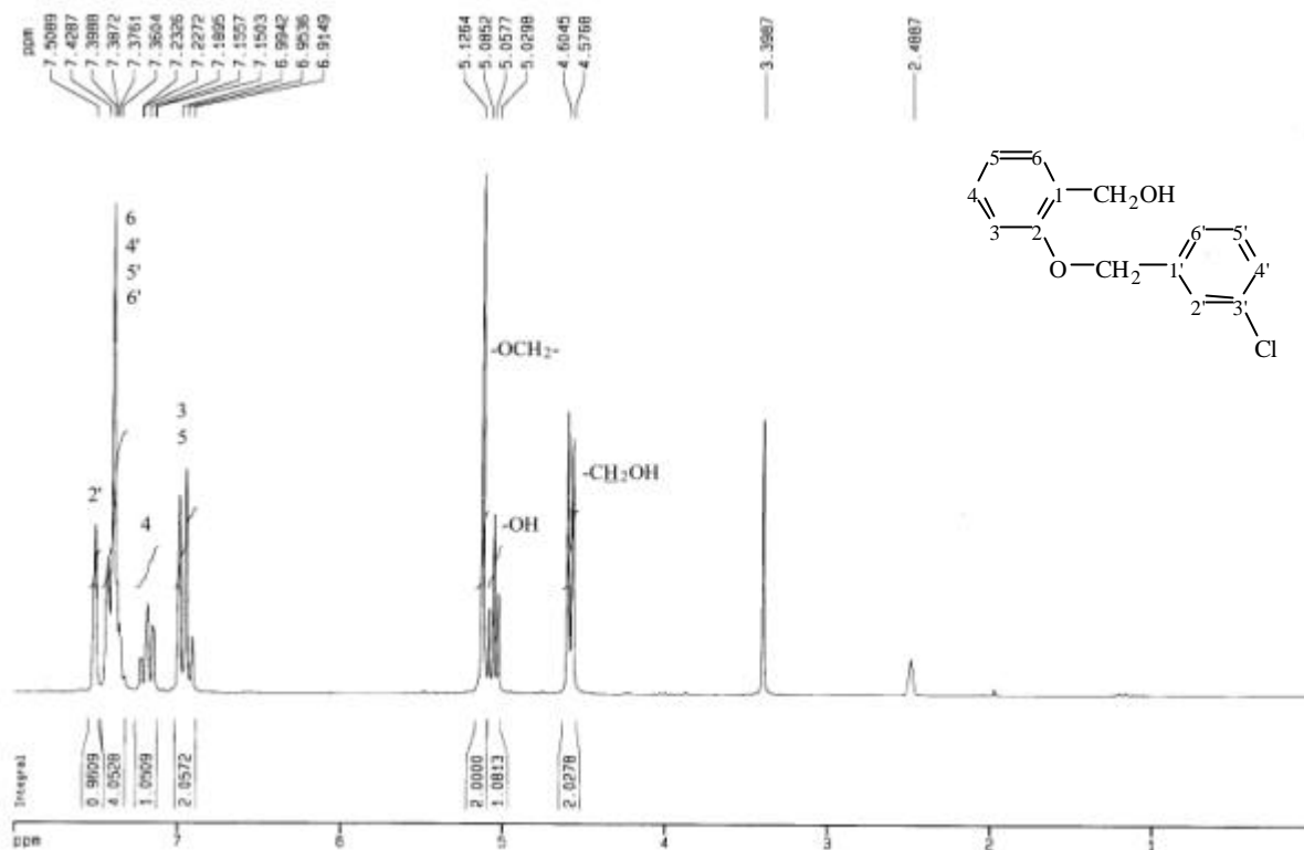
圖 32-3 1 H-NMR (DMSO- d 6 , 200 MHz) spectrum of compound 32
