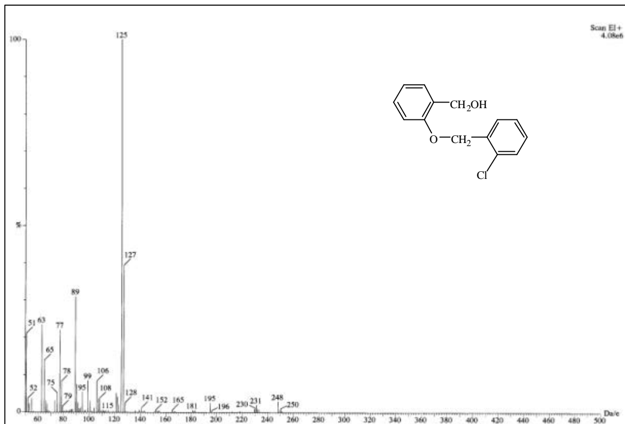
圖 31-1 MS spectrum of compound 31
