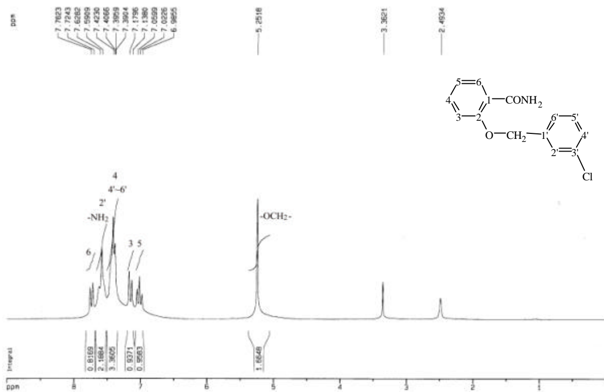
圖 43-3 ^1\text{H-NMR} ( \text{DMSO-}d_6 , 200 MHz) spectrum of compound 43
