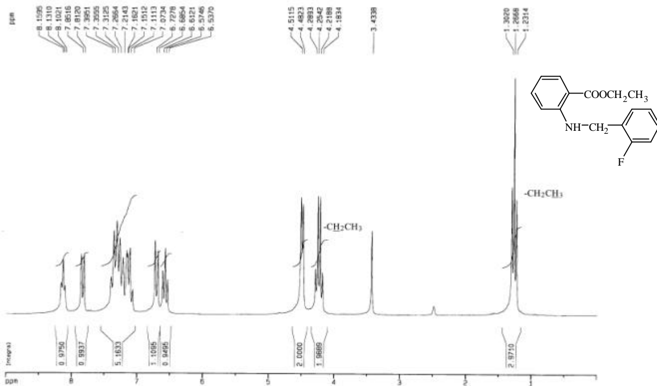
圖 49-1 1 H-NMR (DMSO- d 6 , 200 MHz) spectrum of compound 49
