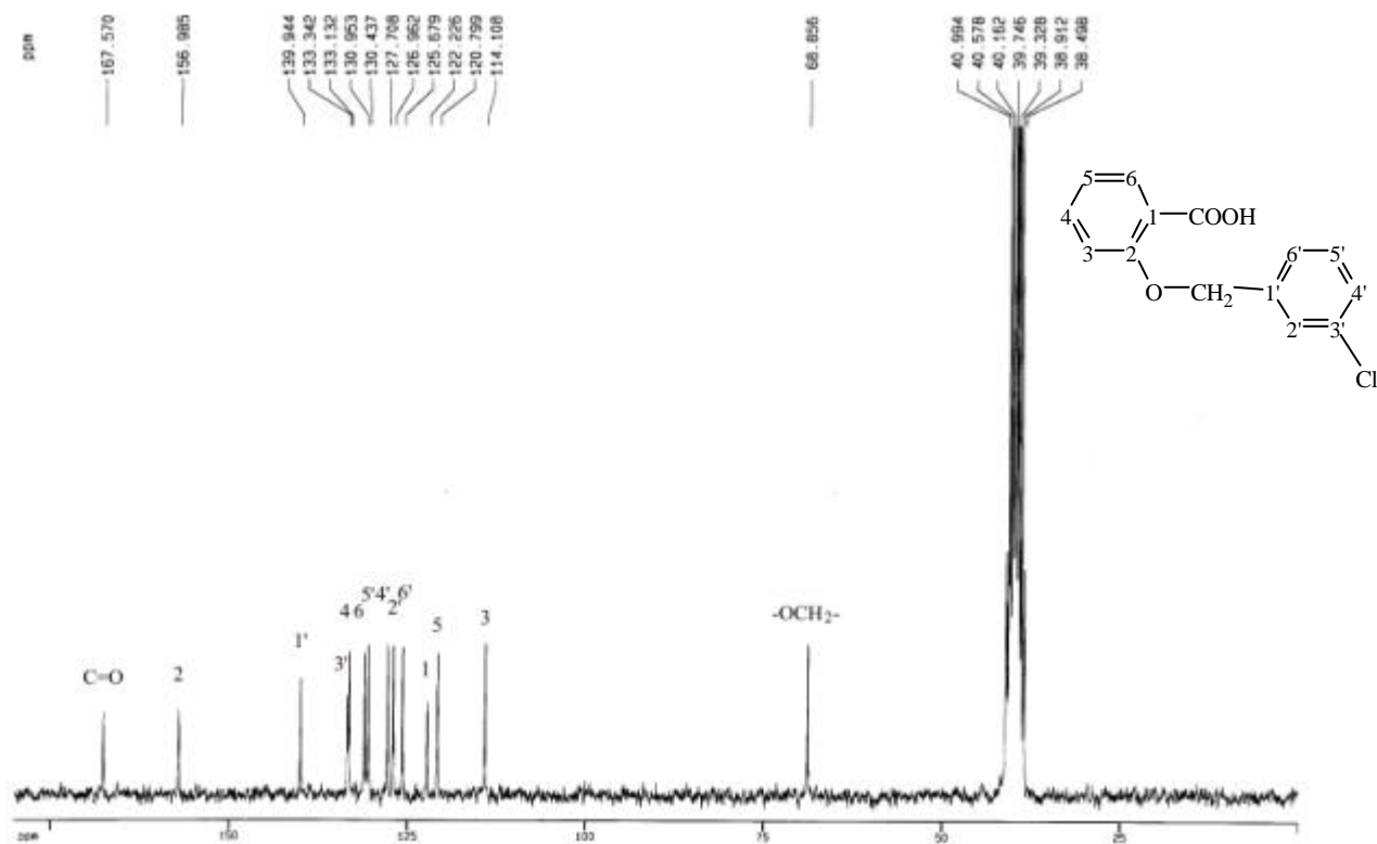
圖 58-4 ^{13}\text{C-NMR} ( \text{DMSO-}d_6 , 50 MHz) spectrum of compound 58
