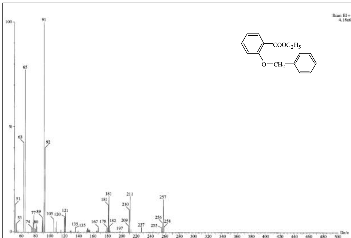
圖 38-1 MS spectrum of compound 38
