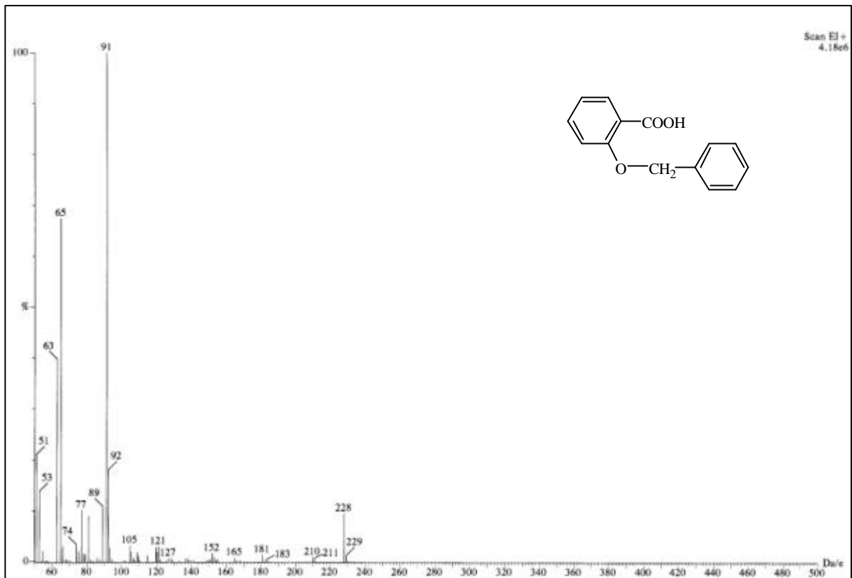
圖 56-1 MS spectrum of compound 56
