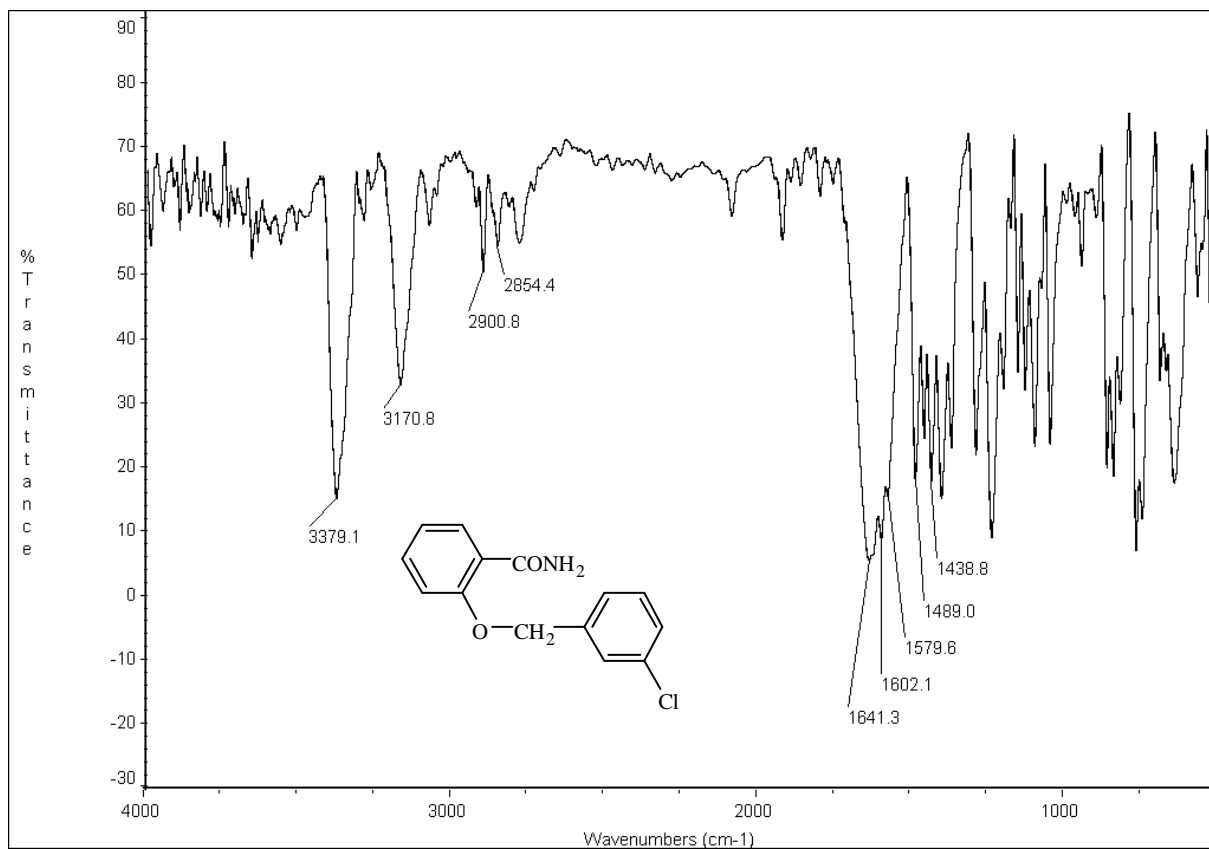
圖 43-2 IR (KBr) spectrum of compound 43
