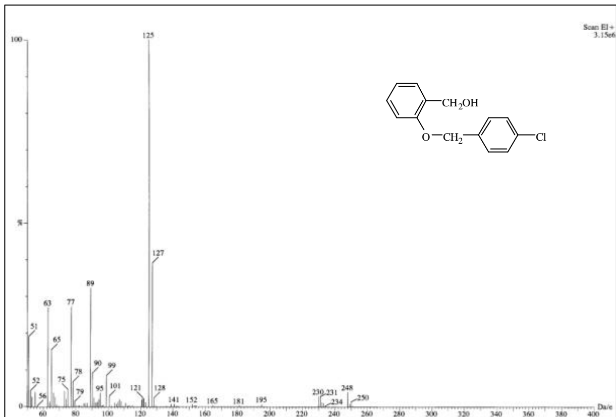
圖 33-1 MS spectrum of compound 33
