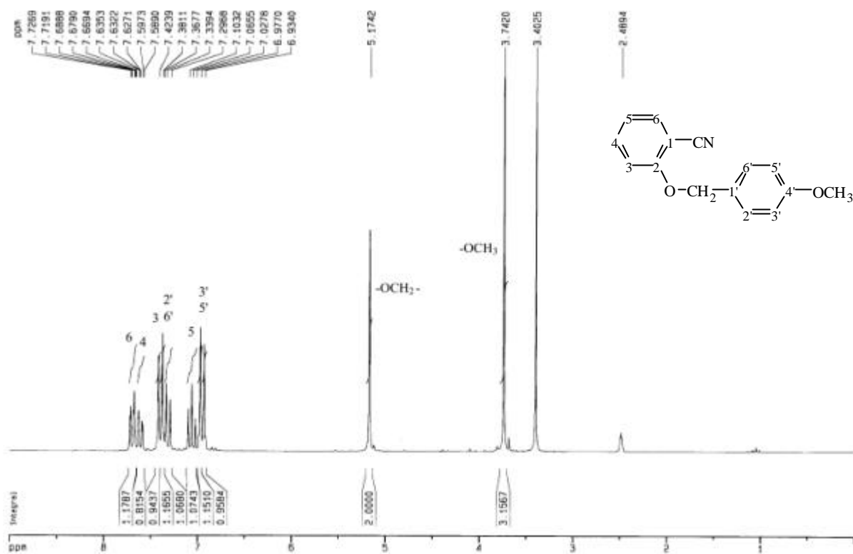
圖 25-3 ^1\text{H-NMR} ( \text{DMSO-}d_6 , 200 MHz) spectrum of compound
