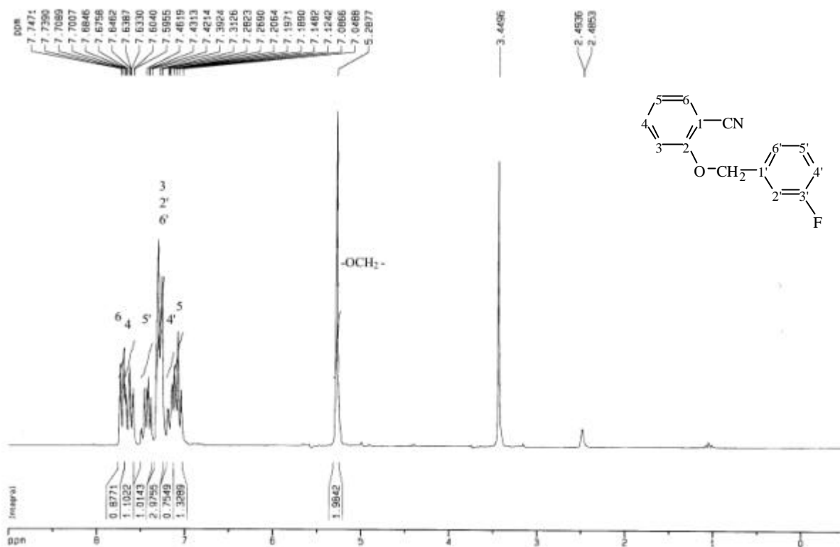
圖 22-3 1 H-NMR (DMSO- d 6 , 200 MHz) spectrum of compound 22
