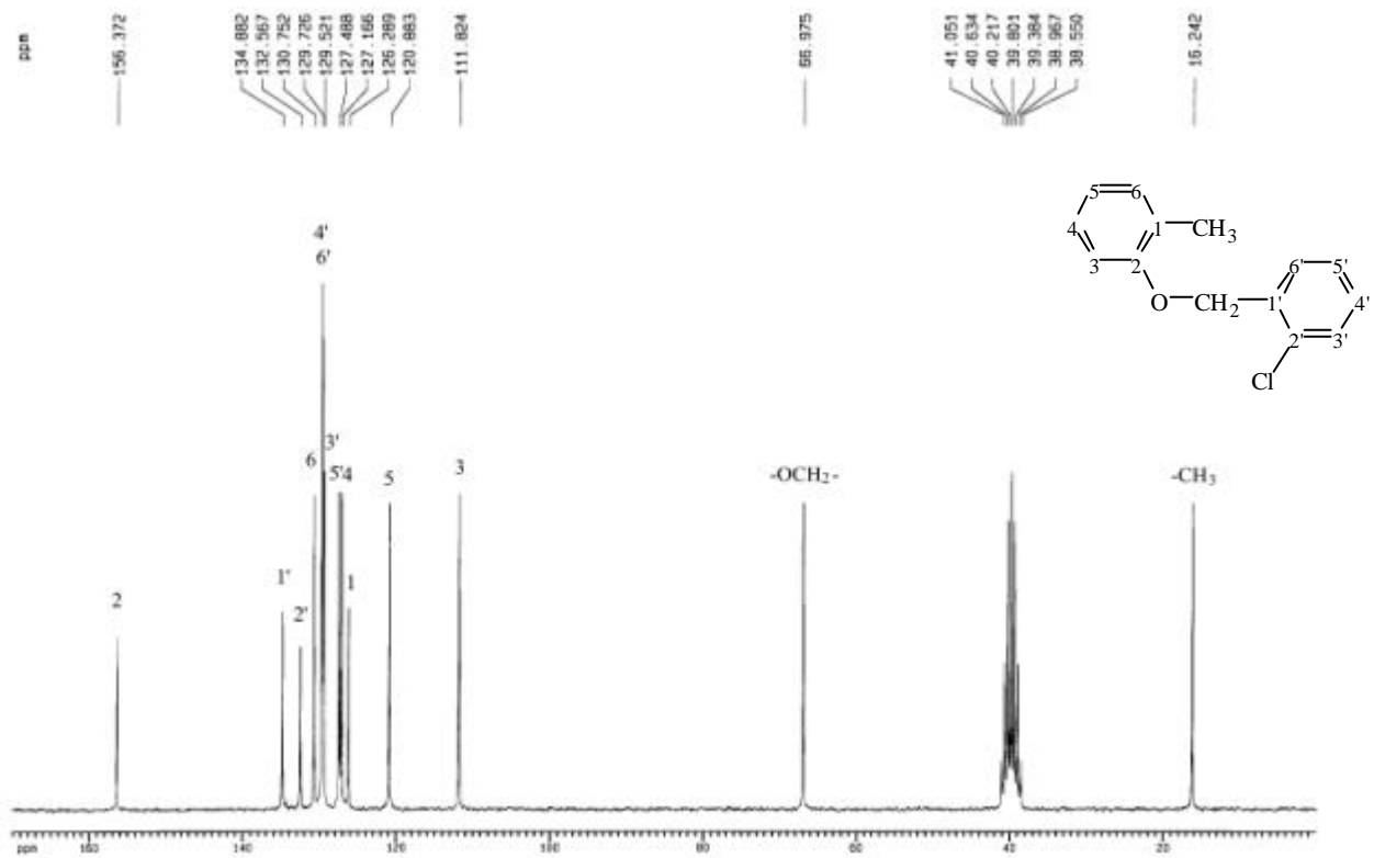
圖 27-4 13 C-NMR (DMSO- d 6 , 50 MHz) spectrum of compound 27
