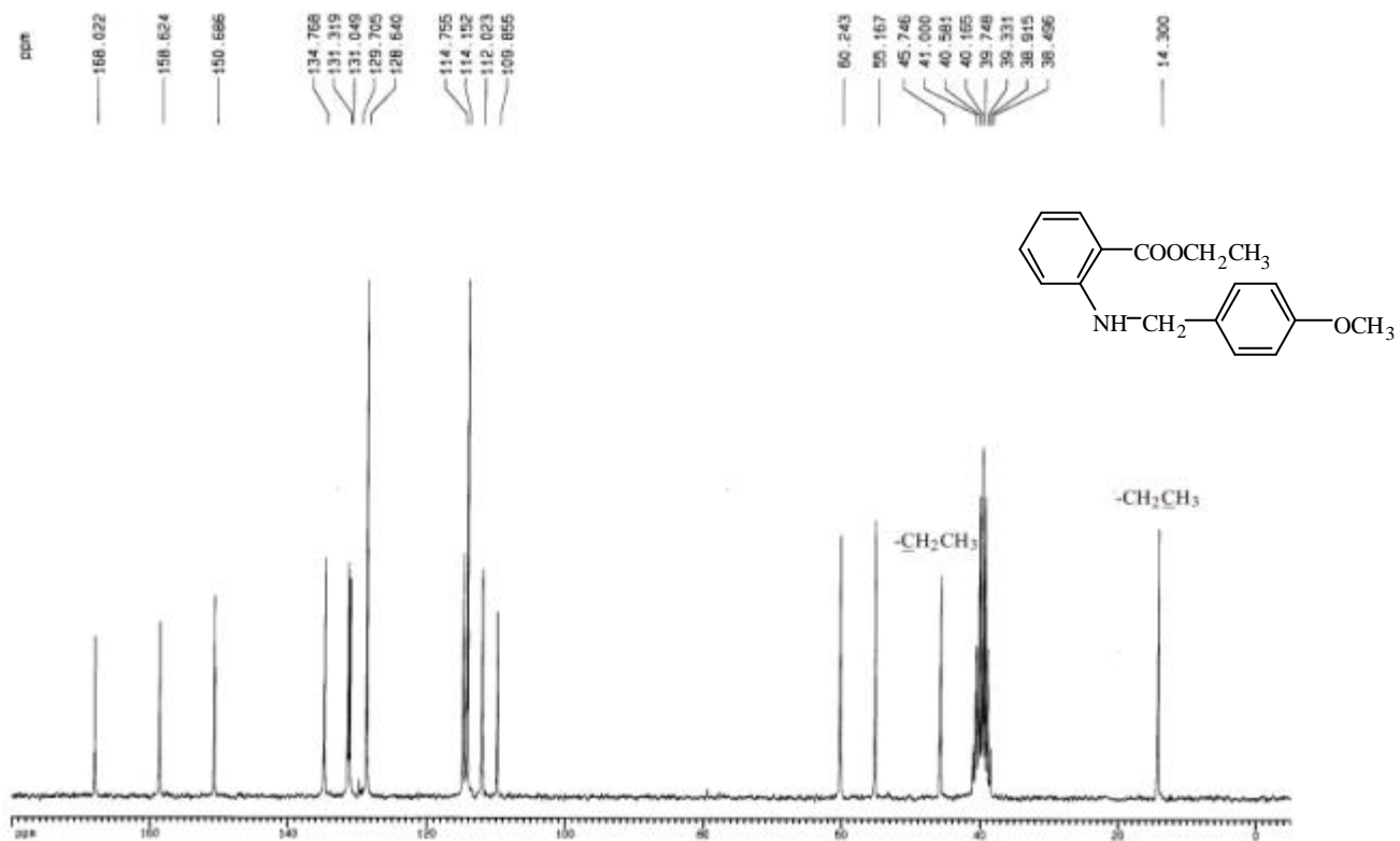
圖 53-2 ^{13}\text{C-NMR} ( \text{DMSO-}d_6 , 50 MHz) spectrum of compound 53
