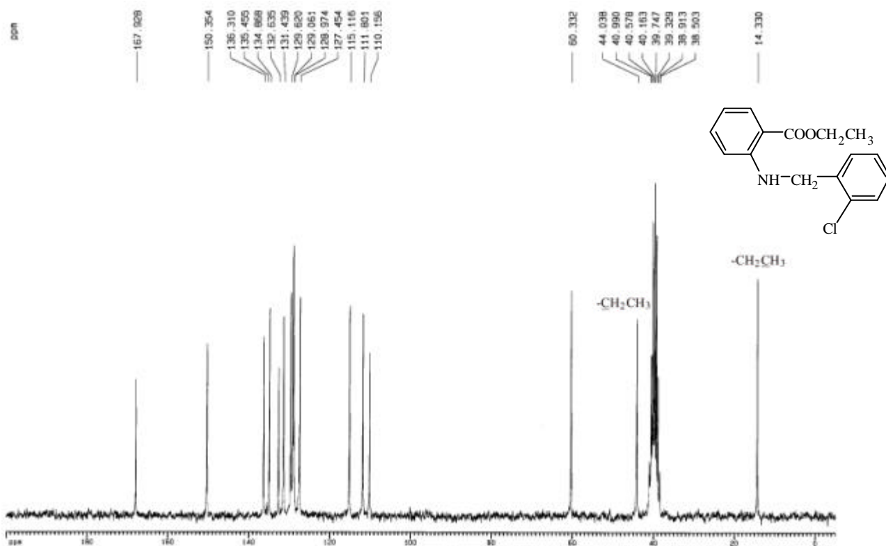
圖 46-2 13 C-NMR (DMSO- d 6 , 50 MHz) spectrum of compound 46
