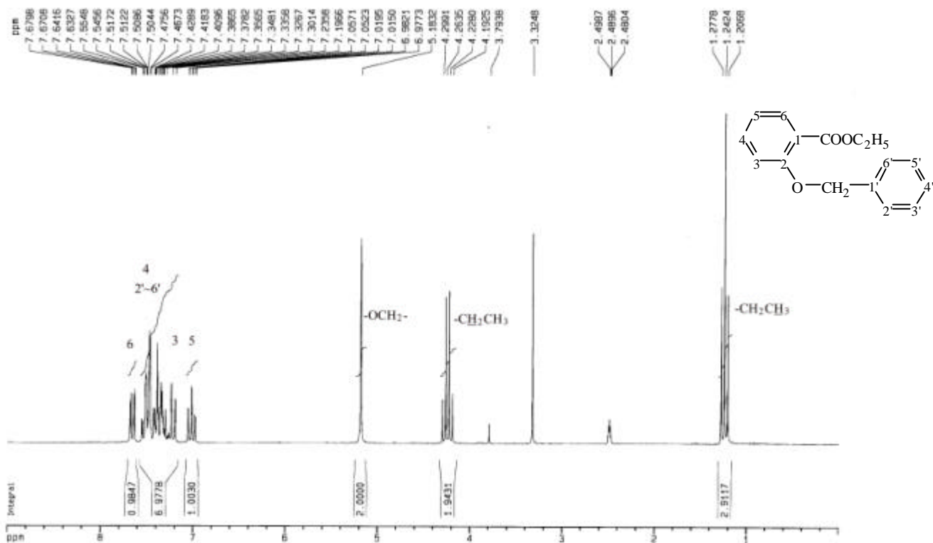
圖 38-3 1 H-NMR (DMSO- d 6 , 200 MHz) spectrum of compound 38
