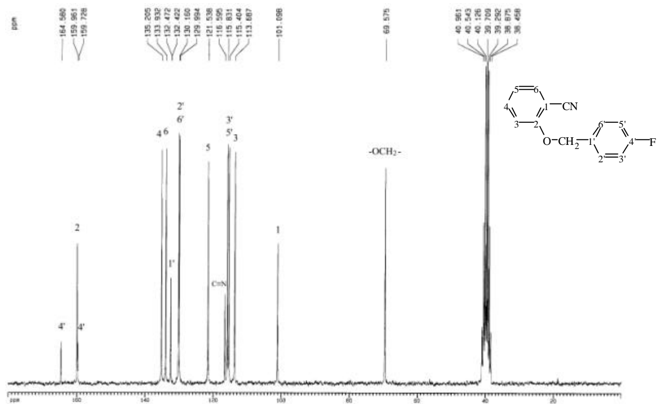
圖 23-4 ^{13}\text{C-NMR} (DMSO- d_6 , 50 MHz) spectrum of compound 23
