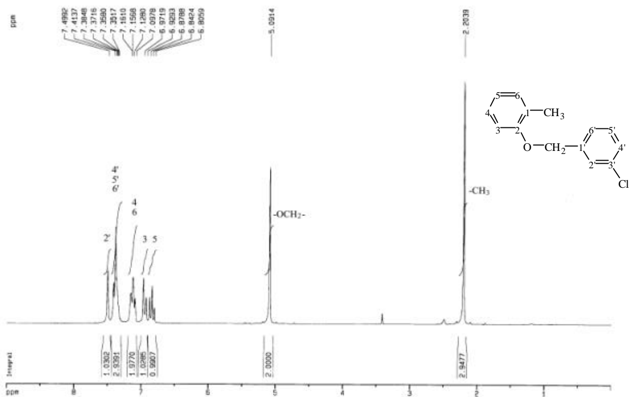
圖 28-3 1 H-NMR (DMSO- d 6 , 200 MHz) spectrum of compound 28
