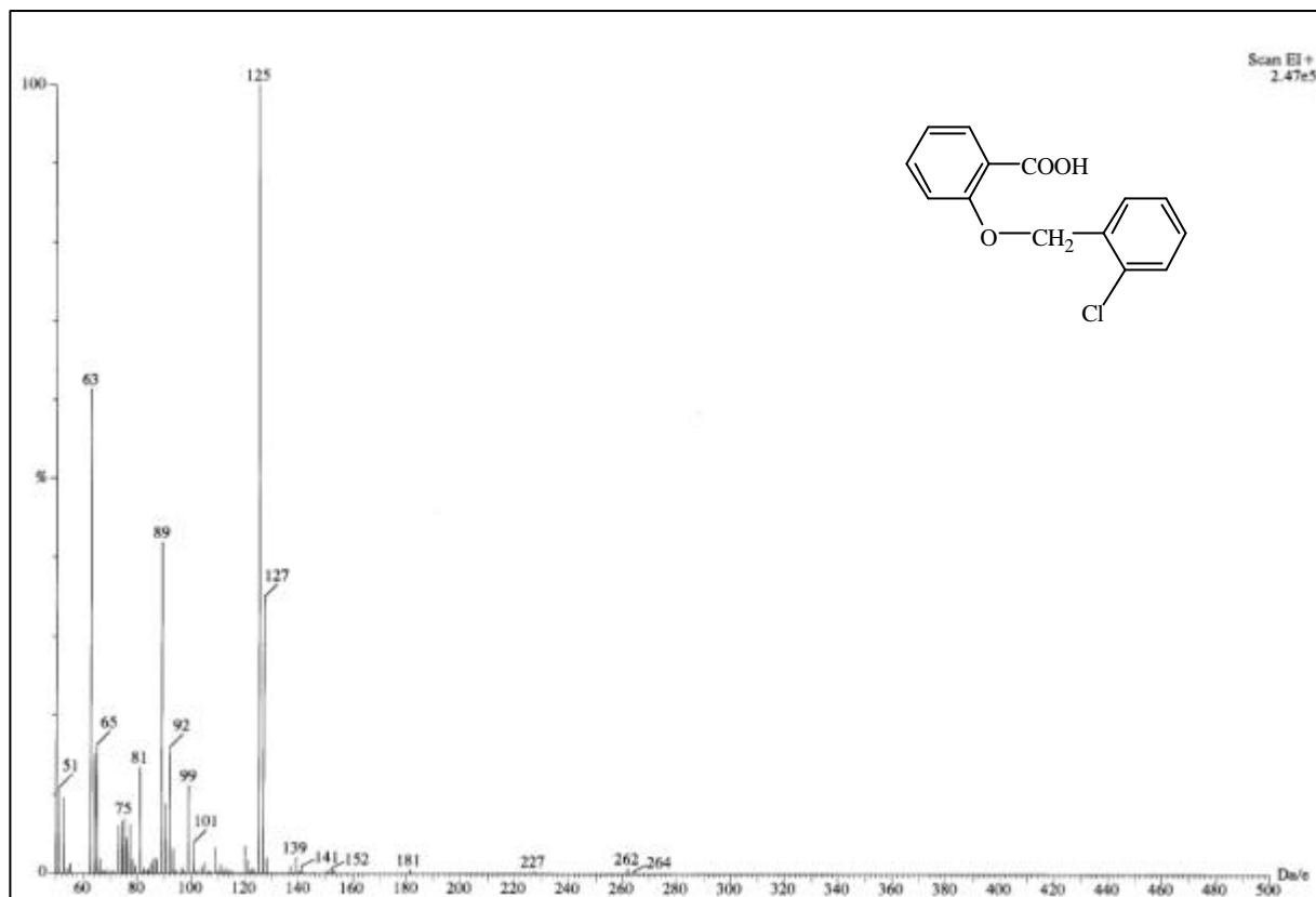
圖 57-1 MS spectrum of compound 57
