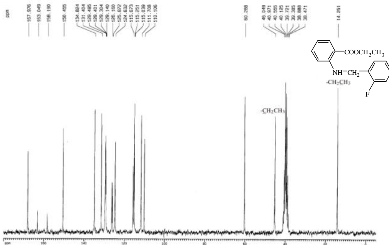
圖 49-2 13 C-NMR (DMSO- d 6 , 50 MHz) spectrum of compound 49
