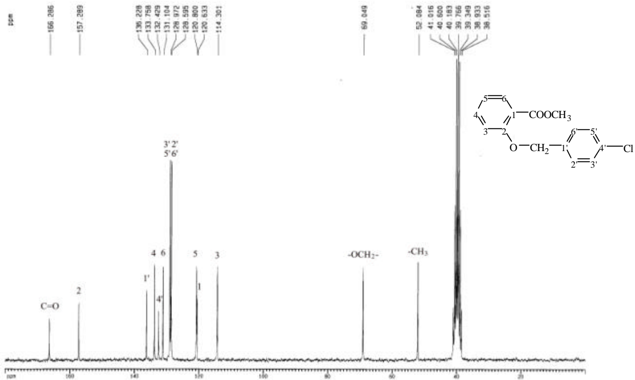
圖 37-4 13 C-NMR (DMSO- d 6 , 50 MHz) spectrum of compound 37
