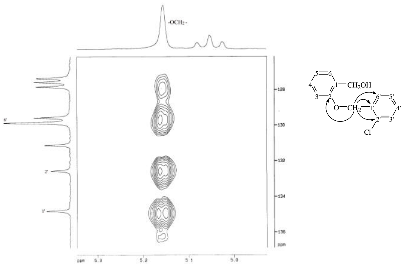
圖 31-5d HMBC (DMSO- d_6 ) spectrum of compound 31
