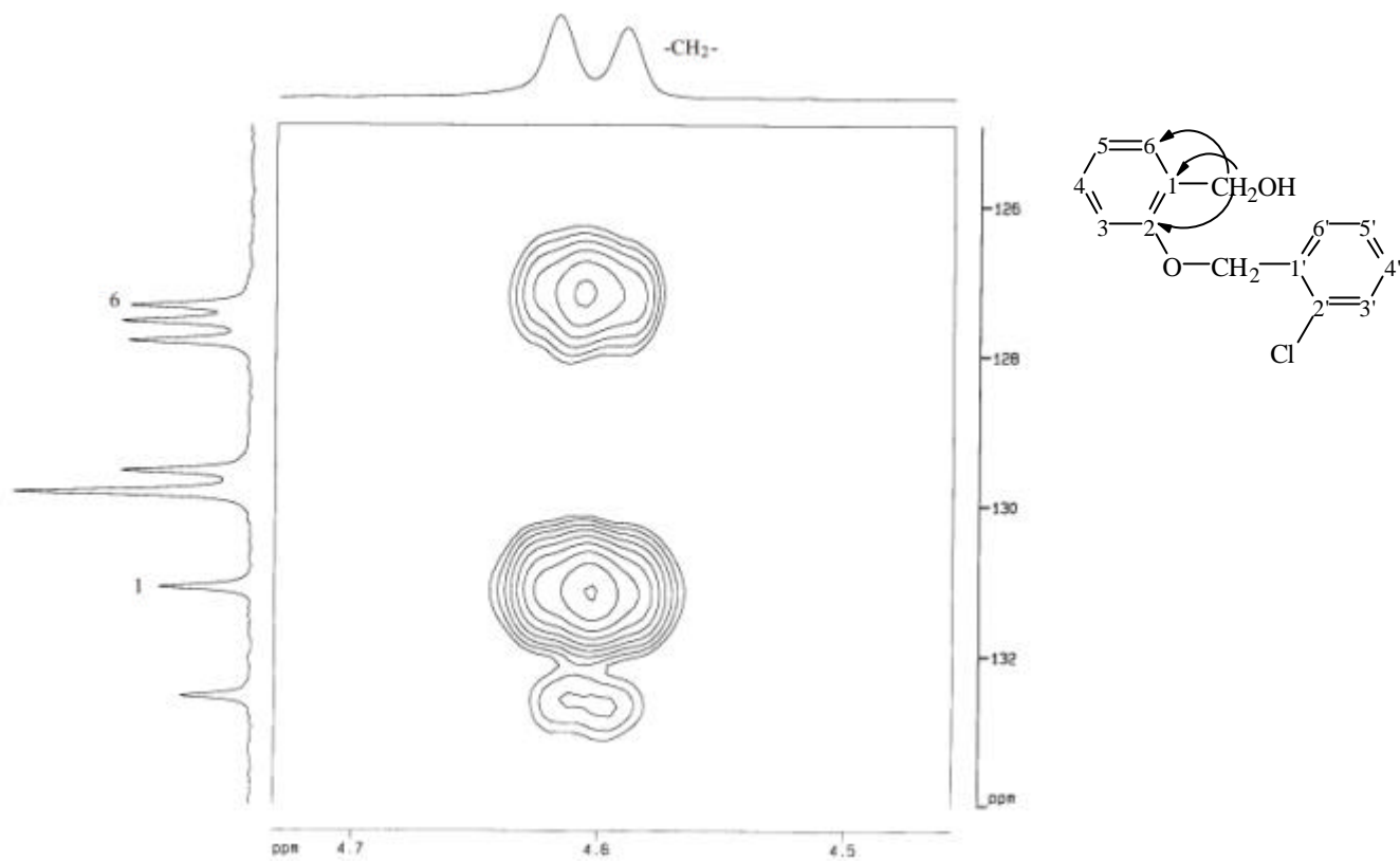
圖 31-5c HMBC (DMSO- d_6 ) spectrum of compound 31
