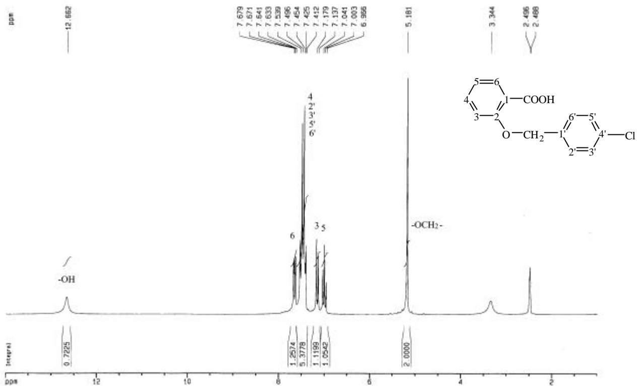
圖 59-3 ^1\text{H-NMR} ( \text{DMSO-}d_6 , 200 MHz) spectrum of compound 59
