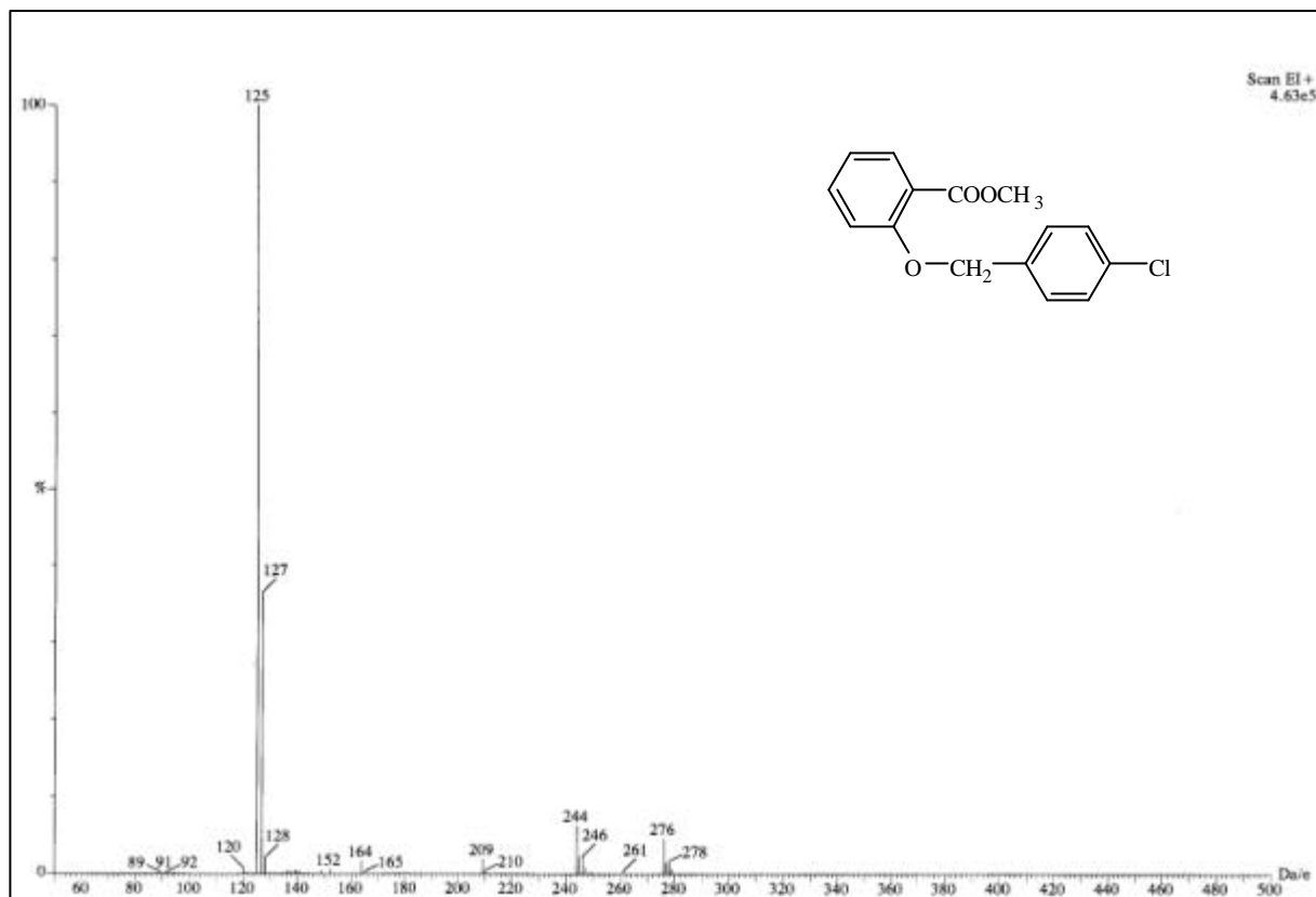
圖 37-1 MS spectrum of compound 37
