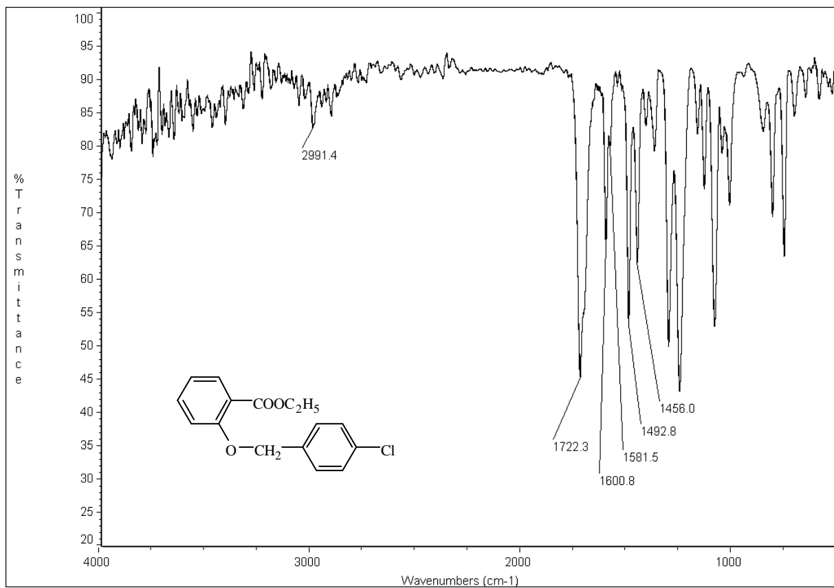
圖 41-2 IR (KBr) spectrum of compound 41
