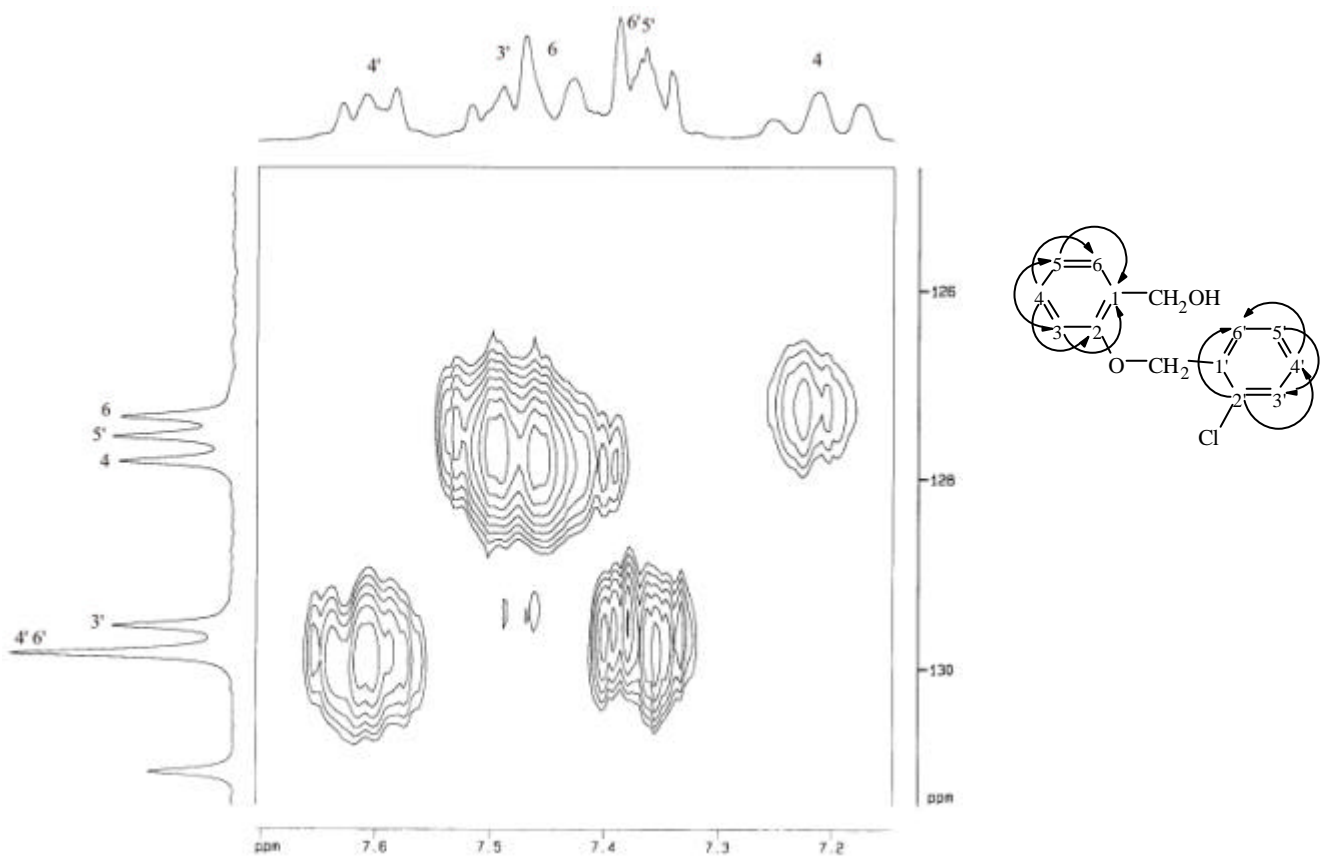
圖 31-5b HMBC (DMSO- d_6 ) spectrum of compound 31
