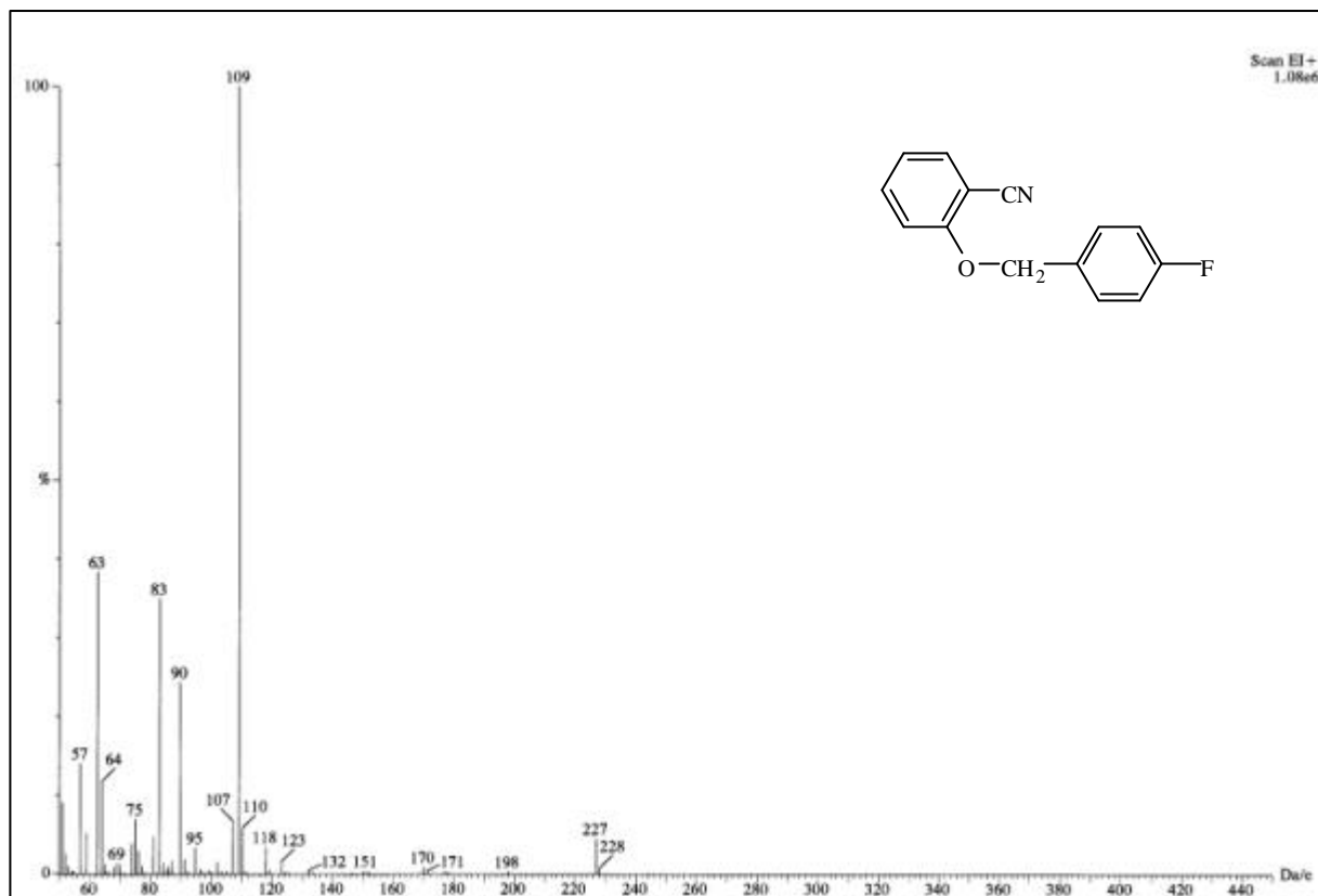
圖 23-1 MS spectrum of compound 23
