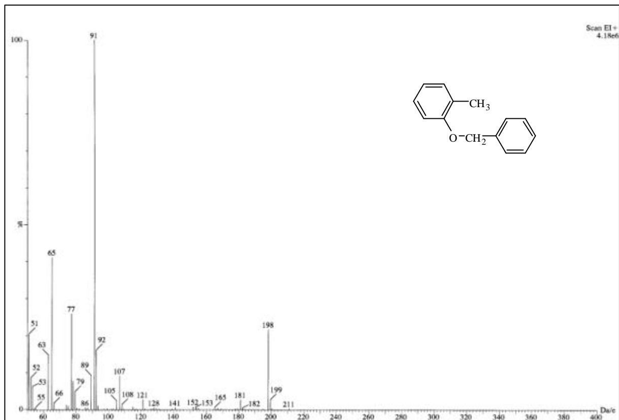
圖 26-1 MS spectrum of compound 26
