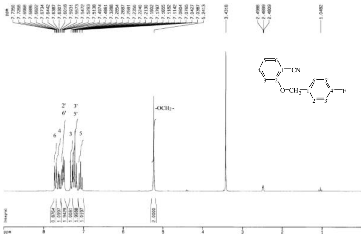
圖 23-3 ^1\text{H-NMR} (DMSO- d_6 , 200 MHz) spectrum of compound 23
