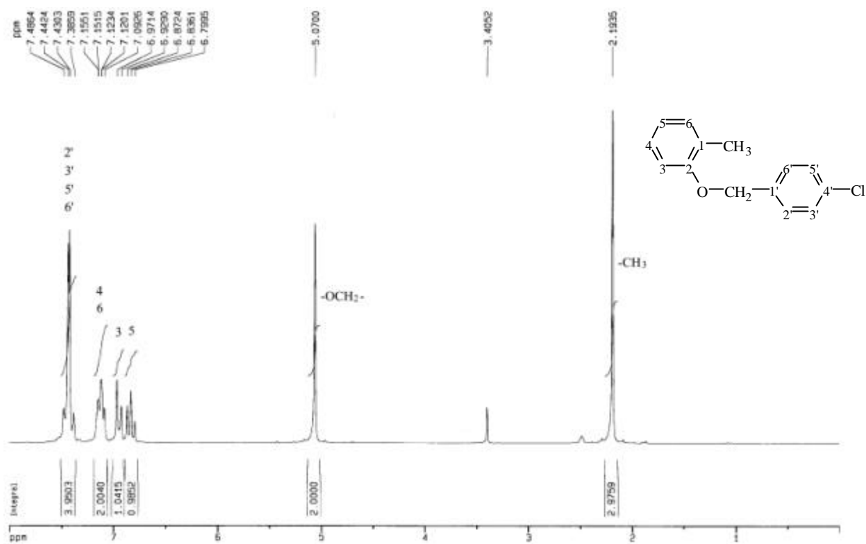
圖 29-3 ^1\text{H-NMR} (DMSO- d_6 , 200 MHz) spectrum of compound 29
