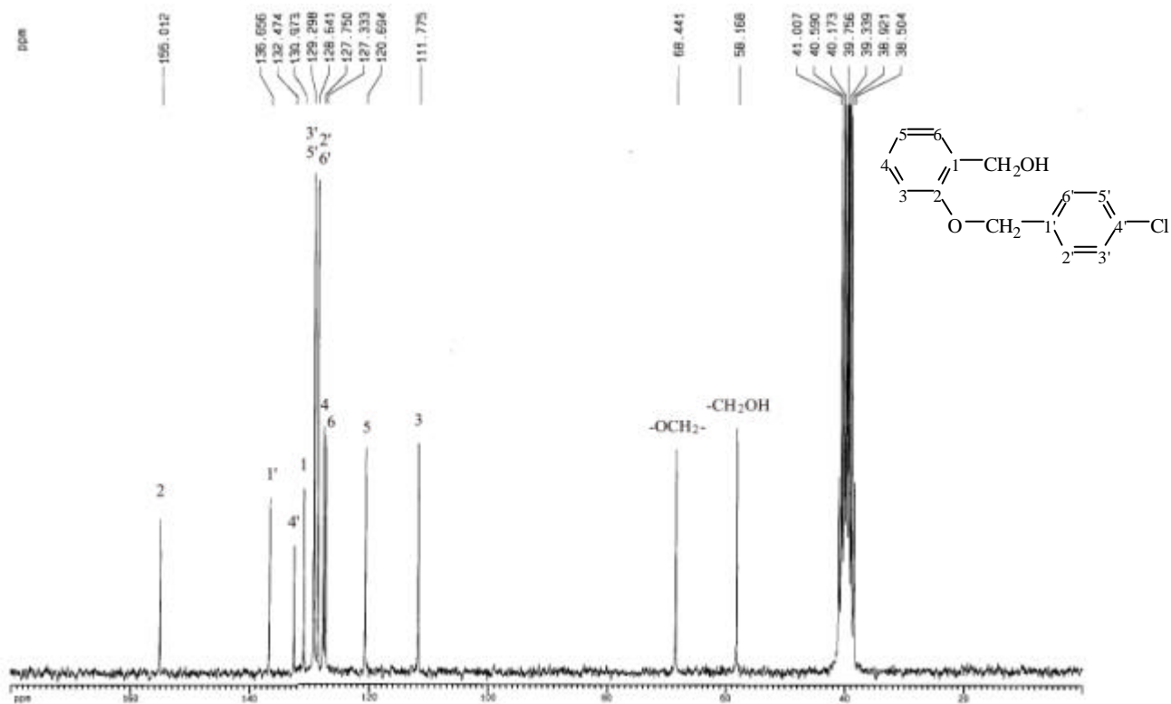
圖 33-4 13 C-NMR (DMSO- d 6 , 50 MHz) spectrum of compound 33
