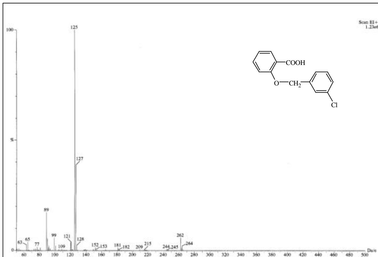
圖 58-1 MS spectrum of compound 58
