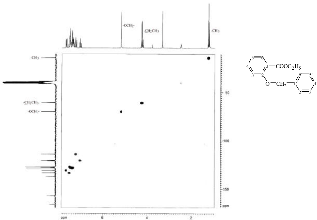
圖 38-6a HMQC (DMSO- d_6 ) spectrum of compound 38
