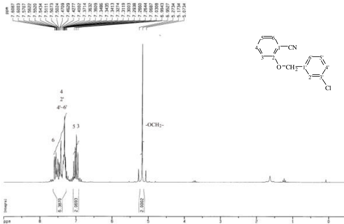
圖 19-3 ^1\text{H-NMR} ( \text{CDCl}_3 , 200 MHz) spectrum of compound 19
