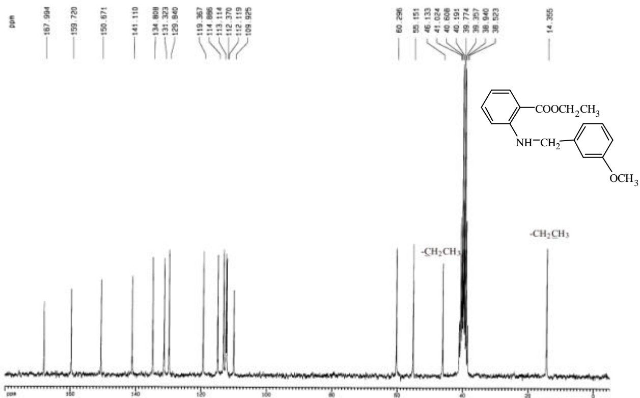
圖 52-2 13 C-NMR (DMSO- d 6 , 50 MHz) spectrum of compound 52
