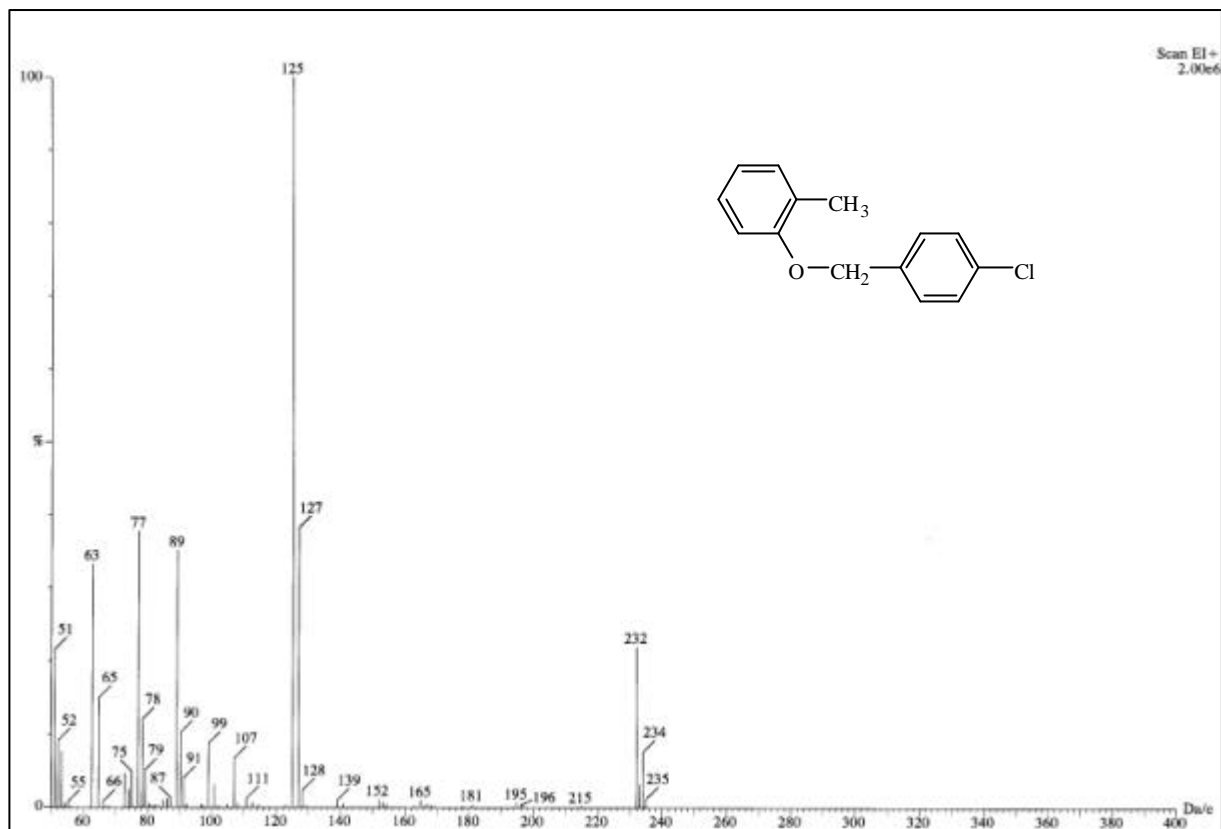
圖 29-1 MS spectrum of compound 29
