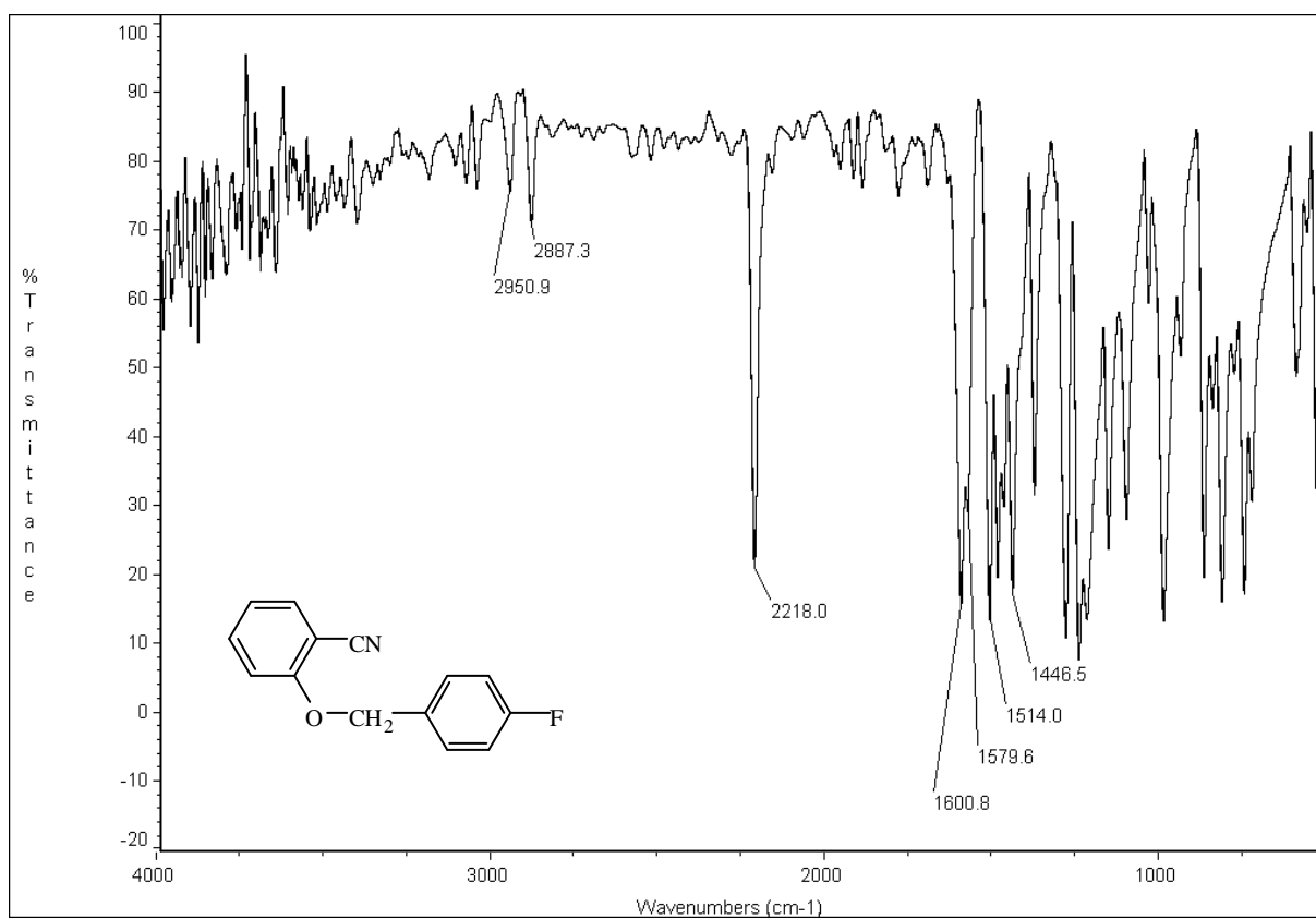
圖 23-2 IR (KBr) spectrum of compound 23
