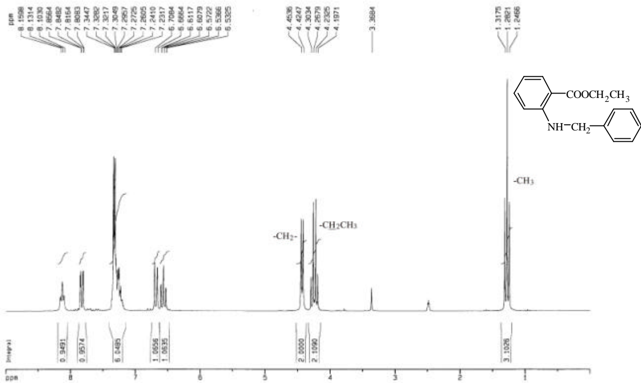
圖 45-1 ^1\text{H-NMR} ( \text{DMSO-}d_6 , 200 MHz) spectrum of compound 45
