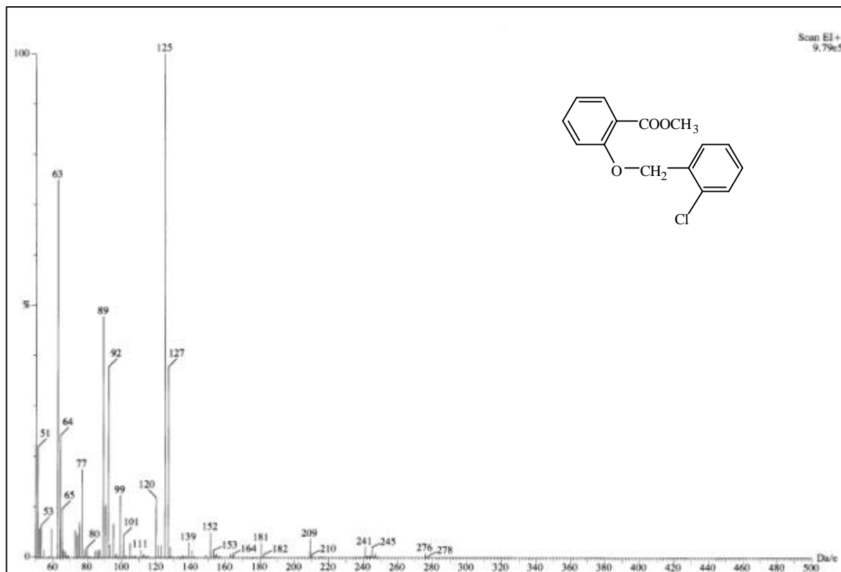
圖 35-1 MS spectrum of compound 35
