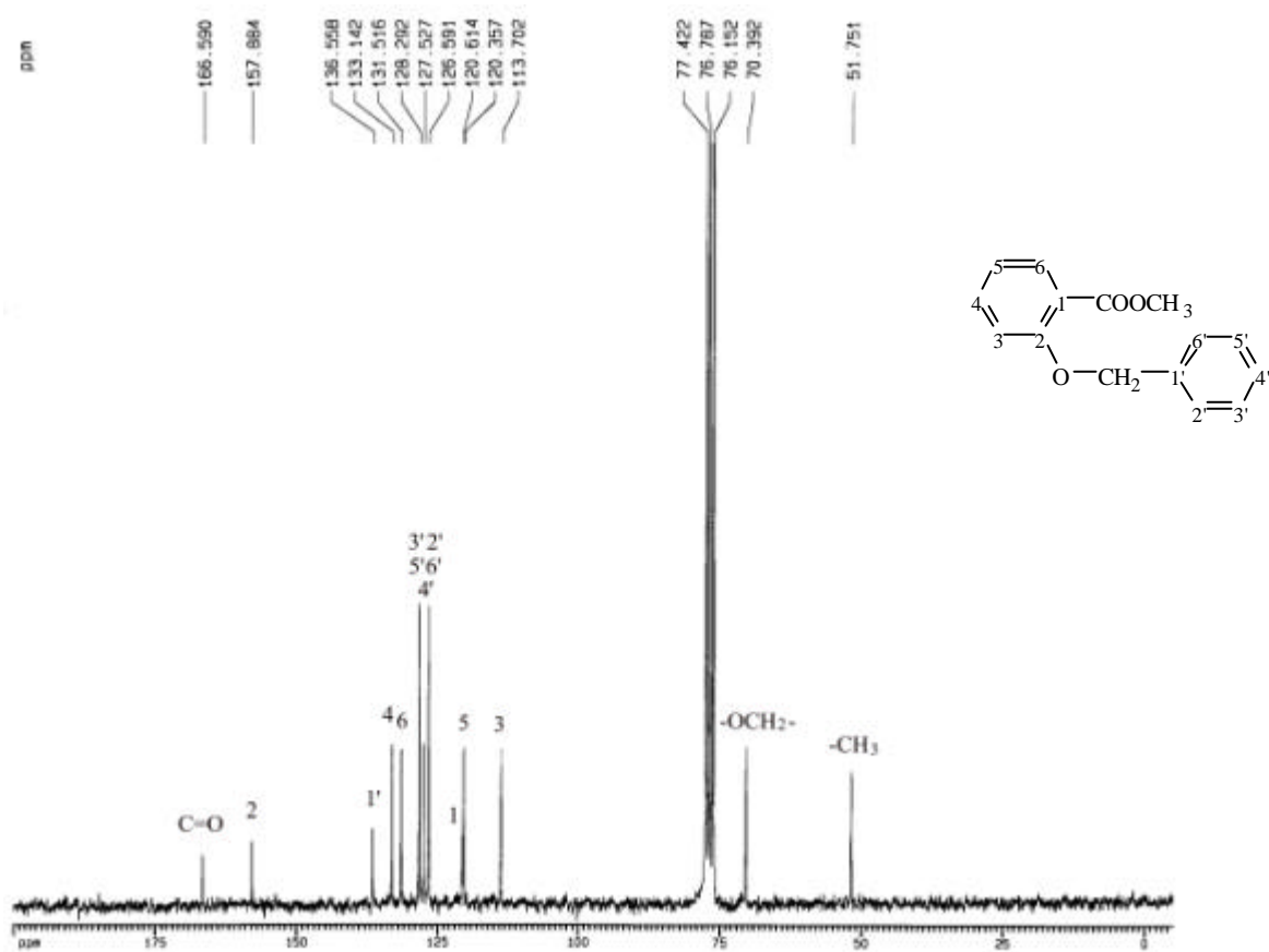
圖 34-4 13 C-NMR (CDCl 3 , 50 MHz) spectrum of compound 34
