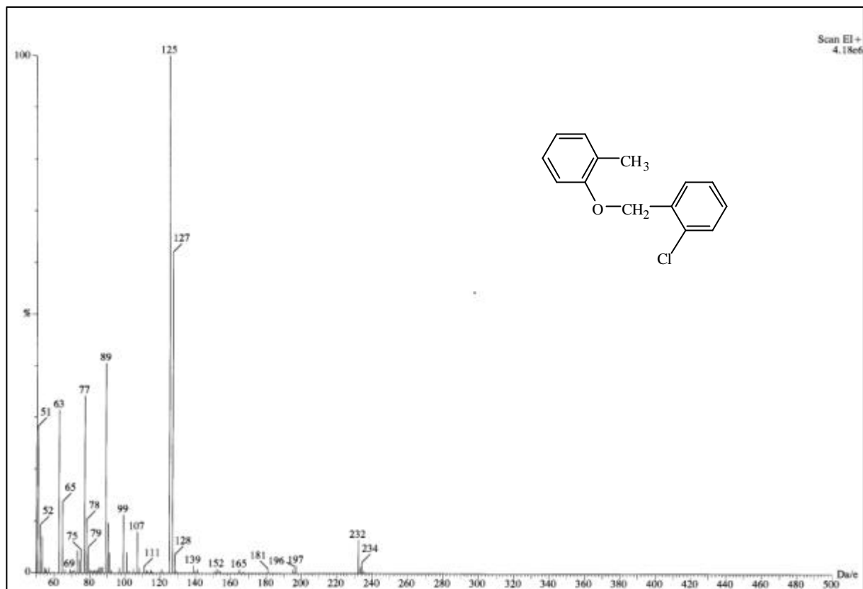
圖 27-1 MS spectrum of compound 27
