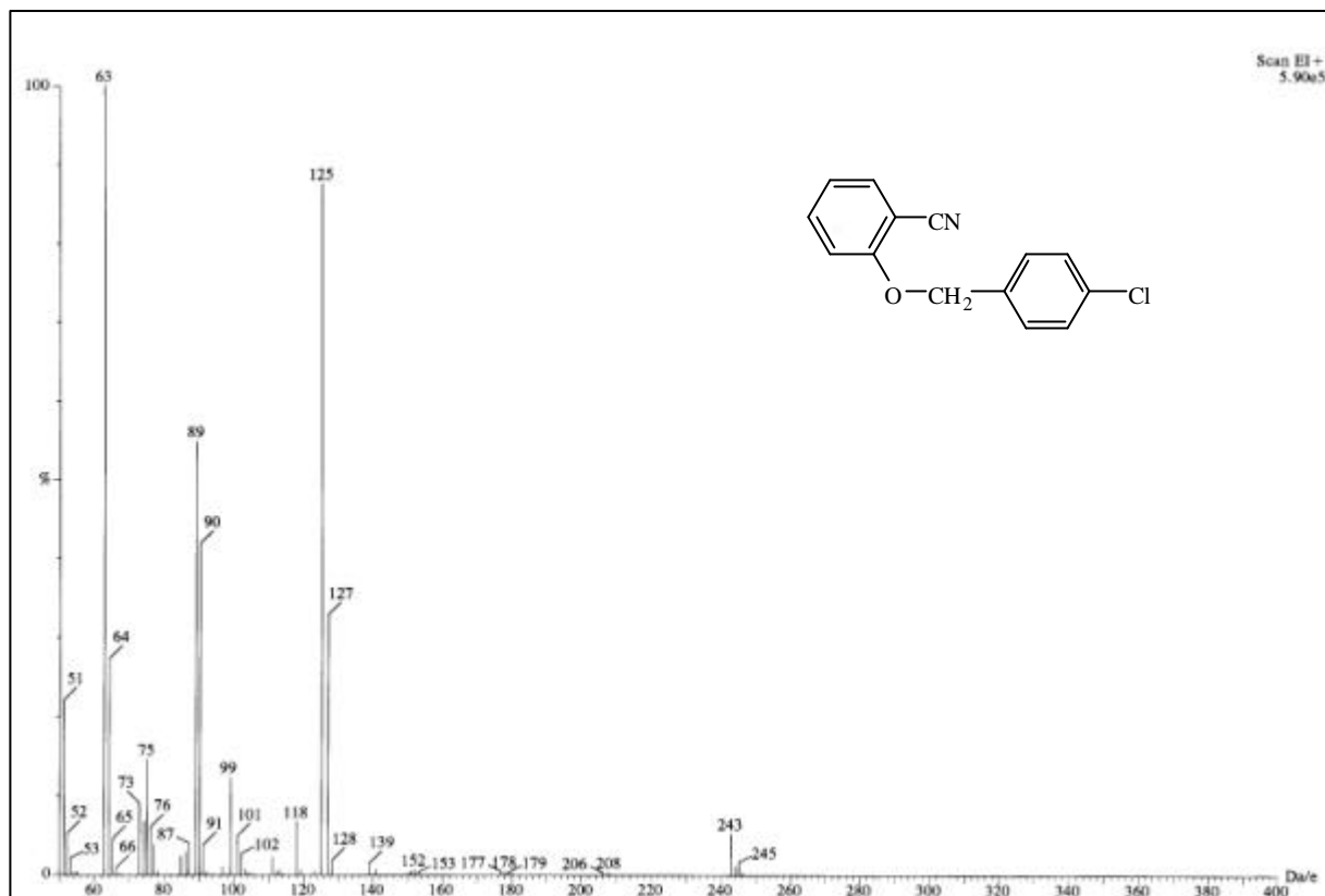
圖 20-1 MS spectrum of compound 20
