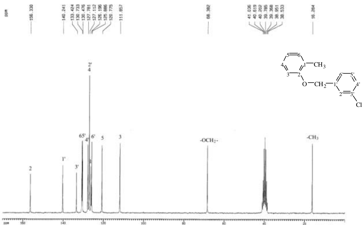
圖 28-4 13 C-NMR (DMSO- d 6 , 50 MHz) spectrum of compound 28
