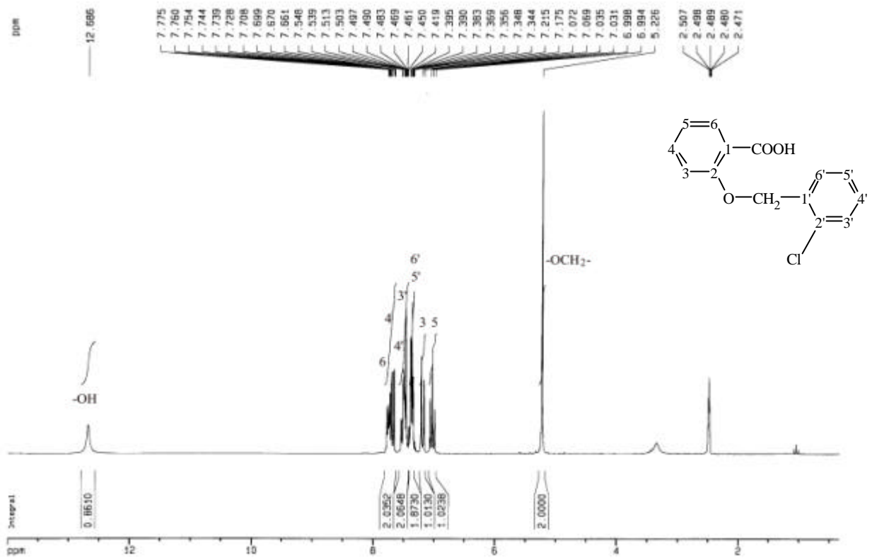
圖 57-3 ^1\text{H-NMR} ( \text{DMSO-}d_6 , 200 MHz) spectrum of compound 57
