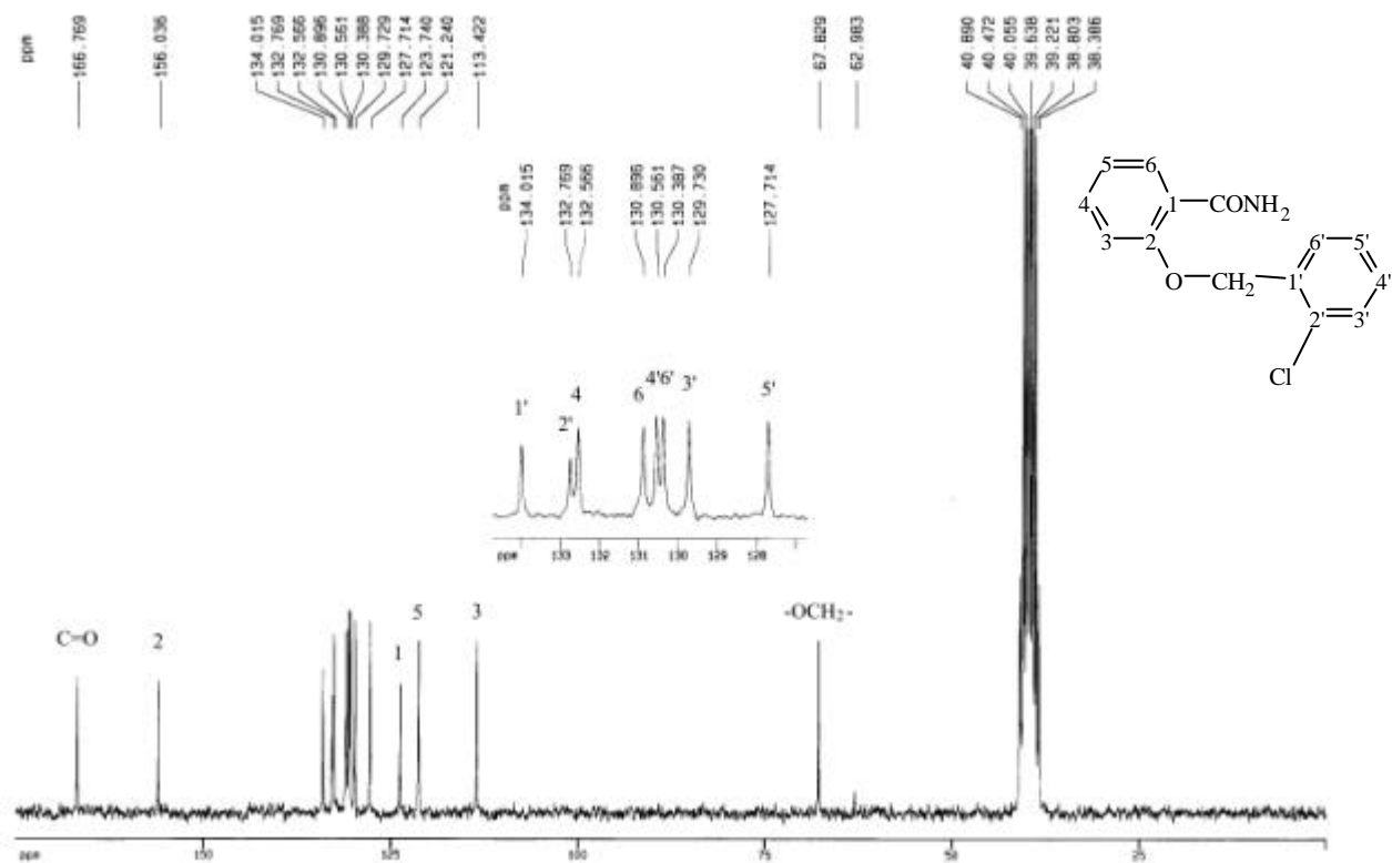
圖 42-4 ^{13}\text{C-NMR} (DMSO- d_6 , 50 MHz) spectrum of compound 42
