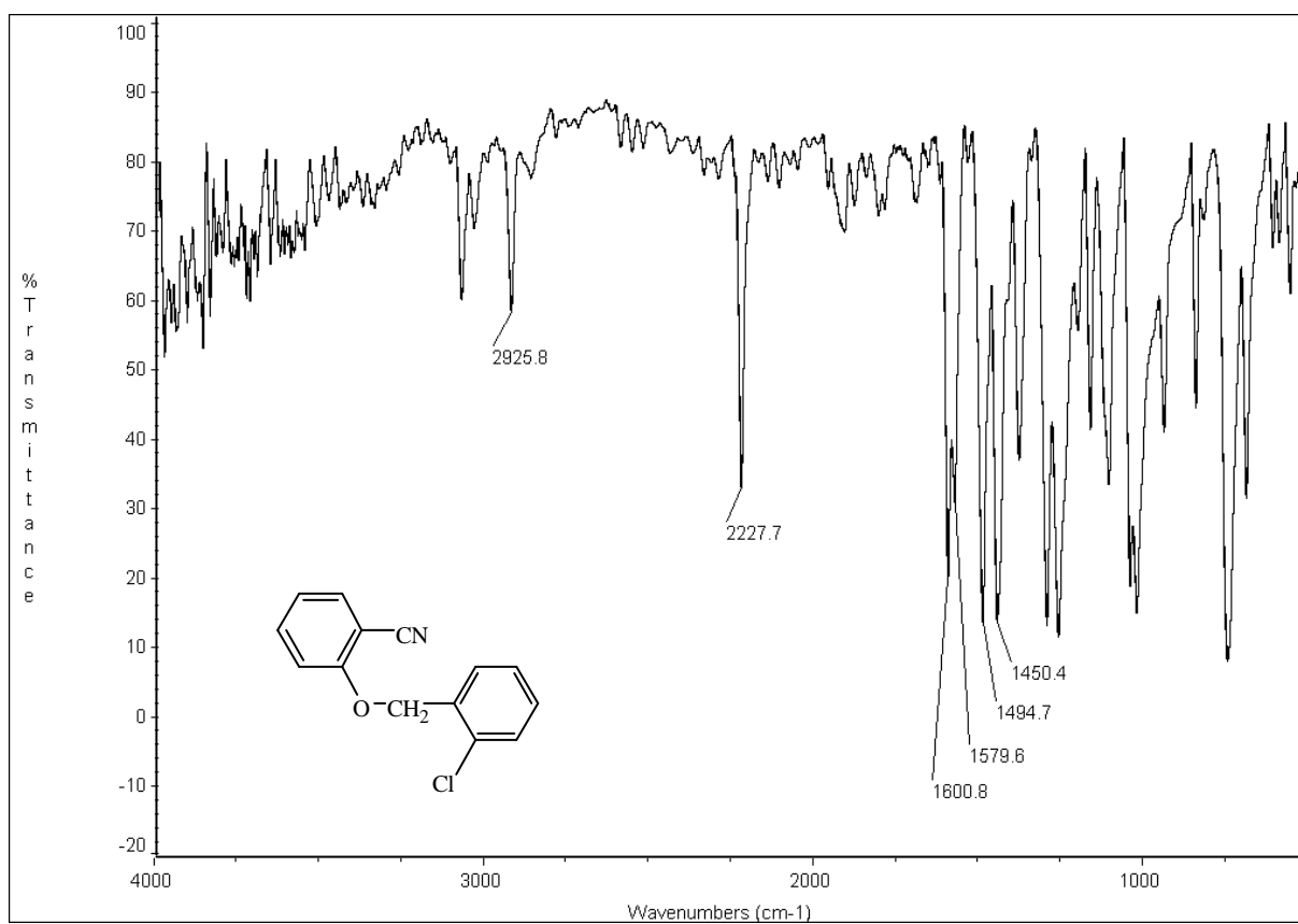
圖 18-2 IR (KBr) spectrum of compound 18
