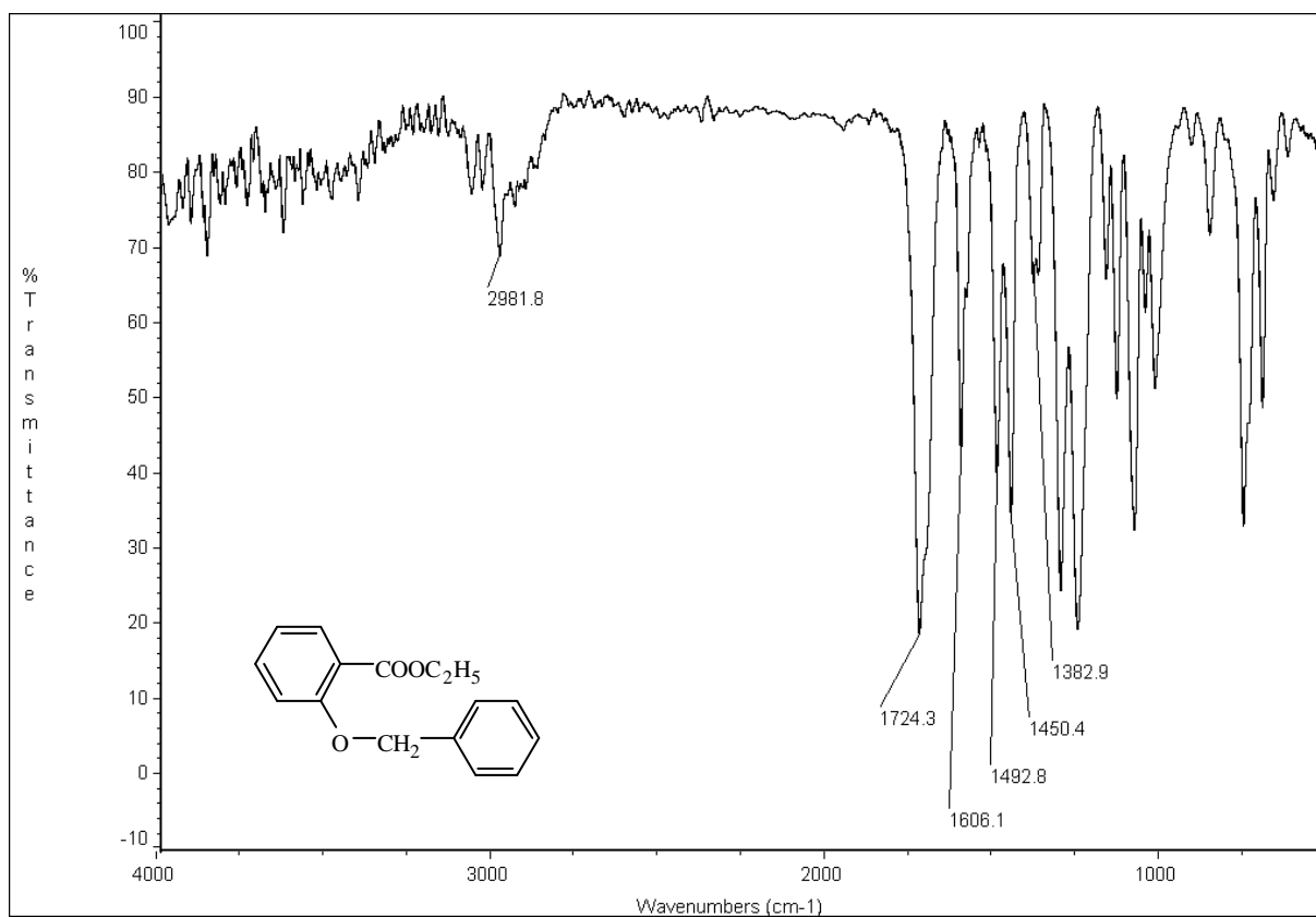
圖 38-2 IR (KBr) spectrum of compound 38
