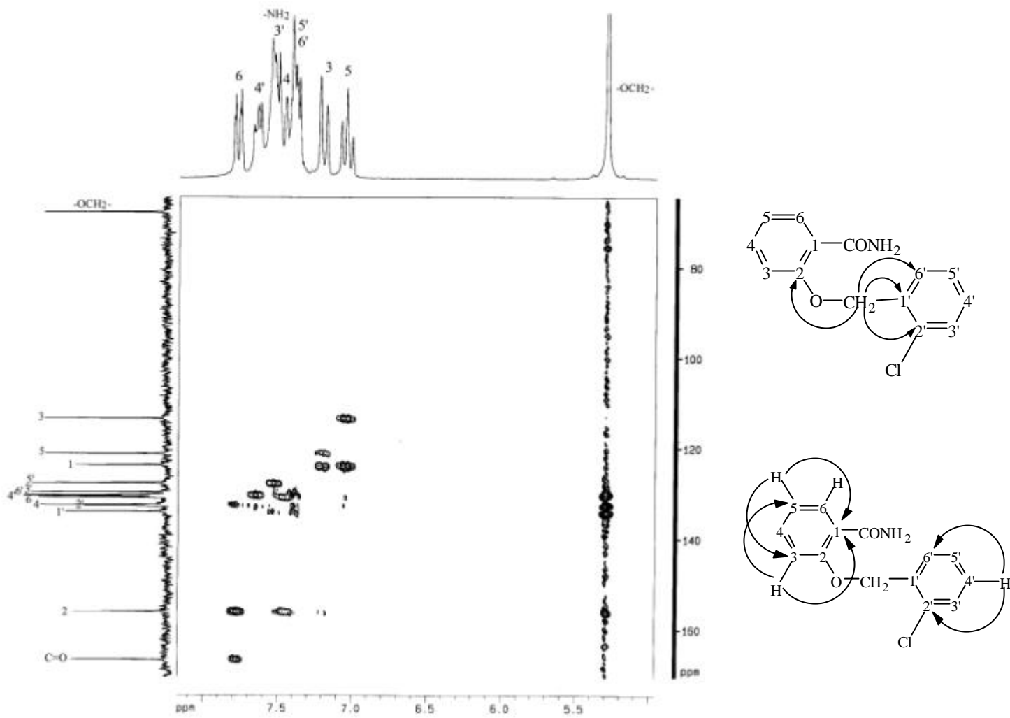
圖 42-5a HMBC (DMSO- d_6 ) spectrum of compound 42
