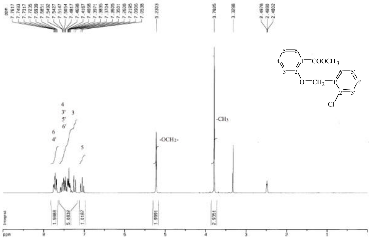
圖 35-3 1 H-NMR (DMSO- d 6 , 200 MHz) spectrum of compound 35
