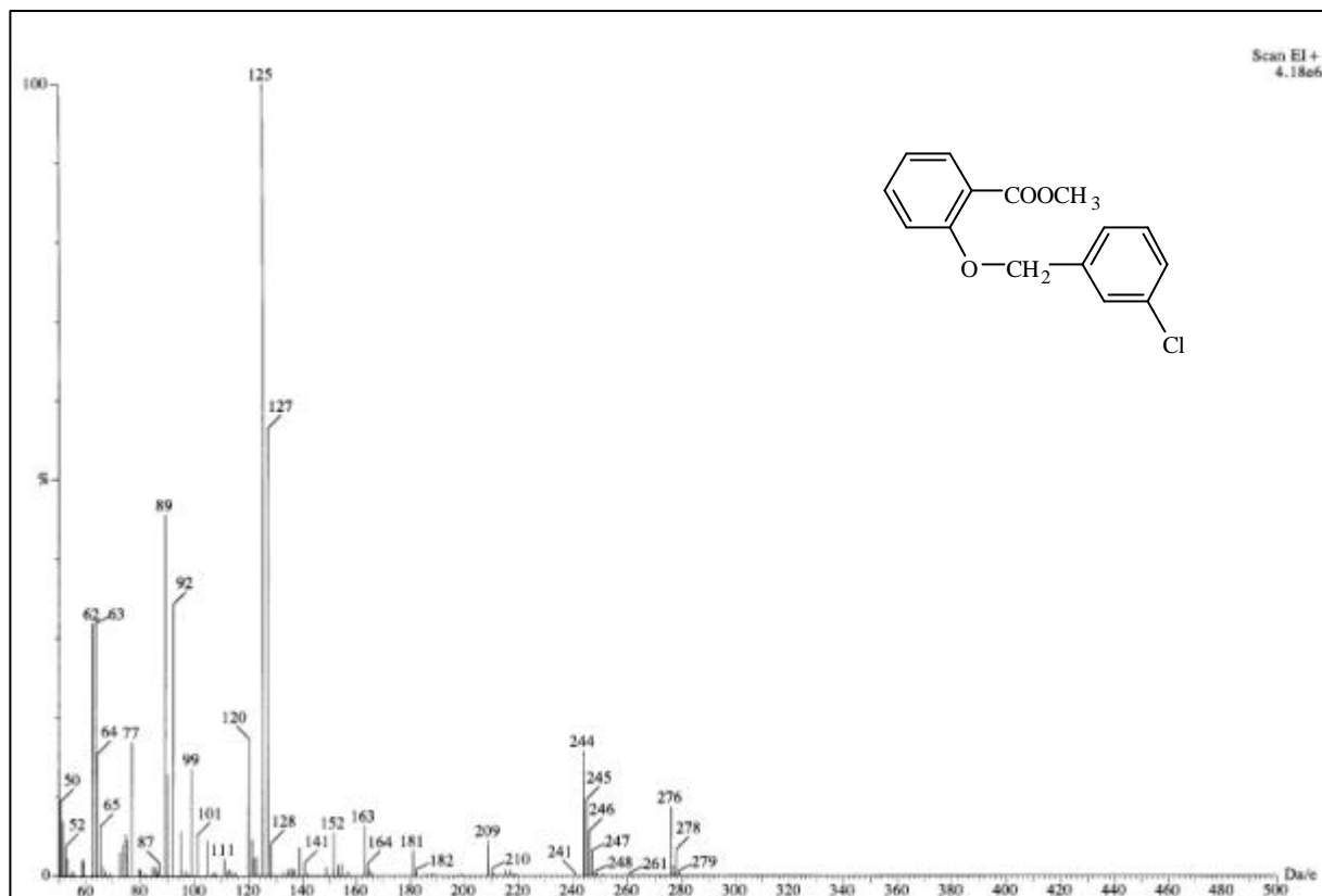
圖 36-1 MS spectrum of compound 36
