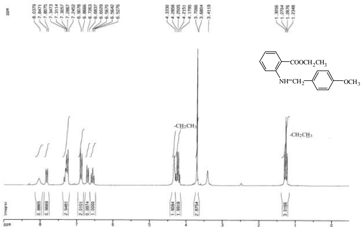
圖 53-1 ^1\text{H-NMR} ( \text{DMSO-}d_6 , 200 MHz) spectrum of compound 53
