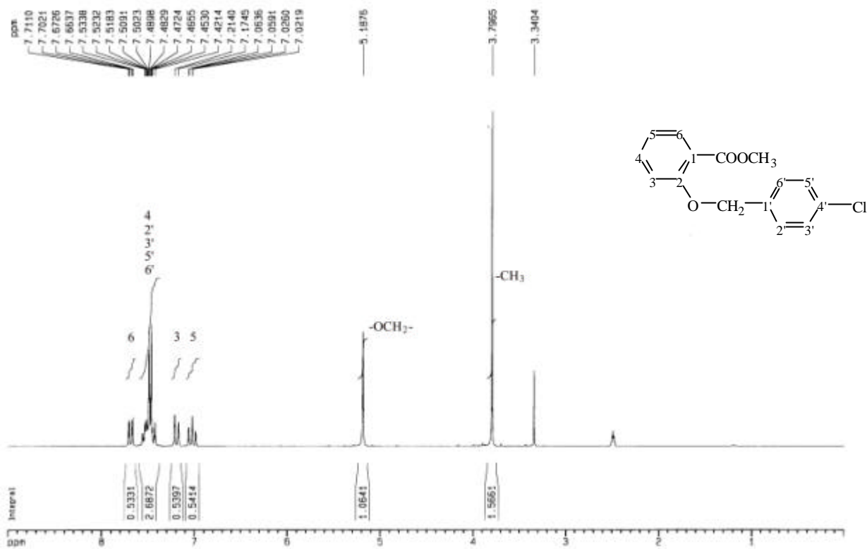
圖 37-3 1 H-NMR (DMSO- d 6 , 200 MHz) spectrum of compound 37
