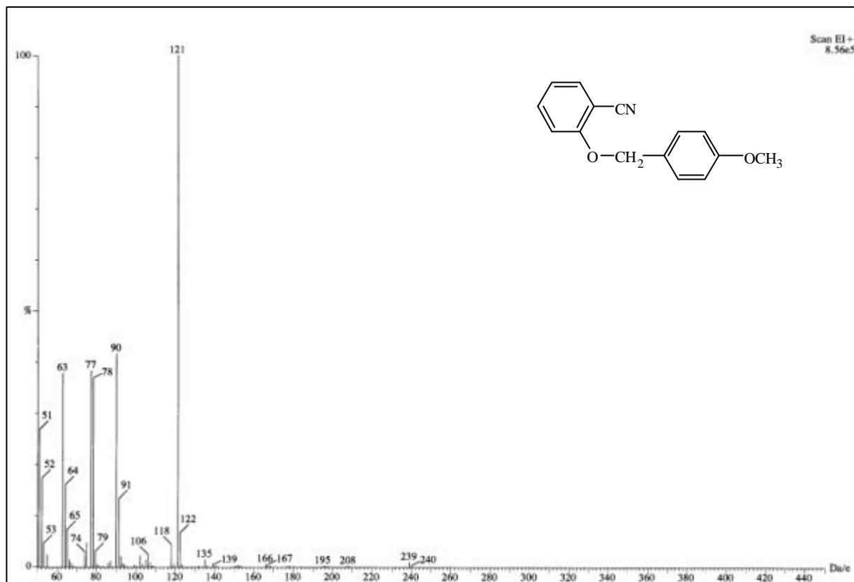
圖 25-1 MS spectrum of compound 25
