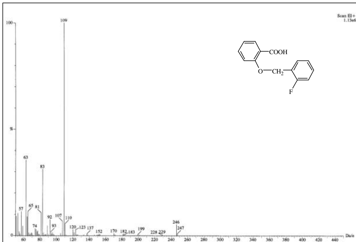
圖 60-1 MS spectrum of compound 60
