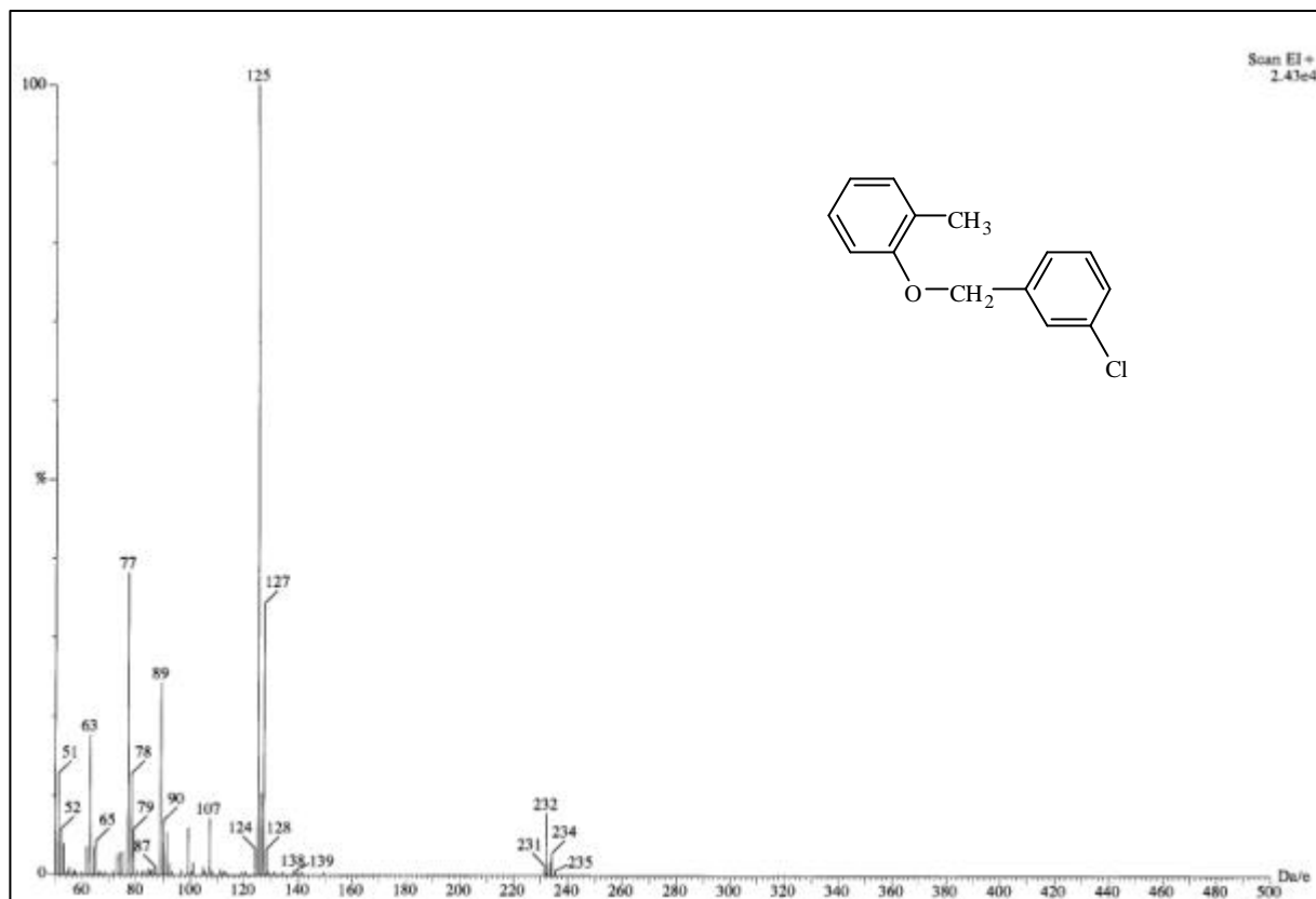
圖 28-1 MS spectrum of compound 28
