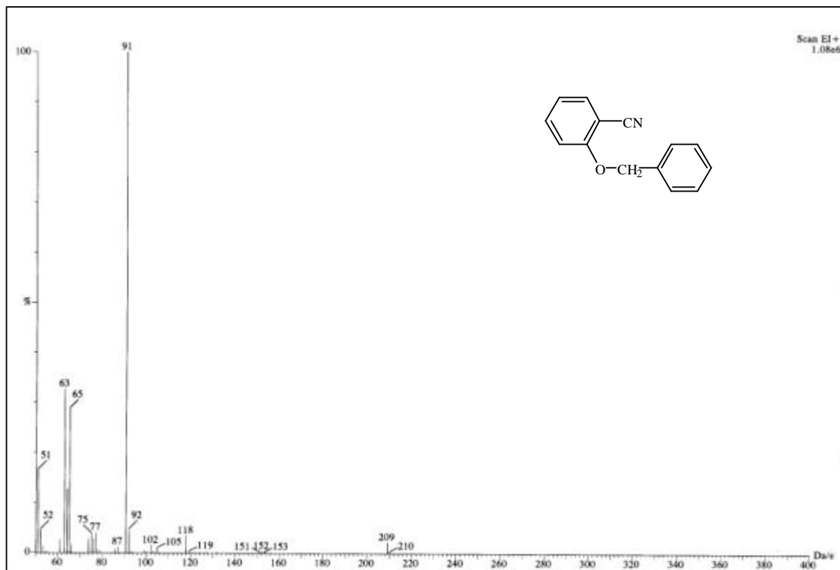
圖 17-1 MS spectrum of compound 17
