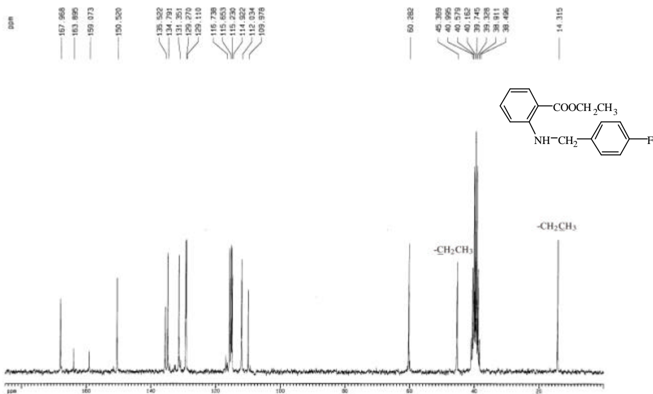
圖 51-2 ^{13}\text{C-NMR} (DMSO- d_6 , 50 MHz) spectrum of compound 51
