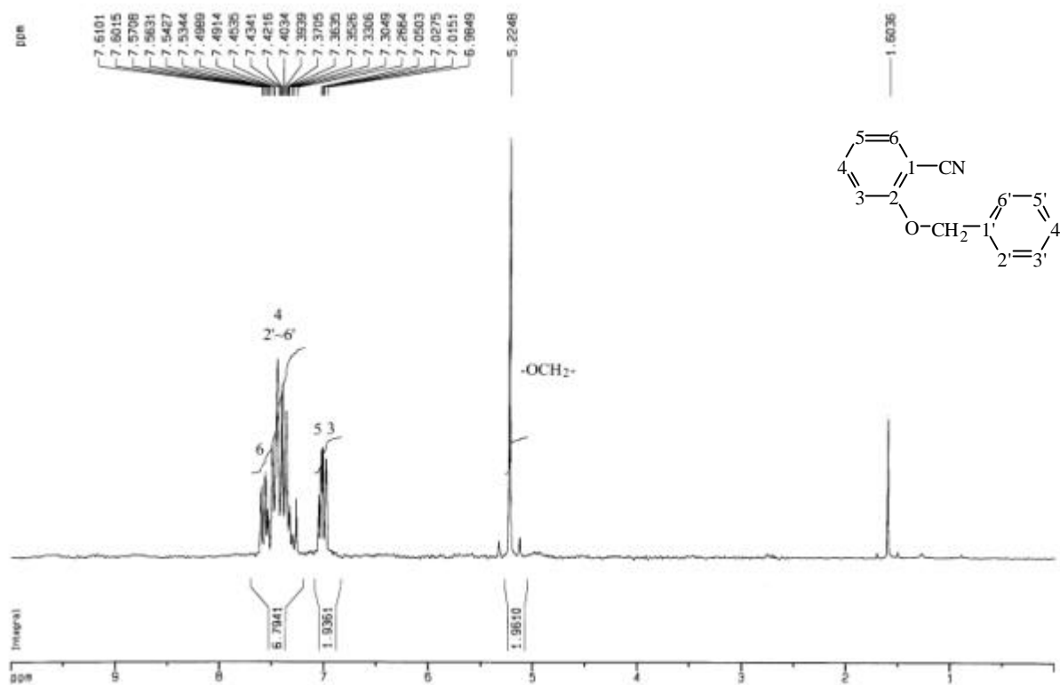
圖 17-3 ^1\text{H-NMR} (CDCl 3 , 200 MHz) spectrum of compound 17
