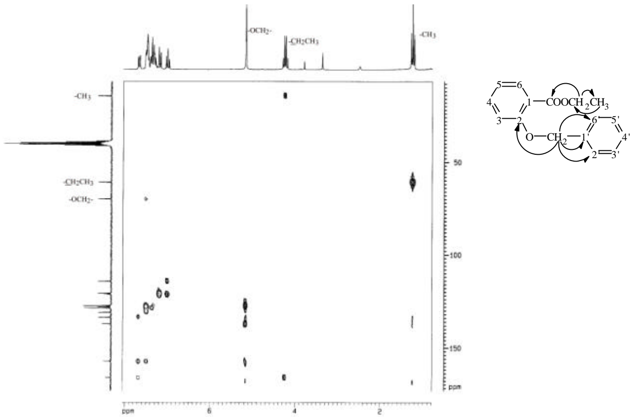
圖 38-5a HMBC (DMSO- d_6 ) spectrum of compound 38
