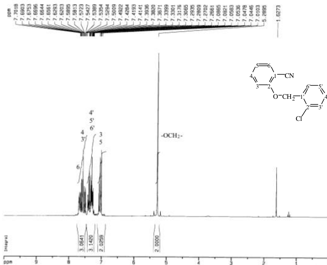
圖 18-3 1 H-NMR (CDCl 3 , 200 MHz) spectrum of compound 18
