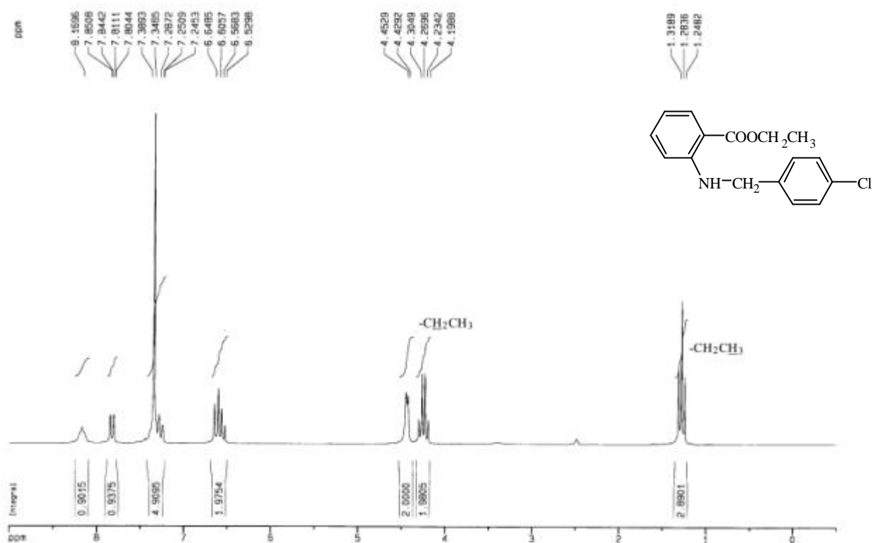
圖 48-1 ^1\text{H-NMR} ( \text{DMSO-}d_6 , 200 MHz) spectrum of compound 48
