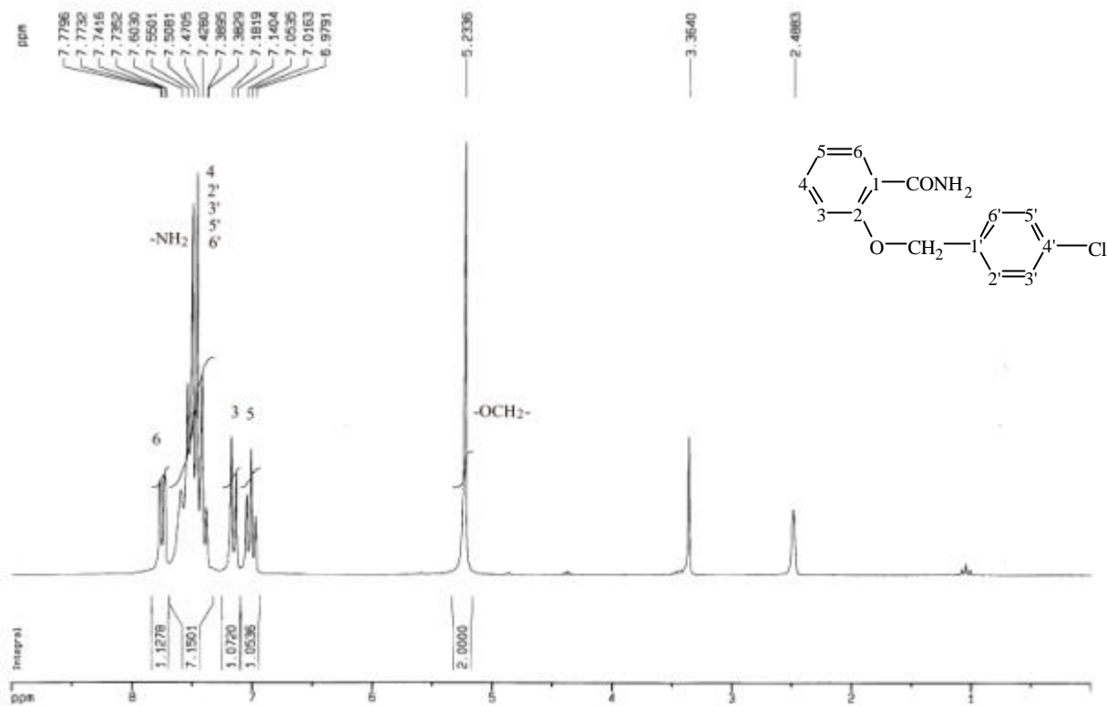
圖 44-3 ^1\text{H-NMR} ( \text{DMSO-}d_6 , 200 MHz) spectrum of compound 44
