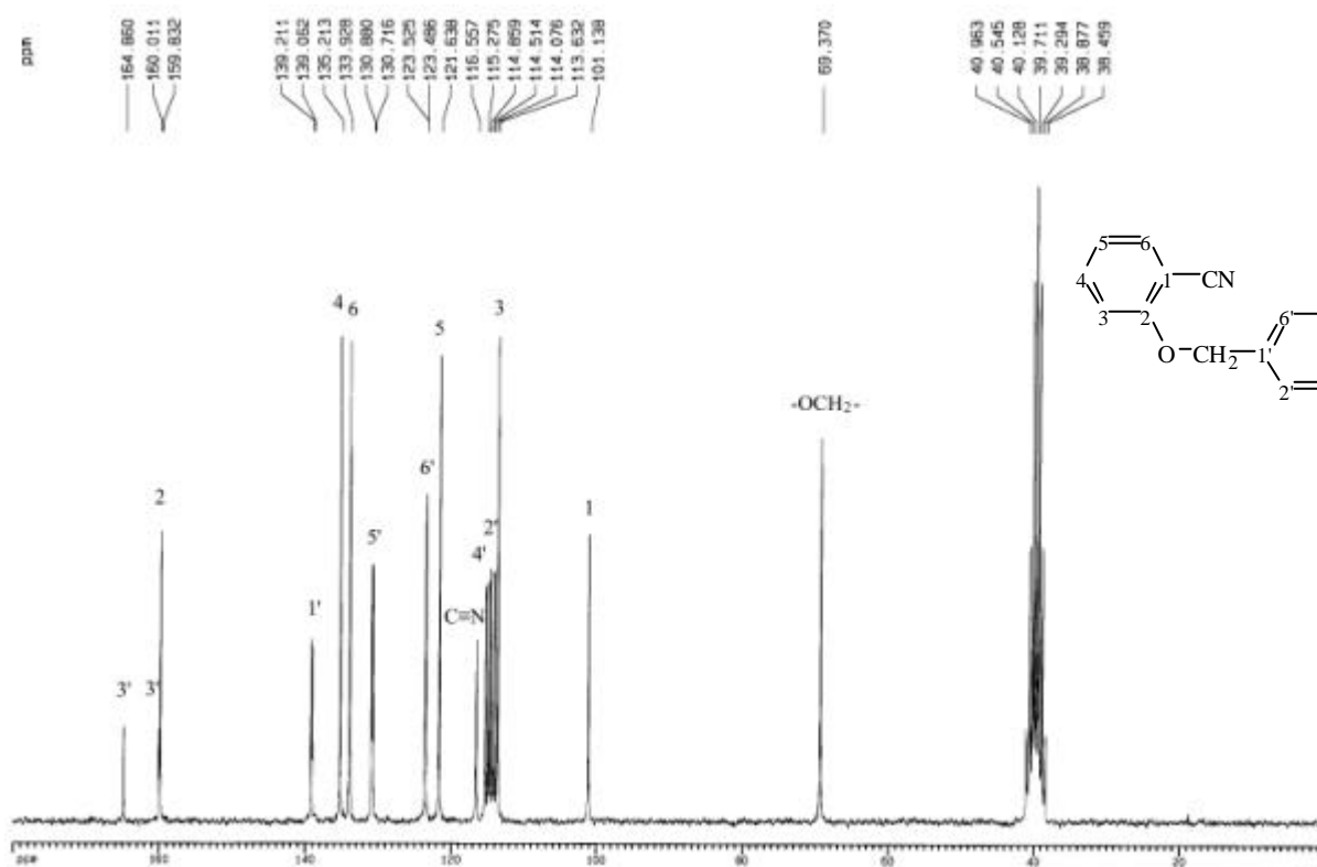
圖 22-4 13 C-NMR (DMSO- d 6 , 50 MHz) spectrum of compound 22
