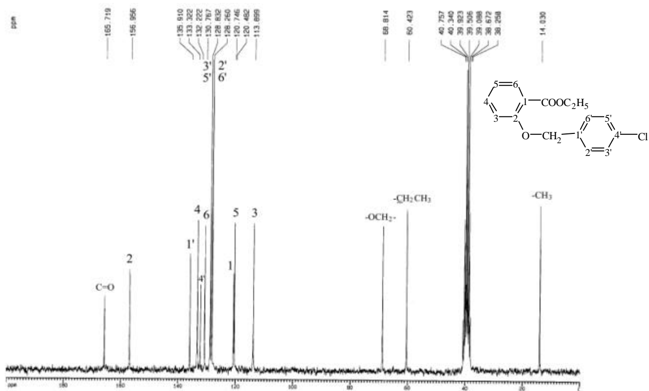
圖 41-4 ^{13}\text{C-NMR} ( \text{DMSO-}d_6 , 50 MHz) spectrum of compound 41
