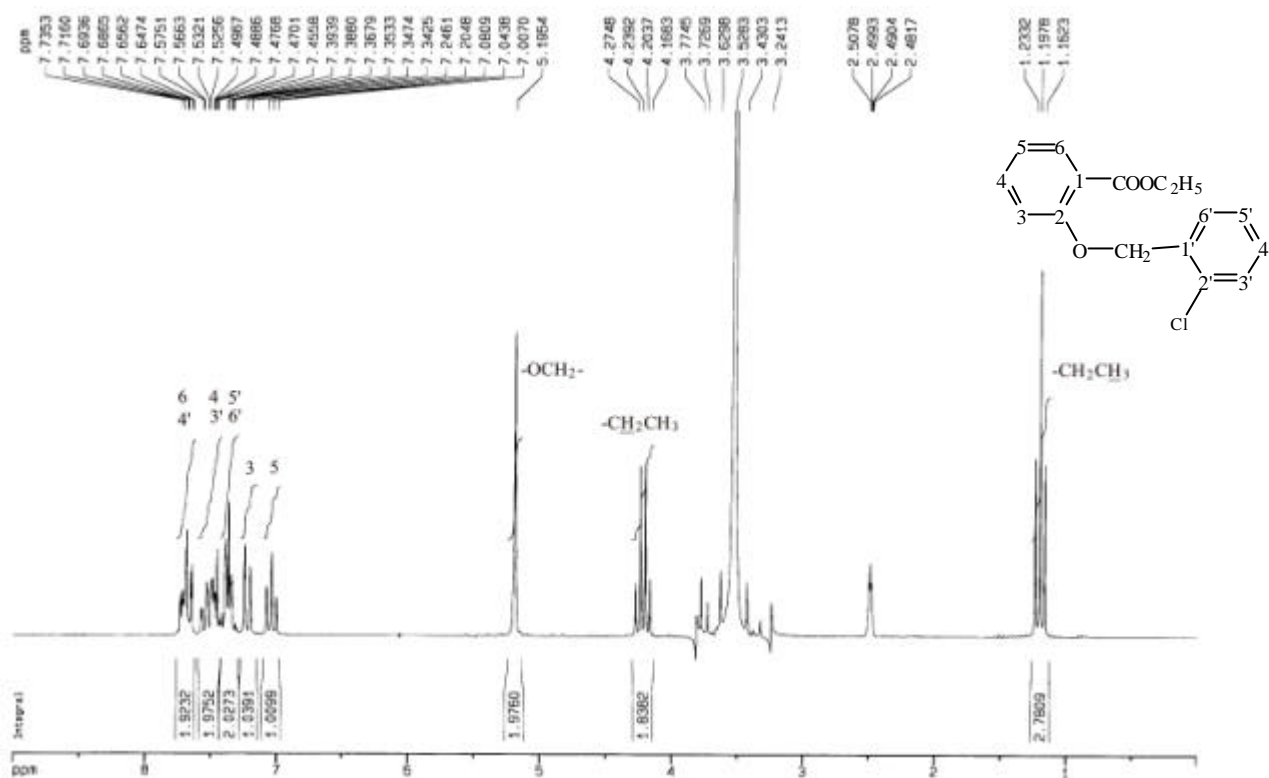
圖 39-3 1 H-NMR (DMSO- d 6 , 200 MHz) spectrum of compound 39
