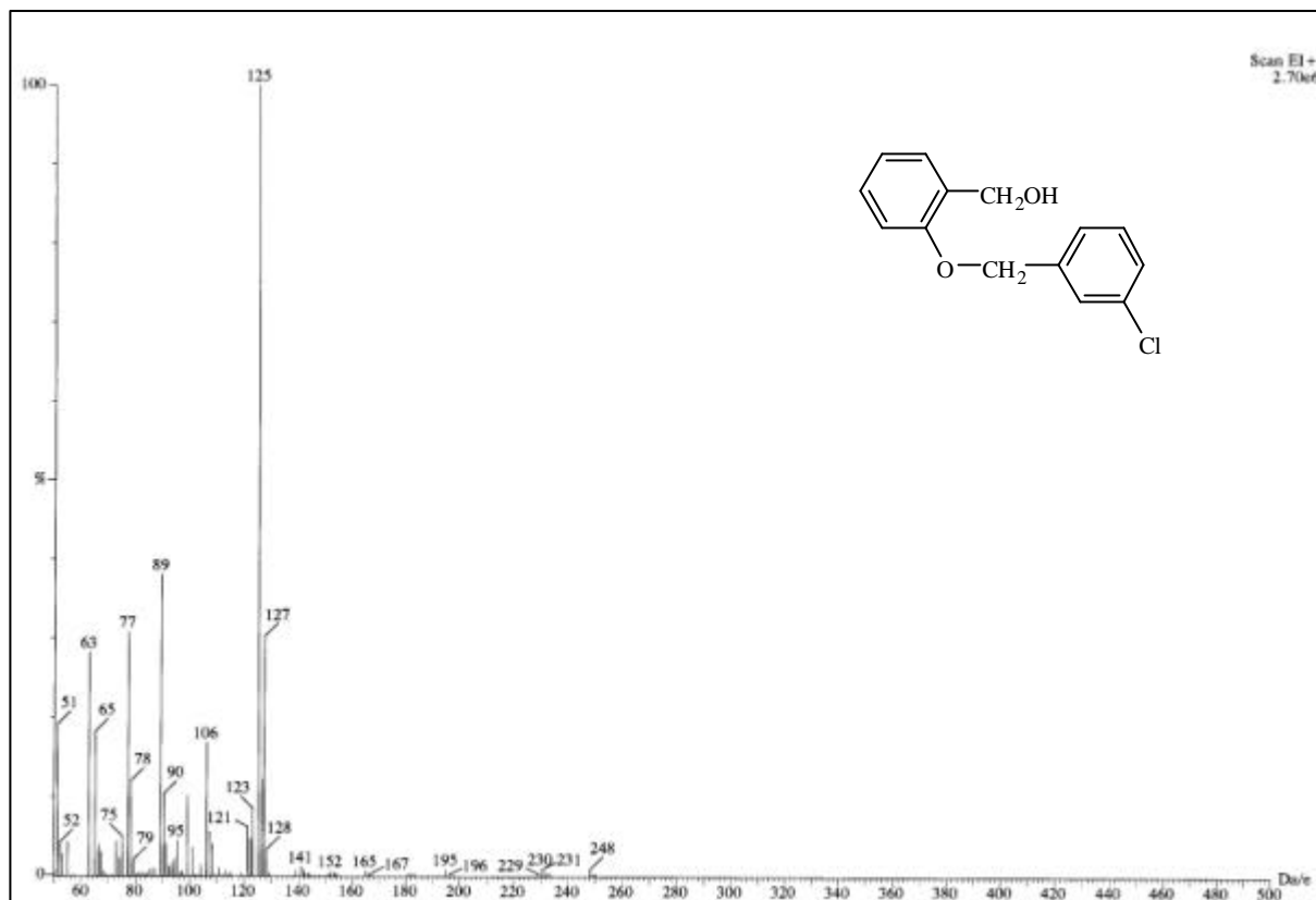
圖 32-1 MS spectrum of compound 32
