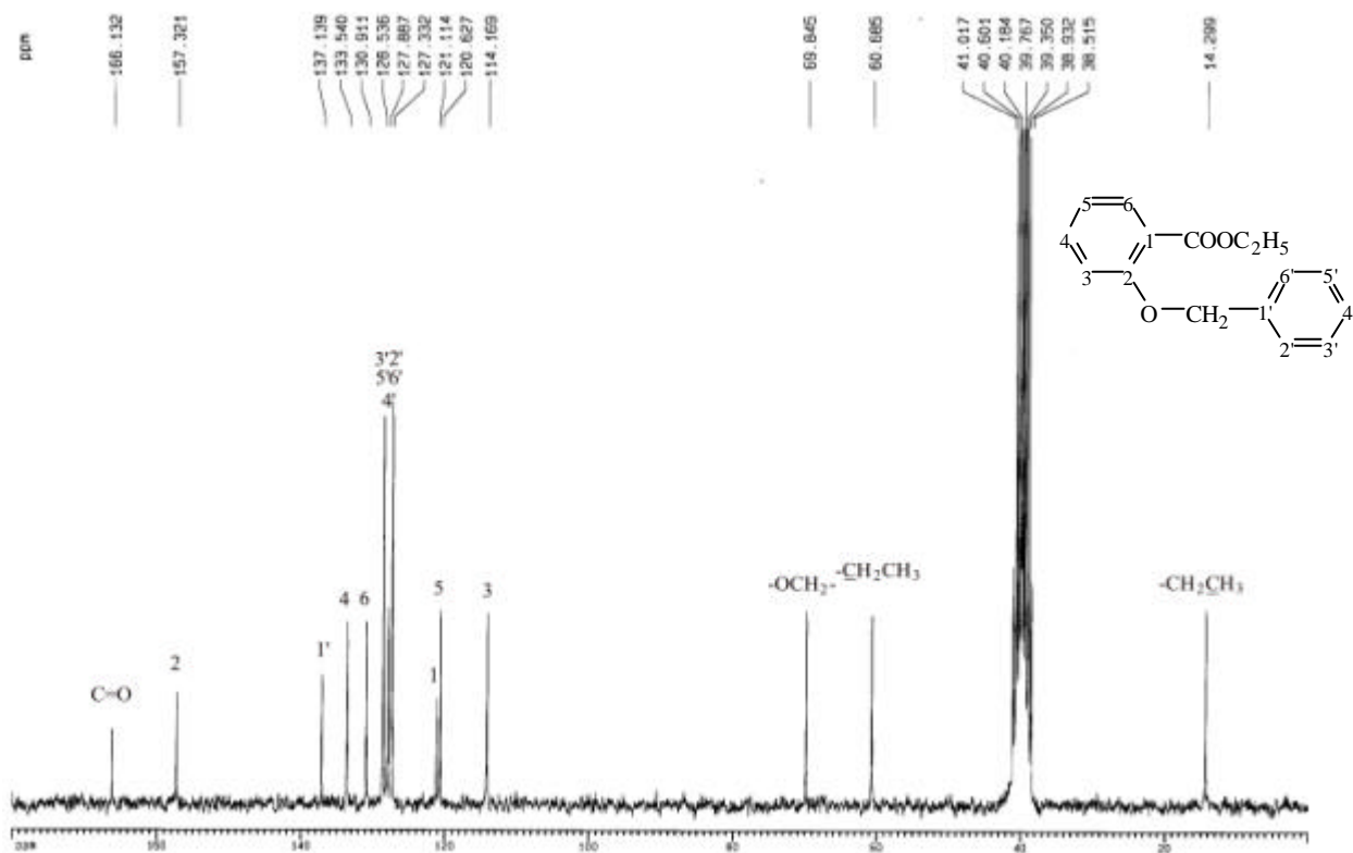
圖 38-4 13 C-NMR (DMSO- d 6 , 50 MHz) spectrum of compound 38
