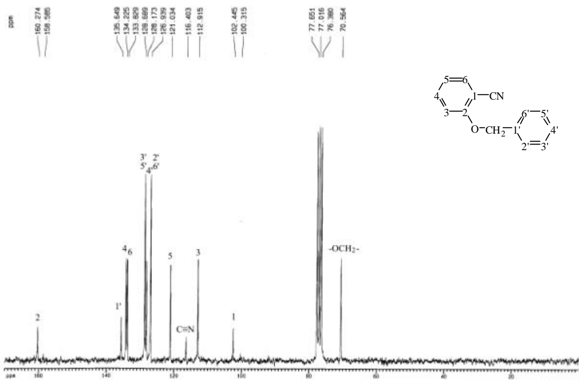
圖 17-4 ^{13}\text{C-NMR} (CDCl 3 , 50 MHz) spectrum of compound 17
