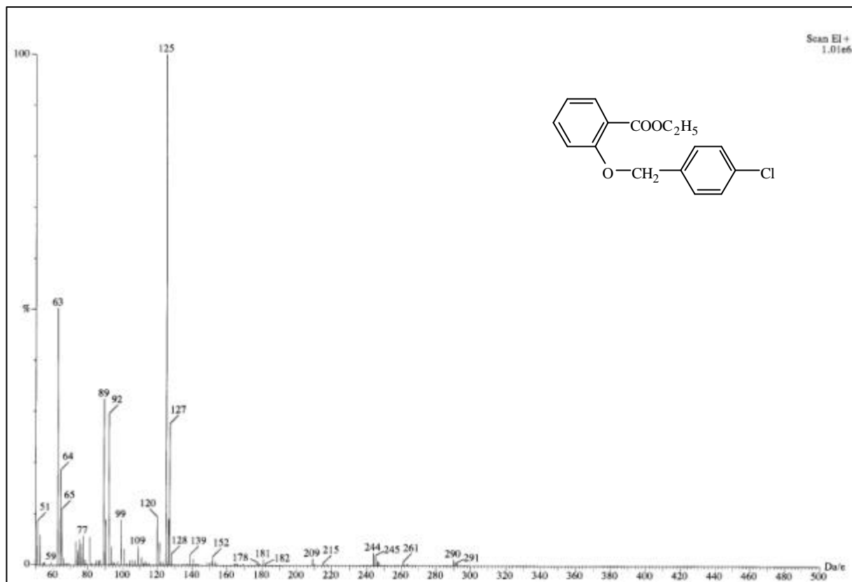
圖 41-1 MS spectrum of compound 41
