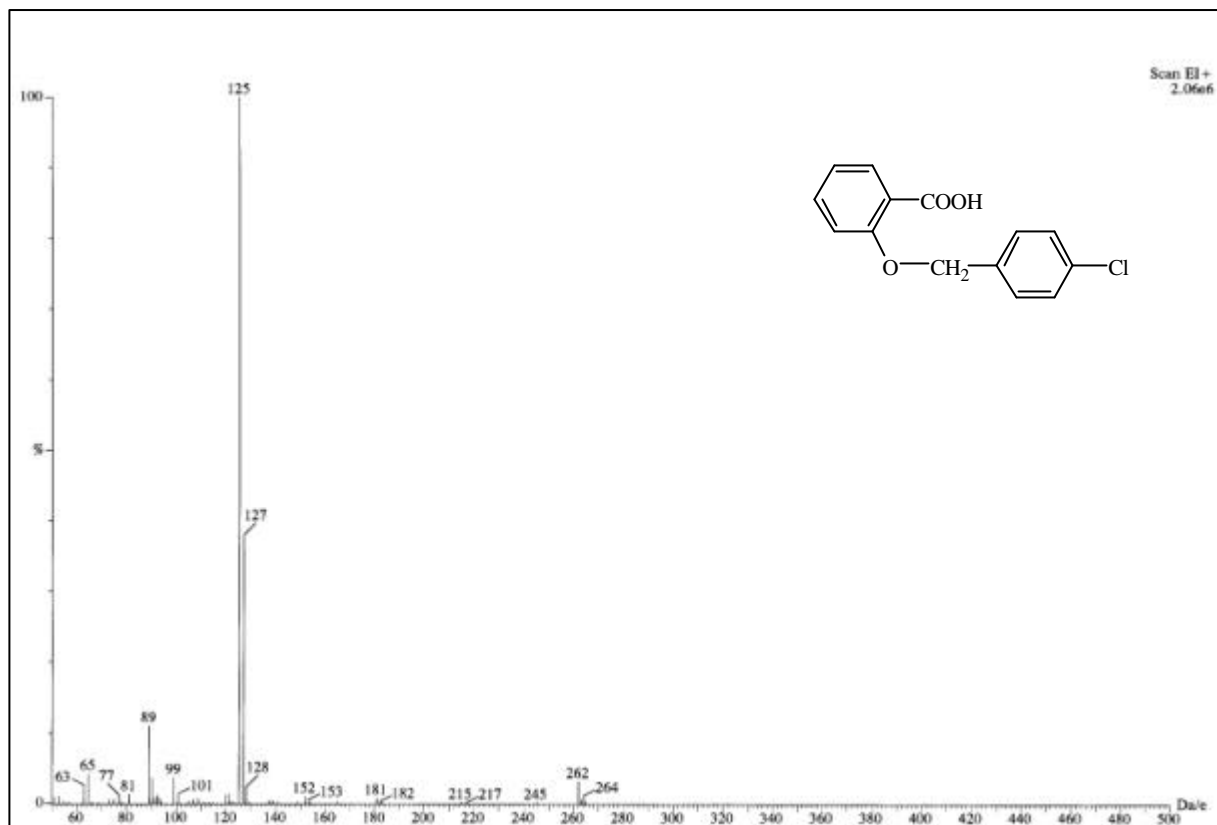
圖 59-1 MS spectrum of compound 59
