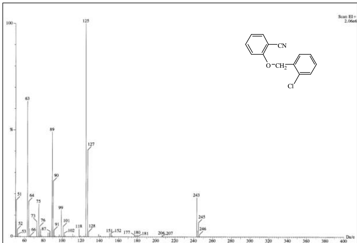
圖 18-1 MS spectrum of compound 18
