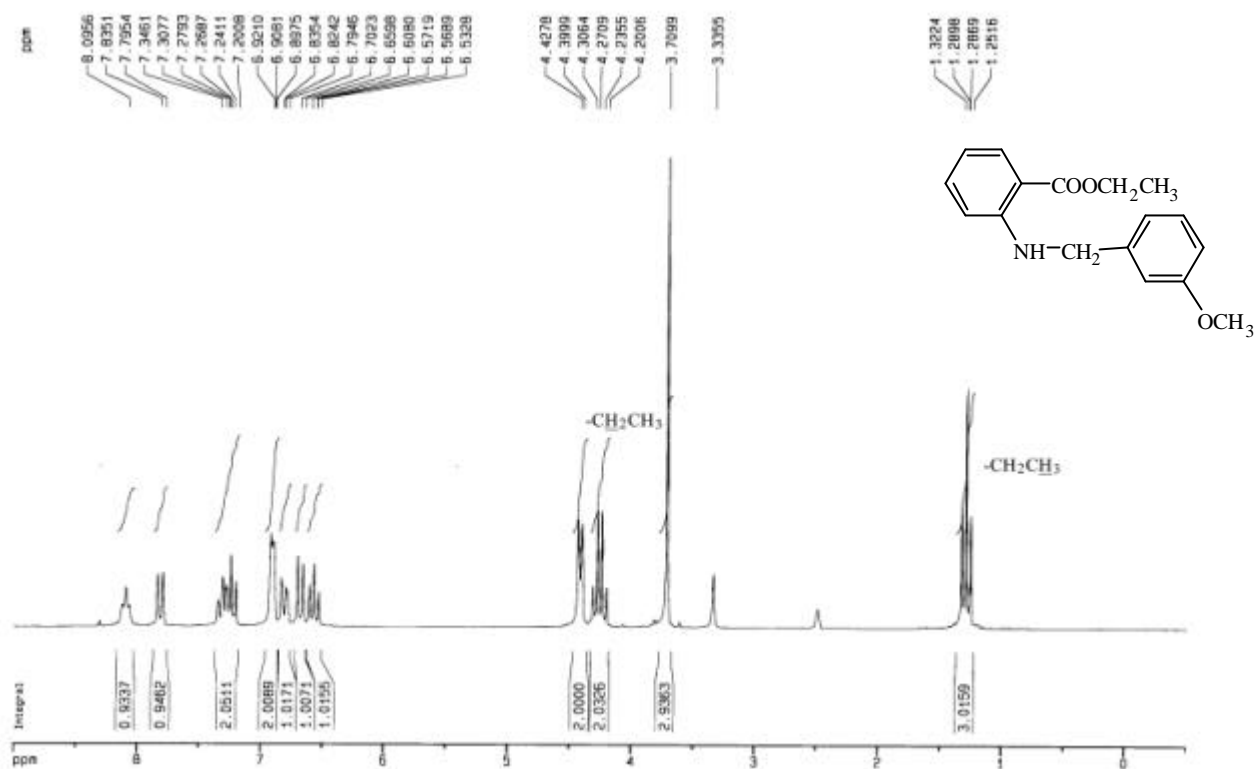
圖 52-1 1 H-NMR (DMSO- d 6 , 200 MHz) spectrum of compound 52
