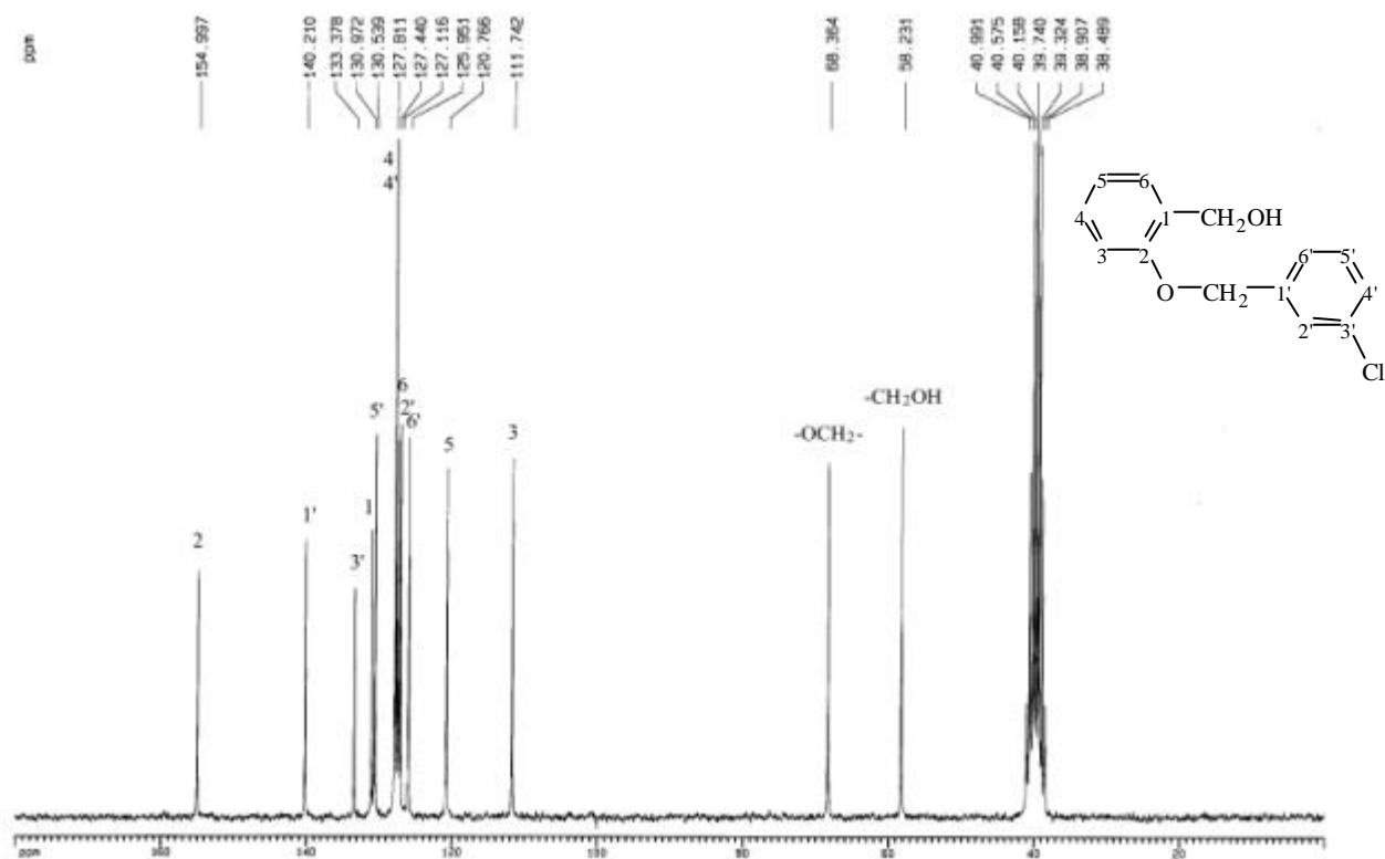
圖 32-4 13 C-NMR (DMSO- d 6 , 50 MHz) spectrum of compound 32
