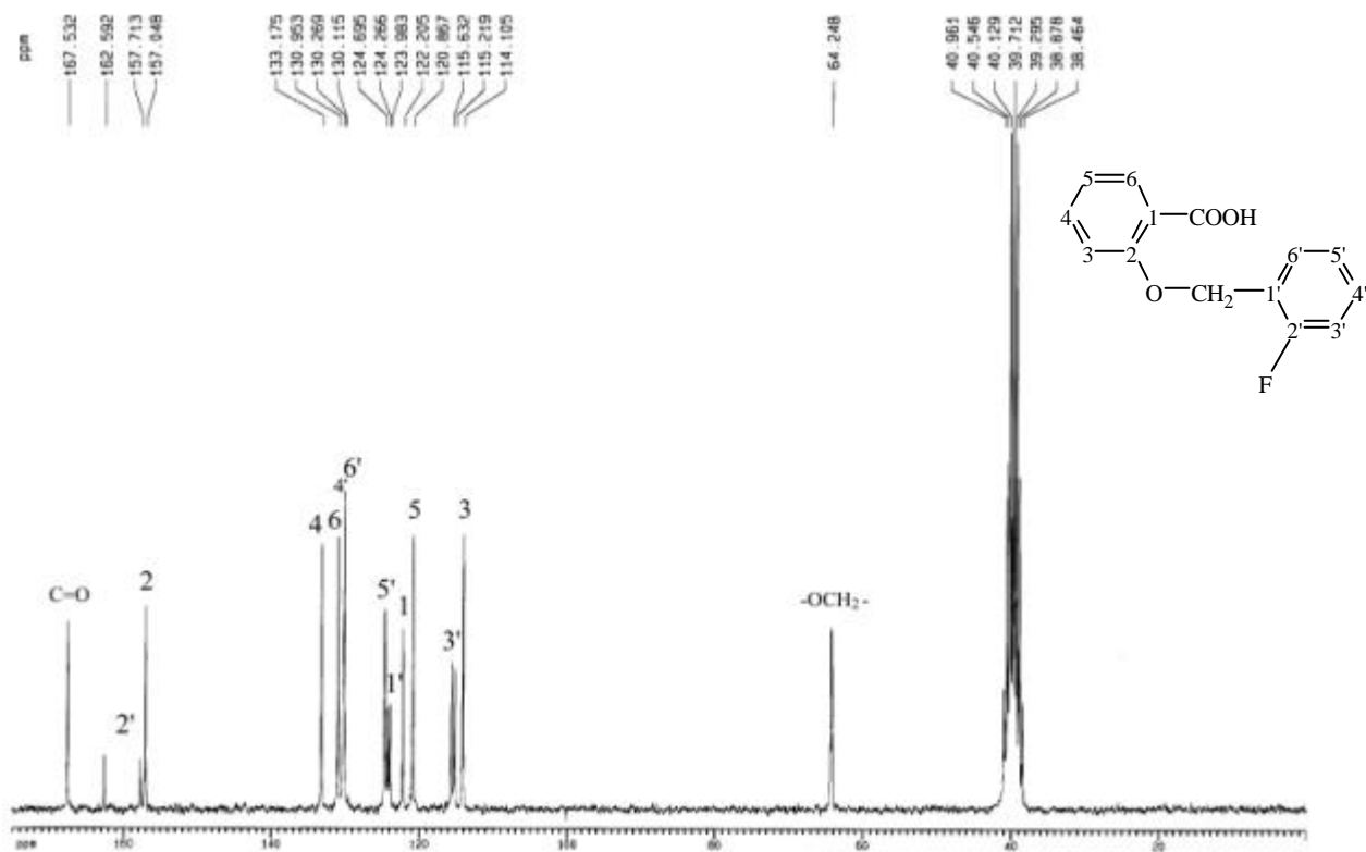
圖 60-4 13 C-NMR (DMSO- d 6 , 50 MHz) spectrum of compound 60
