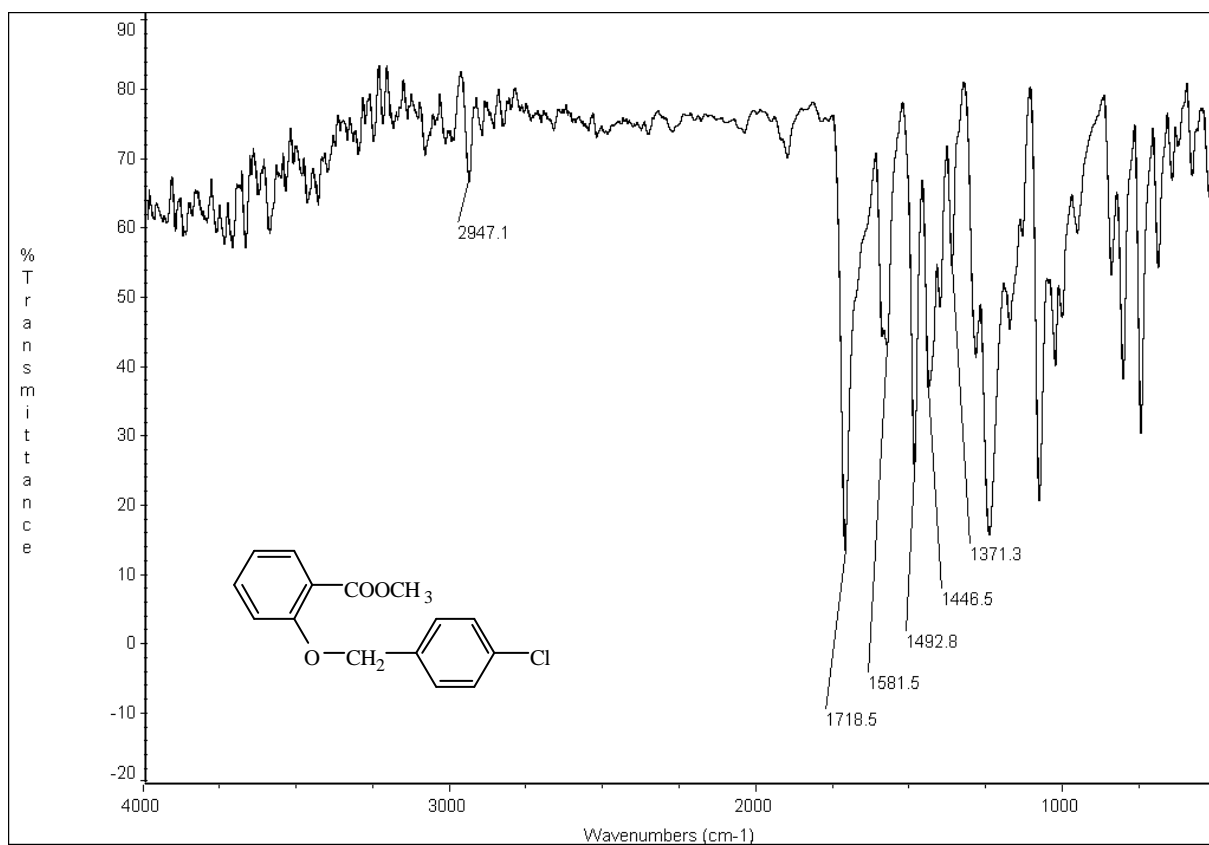
圖 37-2 IR (KBr) spectrum of compound 37
