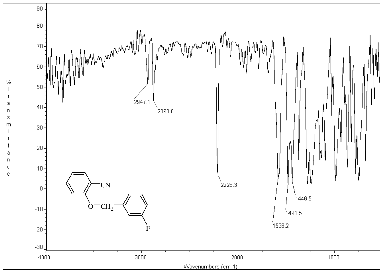
圖 22-2 IR (KBr) spectrum of compound 22
