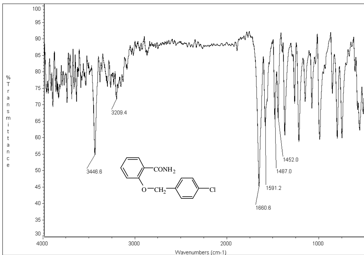
圖 44-2 IR (KBr) spectrum of compound 44
