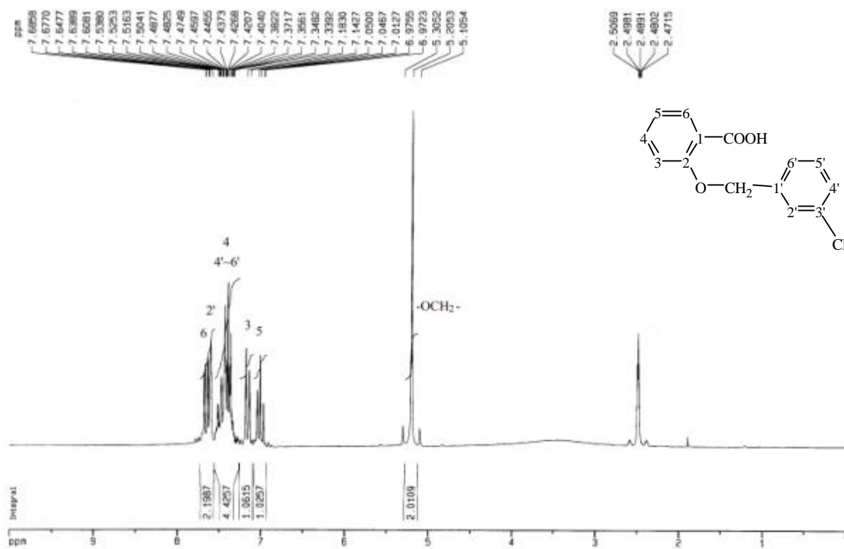
圖 58-3 ^1\text{H-NMR} ( \text{DMSO-}d_6 , 200 MHz) spectrum of compound 58
