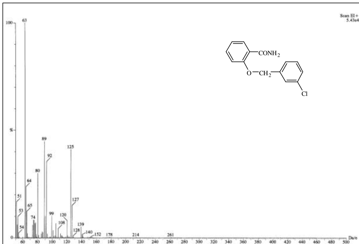
圖 43-1 MS spectrum of compound 43
