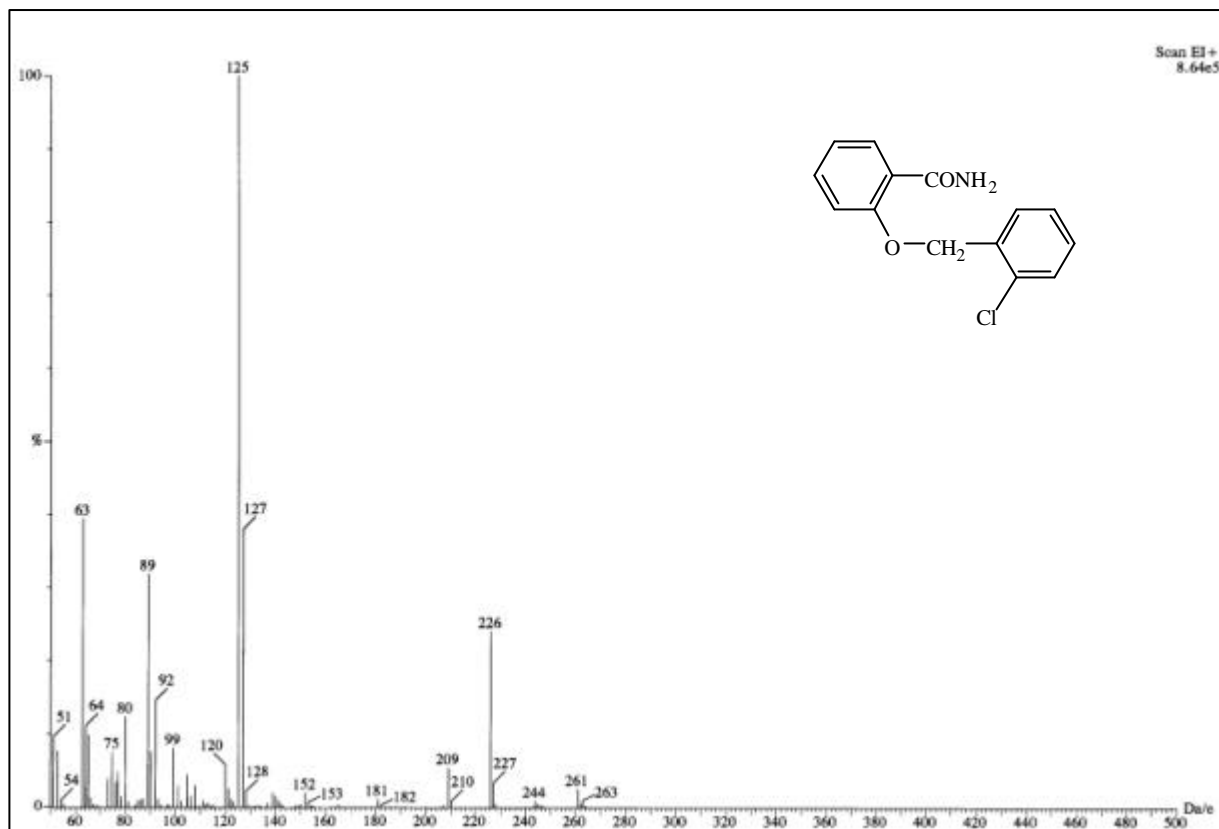
圖 42-1 MS spectrum of compound 42
