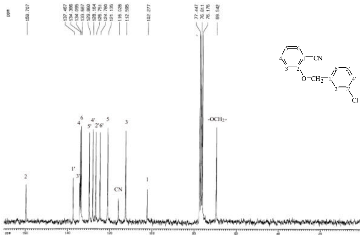
圖 19-4 ^{13}\text{C-NMR} ( \text{CDCl}_3 , 50 MHz) spectrum of compound 19
