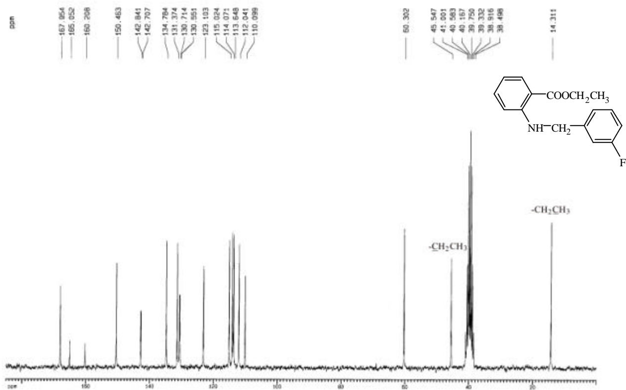
圖 50-2 13 C-NMR (DMSO- d 6 , 50 MHz) spectrum of compound 50
