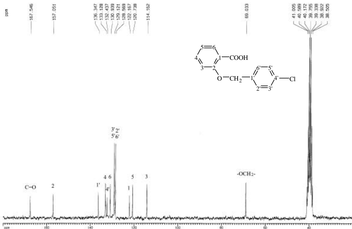
圖 59-4 ^{13}\text{C-NMR} ( \text{DMSO-}d_6 , 50 MHz) spectrum of compound 59
