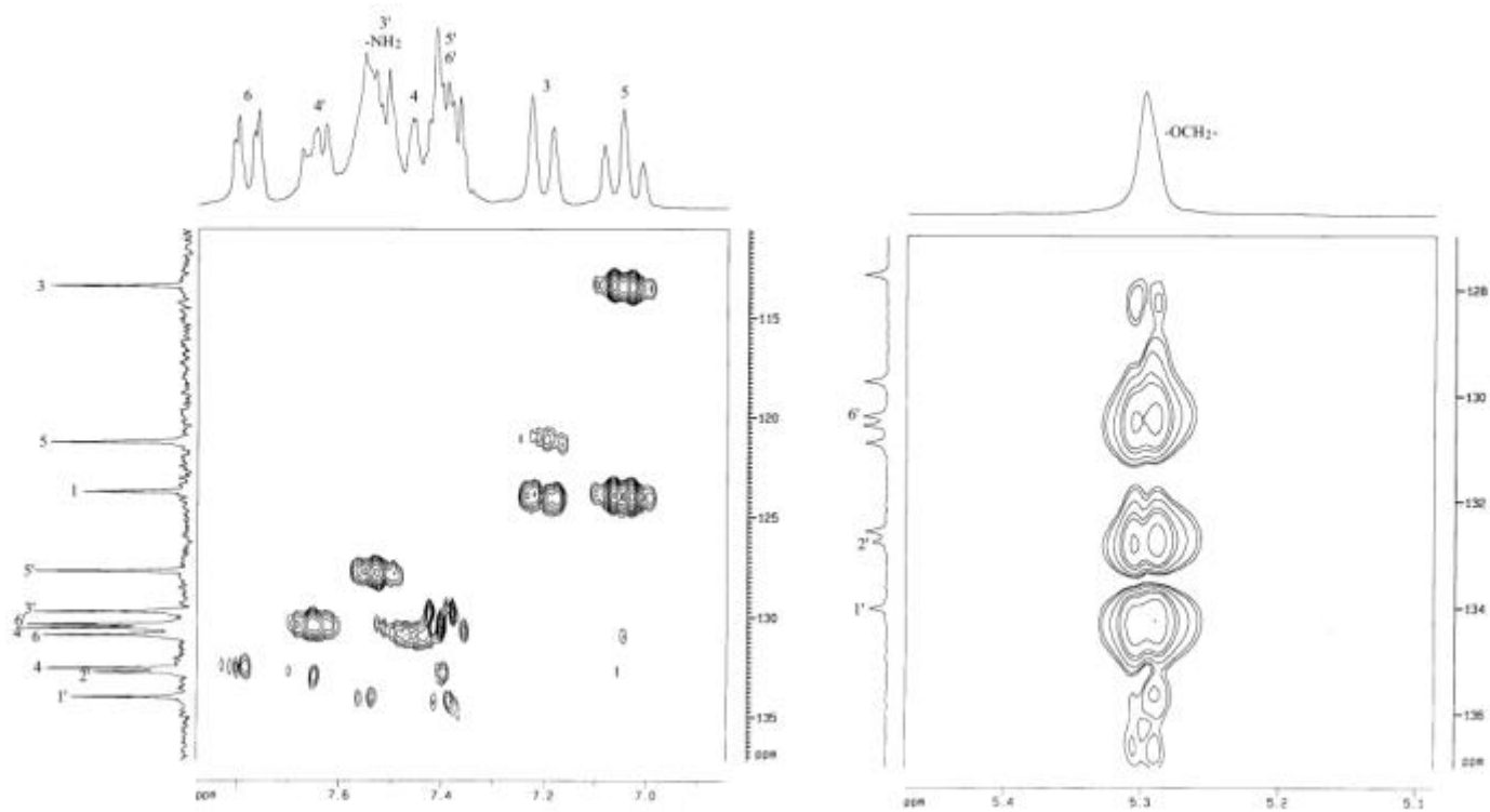
圖 42-5b HMBC (DMSO- d_6 ) spectrum of compound 42
