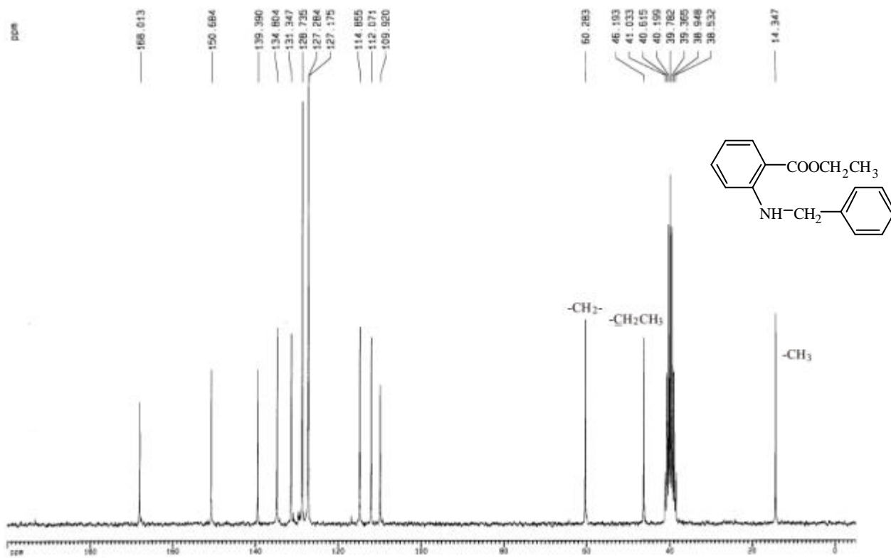
圖 45-2 ^{13}\text{C-NMR} ( \text{DMSO-}d_6 , 50 MHz) spectrum of compound 45
