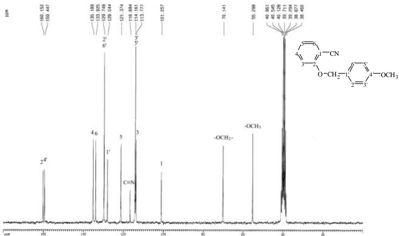
圖 25-4 ^{13}\text{C-NMR} ( \text{DMSO-}d_6 , 50 MHz) spectrum of compound 25
