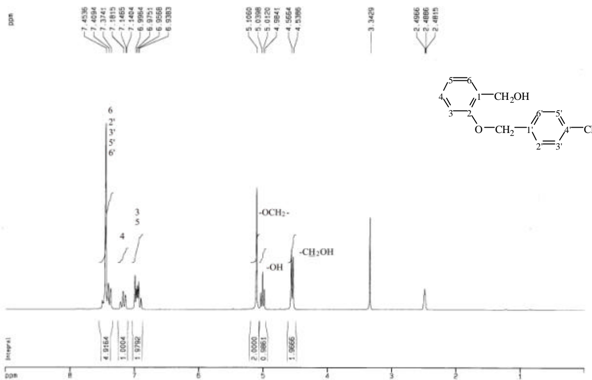
圖 33-3 1 H-NMR (DMSO- d 6 , 200 MHz) spectrum of compound 33
