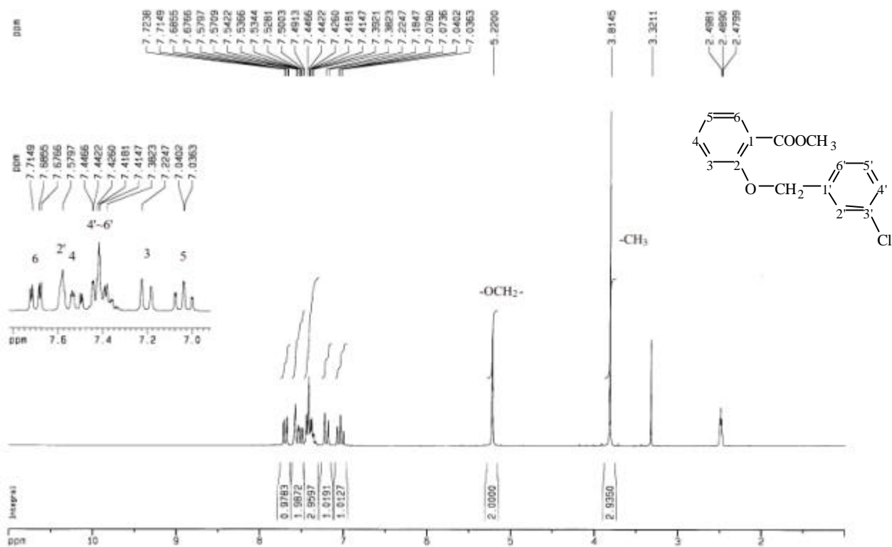
圖 36-3 1 H-NMR (DMSO- d 6 , 200 MHz) spectrum of compound 36
