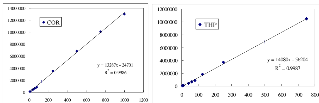
Figure 11. Pure compound of corydaline and tetrahydropalmatine determined by HPLC.
