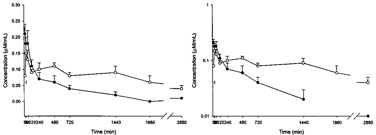
Fig. 3 Mean ( \pm S.E.) serum concentration-time profiles of methotrexate (MTX) after oral administration of MTX alone (●) and coadministration with Scutellariae Radix (o) in rats.
